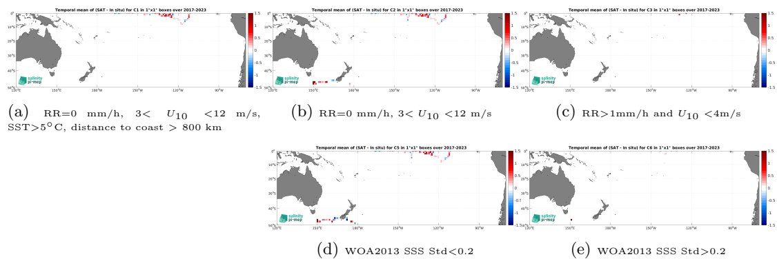
Figure 14: Temporal mean gridded over spatial boxes of size 1^\circ \times 1^\circ of \Delta SSS (SMAP SSS L2 v6 - 40 km (RSS) - Saldrone) for 5 different subdatasets corresponding to:RR=0 mm/h, 3 < U_{10} < 12 m/s, SST >5^\circ C, distance to coast > 800 km (a), RR=0 mm/h, 3 < U_{10} < 12 m/s (b), RR >1 mm/h and U_{10} < 4 m/s (c), WOA2013 SSS Std <0.2 (d), WOA2013 SSS Std >0.2 (e).
