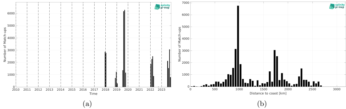
Figure 2: Number of match-ups between Saildrone and SMAP SSS L2 v6 - 40 km (RSS) SSS as a function of time (a) and as function of the distance to coast (b) over the South Pacific Ocean Pi-MEP region and for the full satellite product period.
