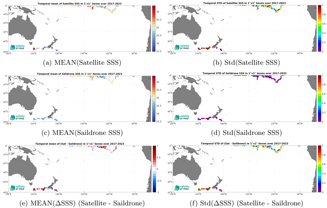
Figure 7: Temporal mean (left) and Std (right) of SSS from SMAP SSS L2 v6 - 40 km (RSS) (top), Saildrone (middle), and of \Delta SSS (Satellite - Saildrone). Only match-up pairs are used to generate these maps.
