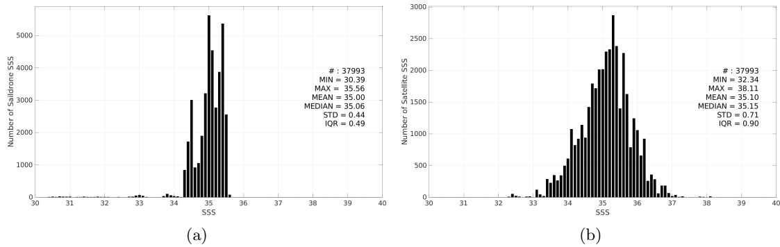
Figure 3: Histograms of SSS from Saildrone (a) and SMAP SSS L2 v6 - 40 km (RSS) (b) considering all match-up pairs per bins of 0.1 over the South Pacific Ocean Pi-MEP region and for the full satellite product period.
