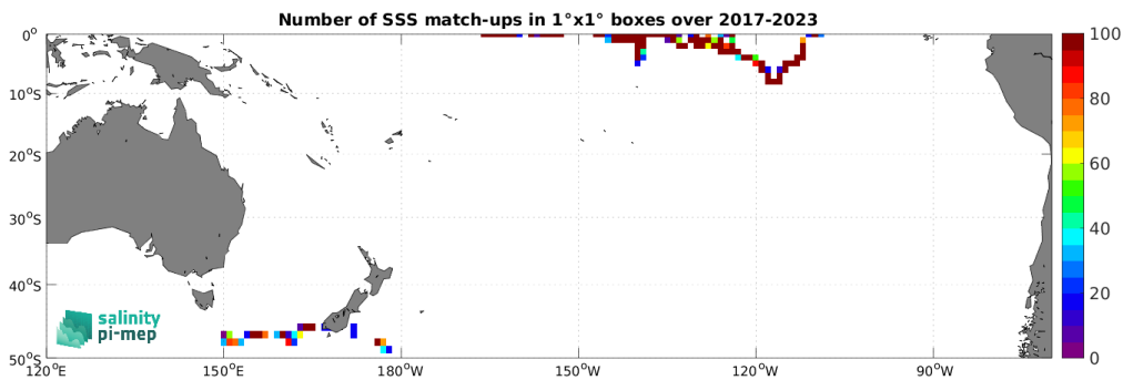
Figure 5: Number of SSS match-ups between Saildrone SSS and the SMAP SSS L2 v6 - 40 km (RSS) SSS product for the South Pacific Ocean Pi-MEP region over 1^\circ \times 1^\circ boxes and for the full satellite product period.
