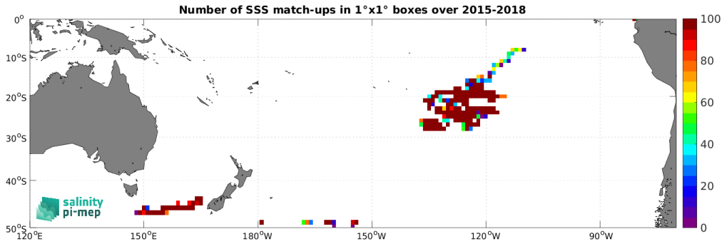
Figure 4: Number of SSS match-ups between Surface drifters SSS and the SMAP SSS L2 v6 - 40 km (RSS) SSS product for the South Pacific Ocean Pi-MEP region over 1^\circ \times 1^\circ boxes and for the full satellite product period.
