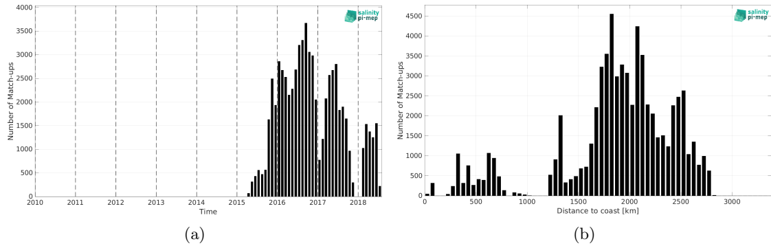
Figure 2: Number of match-ups between Surface drifters and SMAP SSS L2 v6 - 40 km (RSS) SSS as a function of time (a) and as function of the distance to coast (b) over the South Pacific Ocean Pi-MEP region and for the full satellite product period.
