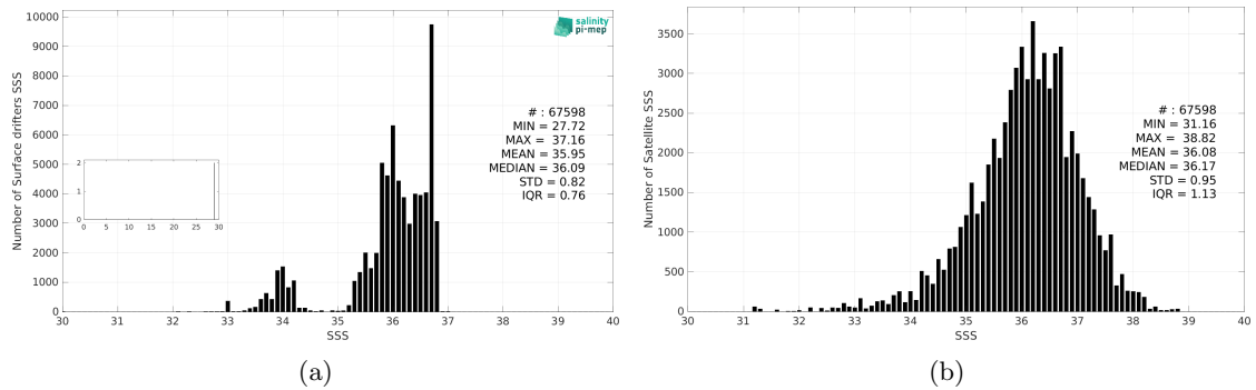
Figure 3: Histograms of SSS from Surface drifters (a) and SMAP SSS L2 v6 - 40 km (RSS) (b) considering all match-up pairs per bins of 0.1 over the South Pacific Ocean Pi-MEP region and for the full satellite product period.
