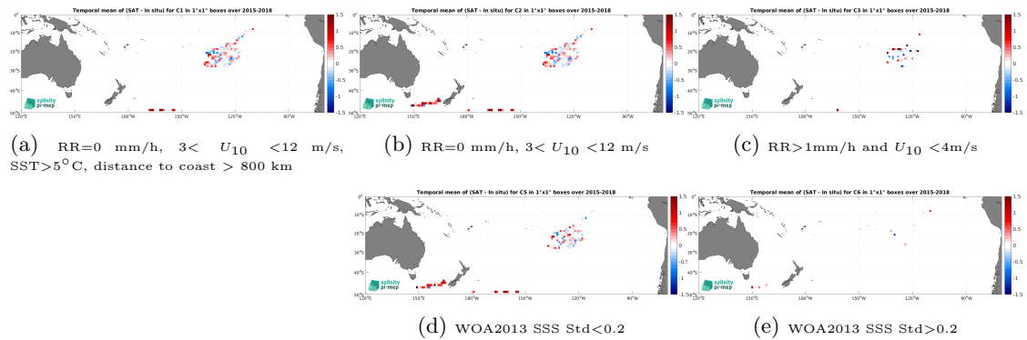
Figure 13: Temporal mean gridded over spatial boxes of size 1^\circ \times 1^\circ of \Delta SSS (SMAP SSS L2 v6 - 40 km (RSS) - Surface drifters) for 5 different subdatasets corresponding to: RR=0 mm/h, 3 < U_{10} < 12 m/s, SST > 5^\circ C , distance to coast > 800 km (a), RR=0 mm/h, 3 < U_{10} < 12 m/s (b), RR > 1 mm/h and U_{10} < 4 m/s (c), WOA2013 SSS Std < 0.2 (d), WOA2013 SSS Std > 0.2 (e).
