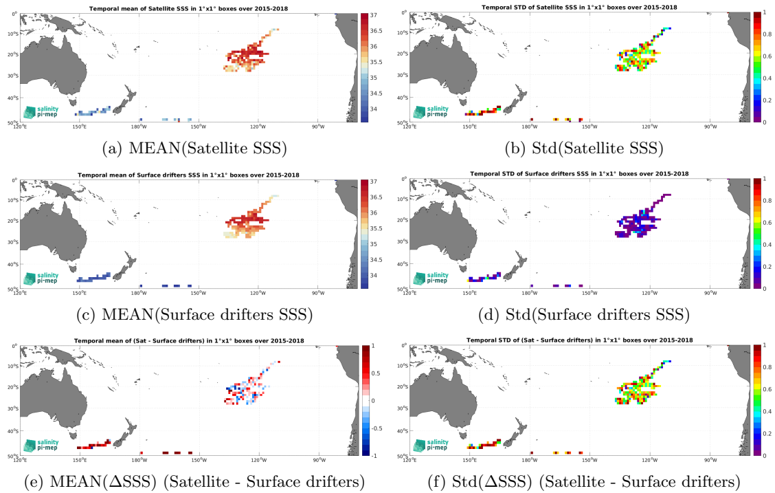
Figure 6: Temporal mean (left) and Std (right) of SSS from SMAP SSS L2 v6 - 40 km (RSS) (top), Surface drifters (middle), and of \Delta SSS (Satellite - Surface drifters). Only match-up pairs are used to generate these maps.
