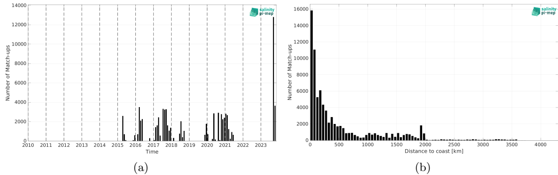
Figure 1: Number of match-ups between TSG (SAMOS) and SMAP SSS L2 v5 (RSS) SSS as a function of time (a) and as function of the distance to coast (b) over the South Pacific Ocean Pi-MEP region and for the full satellite product period.
