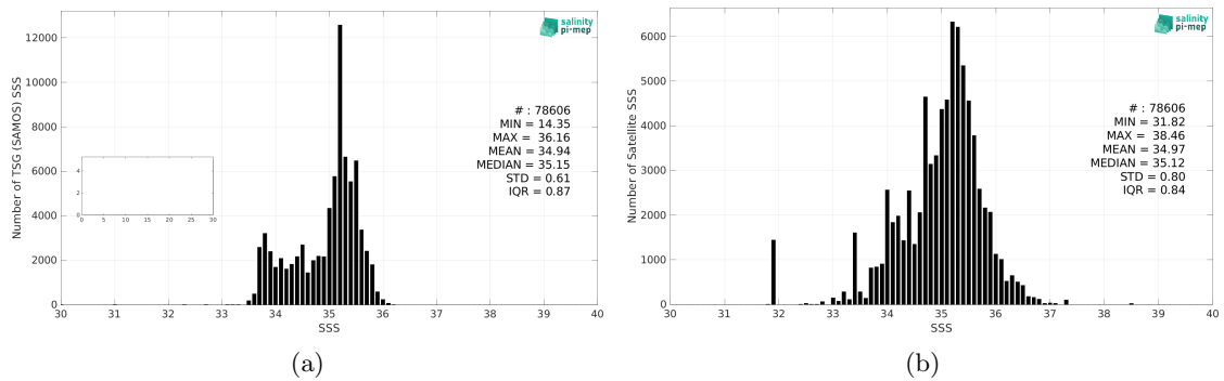
Figure 2: Histograms of SSS from TSG (SAMOS) (a) and SMAP SSS L2 v5 (RSS) (b) considering all match-up pairs per bins of 0.1 over the South Pacific Ocean Pi-MEP region and for the full satellite product period.
