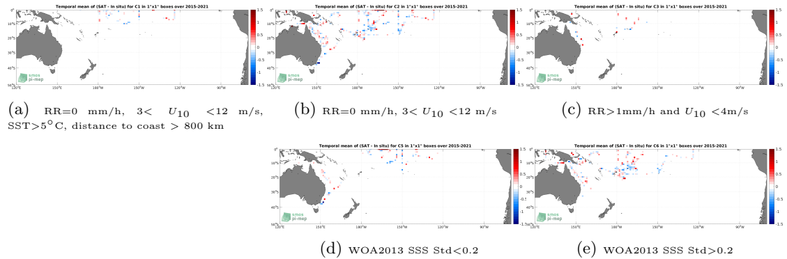
Figure 12: Temporal mean gridded over spatial boxes of size 1^\circ \times 1^\circ of \Delta SSS (SMAP SSS L2 v5 (RSS) - TSG (SAMOS)) for 5 different subdatasets corresponding to:RR=0 mm/h, 3 < U_{10} < 12 m/s, SST >5^\circ C, distance to coast > 800 km (a), RR=0 mm/h, 3 < U_{10} < 12 m/s (b), RR >1 mm/h and U_{10} < 4 m/s (c), WOA2013 SSS Std <0.2 (d), WOA2013 SSS Std >0.2 (e).
