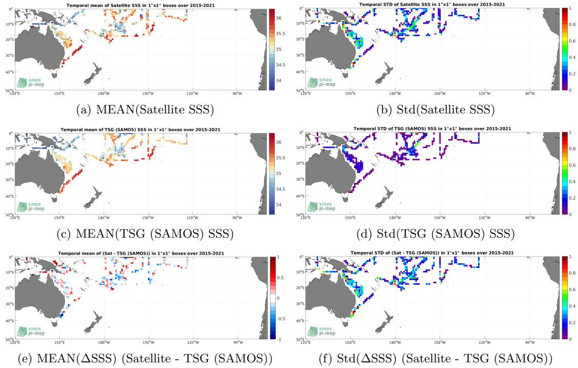
Figure 6: Temporal mean (left) and Std (right) of SSS from SMAP SSS L2 v5 (RSS) (top), TSG (SAMOS) (middle), and of \Delta SSS (Satellite - TSG (SAMOS)). Only match-up pairs are used to generate these maps.
