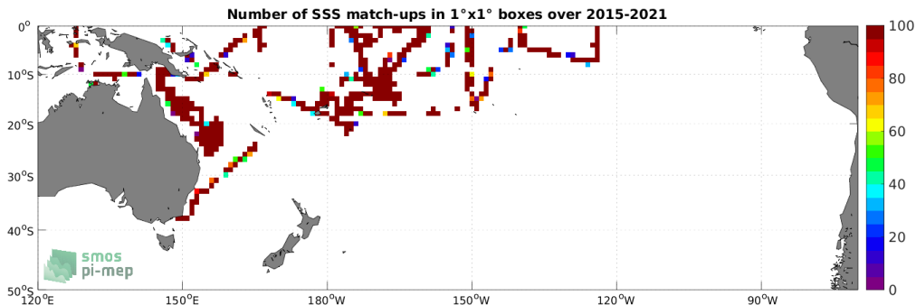
Figure 4: Number of SSS match-ups between TSG (SAMOS) SSS and the SMAP SSS L2 v5 (RSS) SSS product for the South Pacific Ocean Pi-MEP region over 1^\circ \times 1^\circ boxes and for the full satellite product period.
