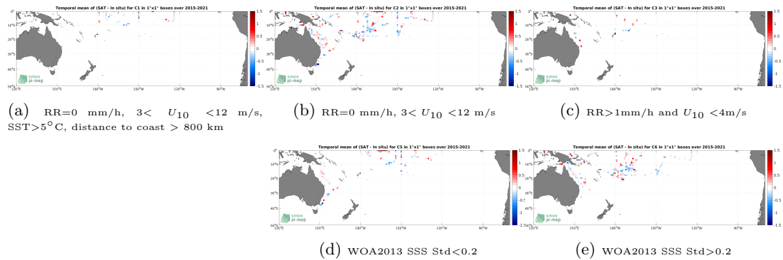
Figure 12: Temporal mean gridded over spatial boxes of size 1^\circ \times 1^\circ of \Delta\text{SSS} (SMAP SSS L2 v5 (RSS) - TSG (SAMOS)) for 5 different subdatasets corresponding to:RR=0 mm/h, 3 < U_{10} < 12 m/s, SST >5^\circ\text{C} , distance to coast > 800 km (a), RR=0 mm/h, 3 < U_{10} < 12 m/s (b), RR >1 mm/h and U_{10} < 4 m/s (c), WOA2013 SSS Std <0.2 (d), WOA2013 SSS Std >0.2 (e).
