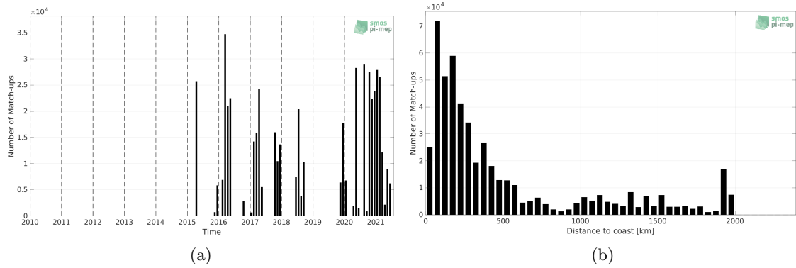
Figure 1: Number of match-ups between TSG (SAMOS) and SMAP SSS L2 v5 (RSS) SSS as a function of time (a) and as function of the distance to coast (b) over the South Pacific Ocean Pi-MEP region and for the full satellite product period.
