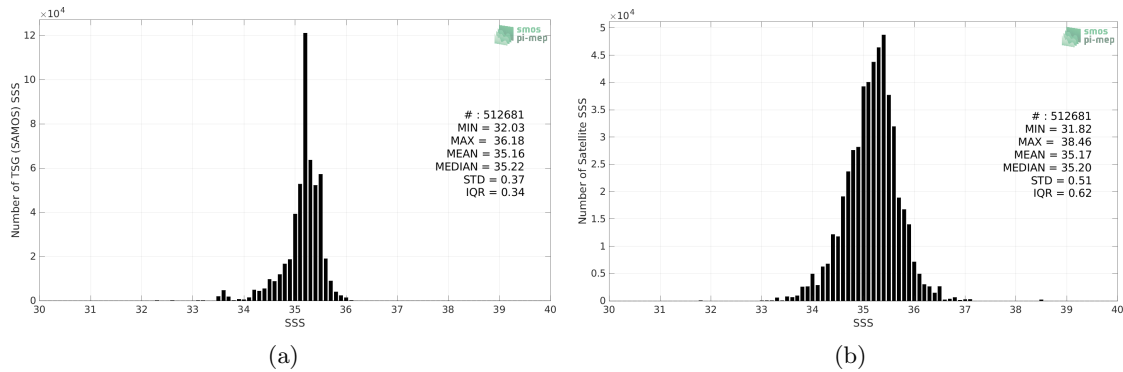
Figure 2: Histograms of SSS from TSG (SAMOS) (a) and SMAP SSS L2 v5 (RSS) (b) considering all match-up pairs per bins of 0.1 over the South Pacific Ocean Pi-MEP region and for the full satellite product period.
