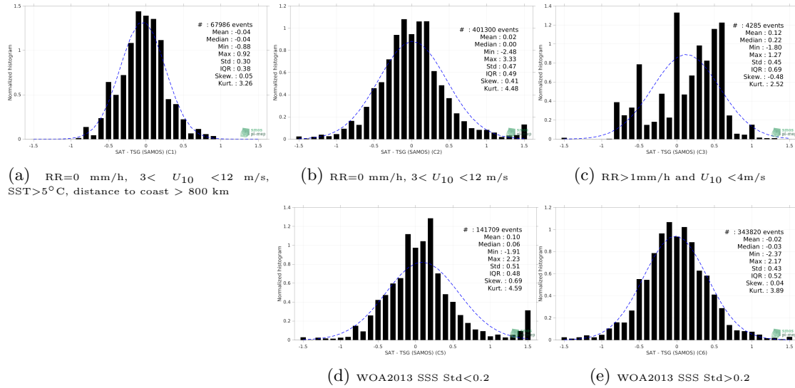
Figure 13: Normalized histogram of \Delta\text{SSS} (SMAP SSS L2 v5 (RSS) - TSG (SAMOS)) for 5 different subdatasets corresponding to: RR=0 mm/h, 3 < U_{10} < 12 m/s, SST>5°C, distance to coast > 800 km (a), RR=0 mm/h, 3 < U_{10} < 12 m/s (b), RR>1mm/h and U_{10} < 4 m/s (c), WOA2013 SSS Std<0.2 (d), WOA2013 SSS Std>0.2 (e).
