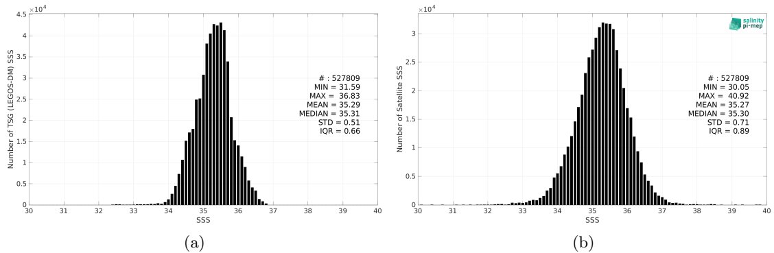
Figure 2: Histograms of SSS from TSG (LEGOS-DM) (a) and SMAP SSS L2 v5 (RSS) (b) considering all match-up pairs per bins of 0.1 over the South Pacific Ocean Pi-MEP region and for the full satellite product period.
