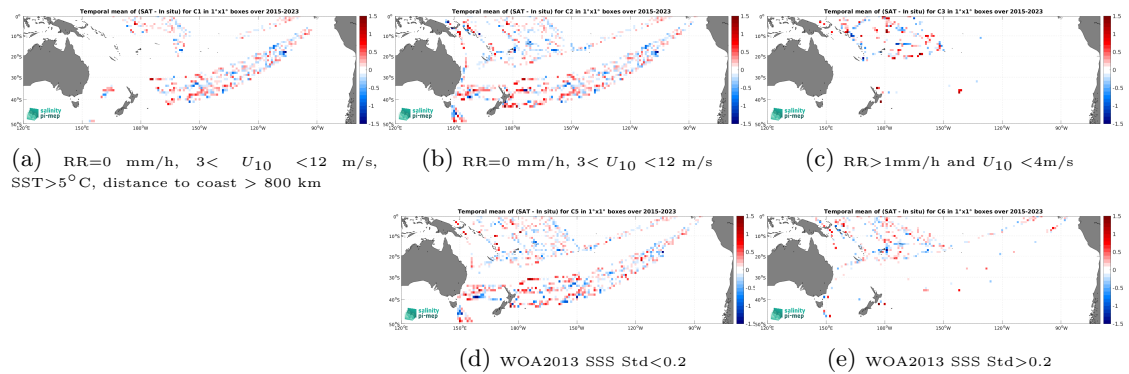
Figure 12: Temporal mean gridded over spatial boxes of size 1^\circ \times 1^\circ of \Delta SSS (SMAP SSS L2 v5 (RSS) - TSG (LEGOS-DM)) for 5 different subdatasets corresponding to:RR=0 mm/h, 3 < U_{10} < 12 m/s, SST >5^\circ C, distance to coast > 800 km (a), RR=0 mm/h, 3 < U_{10} < 12 m/s (b), RR >1 mm/h and U_{10} < 4 m/s (c), WOA2013 SSS Std <0.2 (d), WOA2013 SSS Std >0.2 (e).
