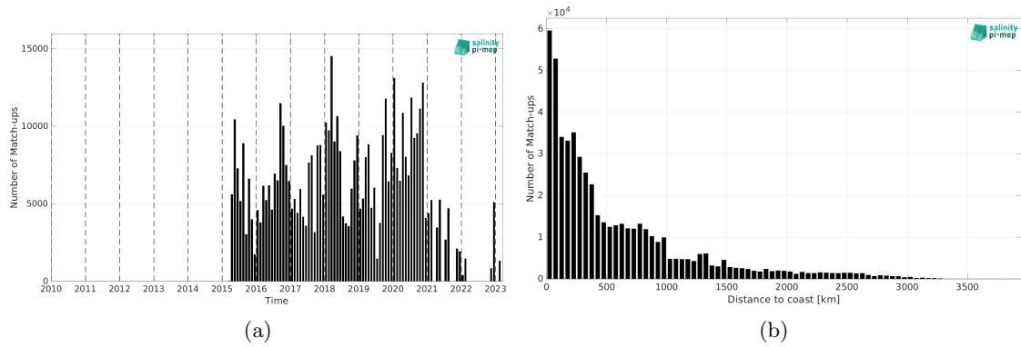
Figure 1: Number of match-ups between TSG (LEGOS-DM) and SMAP SSS L2 v5 (RSS) SSS as a function of time (a) and as function of the distance to coast (b) over the South Pacific Ocean Pi-MEP region and for the full satellite product period.
