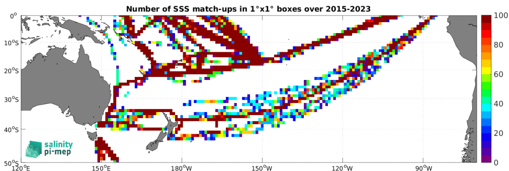
Figure 4: Number of SSS match-ups between TSG (LEGOS-DM) SSS and the SMAP SSS L2 v5 (RSS) SSS product for the South Pacific Ocean Pi-MEP region over 1^\circ \times 1^\circ boxes and for the full satellite product period.
