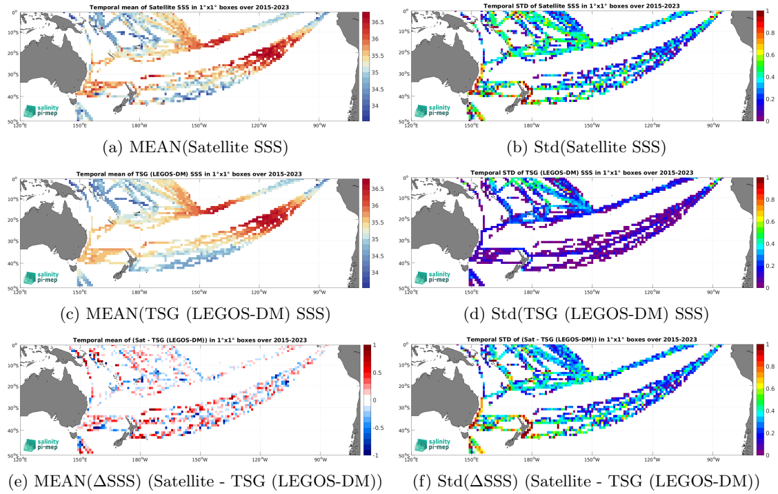
Figure 6: Temporal mean (left) and Std (right) of SSS from SMAP SSS L2 v5 (RSS) (top), TSG (LEGOS-DM) (middle), and of \Delta SSS (Satellite - TSG (LEGOS-DM)). Only match-up pairs are used to generate these maps.
