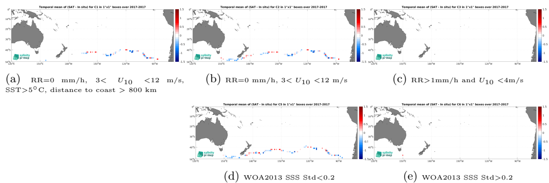
Figure 12: Temporal mean gridded over spatial boxes of size 1^\circ \times 1^\circ of \Delta\text{SSS} (SMAP SSS L2 v5 (RSS) - TSG (GOSUD-Sailing-ship)) for 5 different subdatasets corresponding to:RR=0 mm/h, 3 < U_{10} < 12 m/s, SST>5°C, distance to coast > 800 km (a), RR=0 mm/h, 3 < U_{10} < 12 m/s (b), RR>1mm/h and U_{10} < 4 m/s (c), WOA2013 SSS Std<0.2 (d), WOA2013 SSS Std>0.2 (e).
