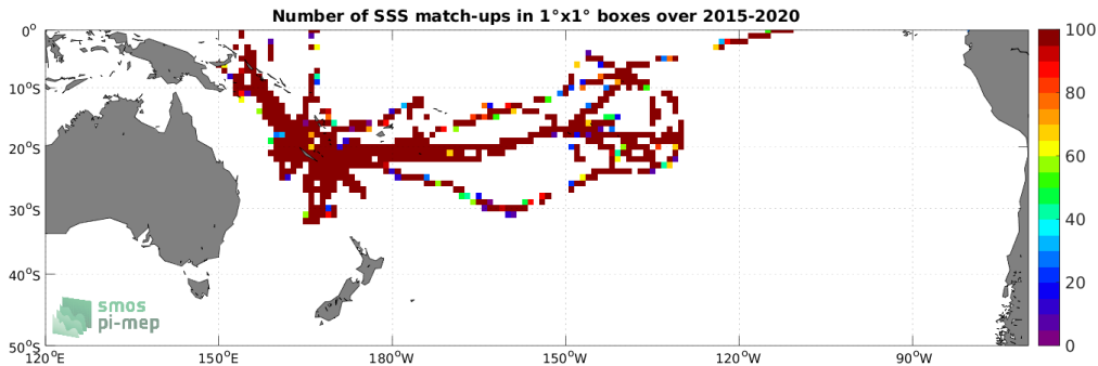
Figure 4: Number of SSS match-ups between TSG (GOSUD-Research-vessel) SSS and the SMAP SSS L2 v5 (RSS) SSS product for the South Pacific Ocean Pi-MEP region over 1^\circ \times 1^\circ boxes and for the full satellite product period.
