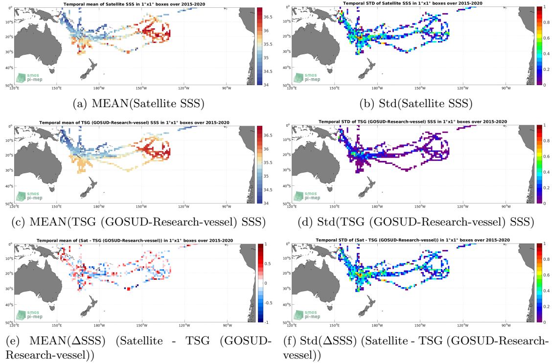
Figure 6: Temporal mean (left) and Std (right) of SSS from SMAP SSS L2 v5 (RSS) (top), TSG (GOSUD-Research-vessel) (middle), and of \Delta SSS (Satellite - TSG (GOSUD-Research-vessel)). Only match-up pairs are used to generate these maps.
