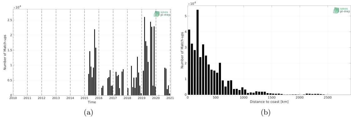
Figure 1: Number of match-ups between TSG (GOSUD-Research-vessel) and SMAP SSS L2 v5 (RSS) SSS as a function of time (a) and as function of the distance to coast (b) over the South Pacific Ocean Pi-MEP region and for the full satellite product period.
