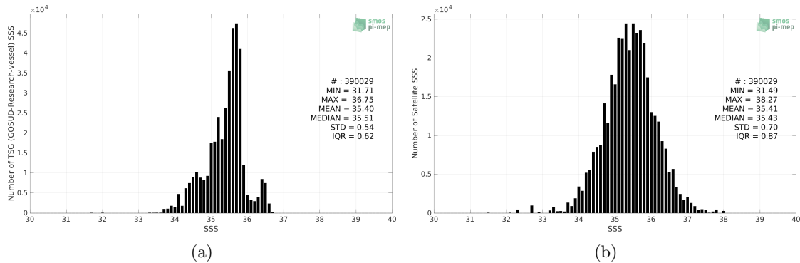
Figure 2: Histograms of SSS from TSG (GOSUD-Research-vessel) (a) and SMAP SSS L2 v5 (RSS) (b) considering all match-up pairs per bins of 0.1 over the South Pacific Ocean Pi-MEP region and for the full satellite product period.
