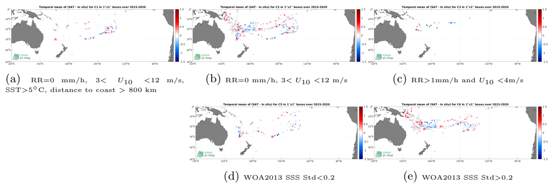
Figure 12: Temporal mean gridded over spatial boxes of size 1^\circ \times 1^\circ of \Delta SSS (SMAP SSS L2 v5 (RSS) - TSG (GOSUD-Research-vessel)) for 5 different subdatasets corresponding to:RR=0 mm/h, 3 < U_{10} < 12 m/s, SST>5°C, distance to coast > 800 km (a), RR=0 mm/h, 3 < U_{10} < 12 m/s (b), RR>1mm/h and U_{10} < 4 m/s (c), WOA2013 SSS Std<0.2 (d), WOA2013 SSS Std>0.2 (e).
