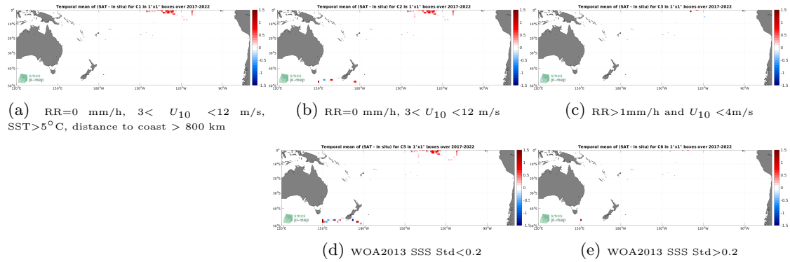
Figure 12: Temporal mean gridded over spatial boxes of size 1^\circ \times 1^\circ of \Delta SSS (SMAP SSS L2 v5 (RSS) - Saildrone) for 5 different subdatasets corresponding to:RR=0 mm/h, 3 < U_{10} < 12 m/s, SST >5^\circ C, distance to coast > 800 km (a), RR=0 mm/h, 3 < U_{10} < 12 m/s (b), RR >1 mm/h and U_{10} < 4 m/s (c), WOA2013 SSS Std <0.2 (d), WOA2013 SSS Std >0.2 (e).
