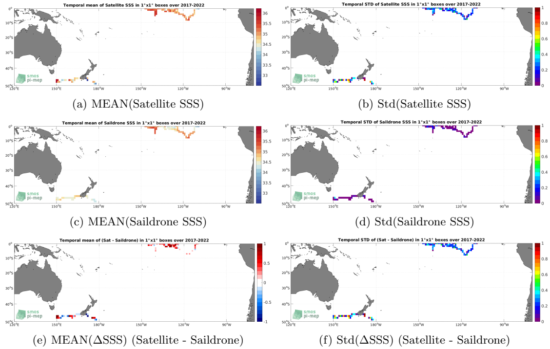
Figure 6: Temporal mean (left) and Std (right) of SSS from SMAP SSS L2 v5 (RSS) (top), Saildrone (middle), and of \Delta SSS (Satellite - Saildrone). Only match-up pairs are used to generate these maps.
