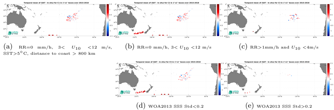
Figure 11: Temporal mean gridded over spatial boxes of size 1^\circ \times 1^\circ of \Delta\text{SSS} (SMAP SSS L2 v5 (RSS) - Surface drifters) for 5 different subdatasets corresponding to:RR=0 mm/h, 3 < U_{10} < 12 m/s, SST >5^\circ\text{C} , distance to coast > 800 km (a), RR=0 mm/h, 3 < U_{10} < 12 m/s (b), RR >1 mm/h and U_{10} < 4 m/s (c), WOA2013 SSS Std <0.2 (d), WOA2013 SSS Std >0.2 (e).
