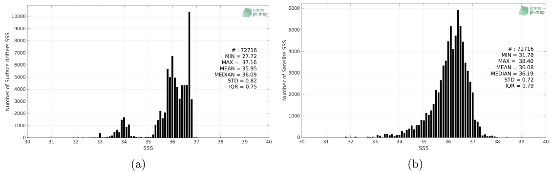
Figure 2: Histograms of SSS from Surface drifters (a) and SMAP SSS L2 v5 (RSS) (b) considering all match-up pairs per bins of 0.1 over the South Pacific Ocean Pi-MEP region and for the full satellite product period.
