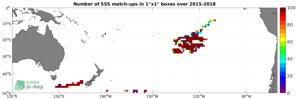
Figure 3: Number of SSS match-ups between Surface drifters SSS and the SMAP SSS L2 v5 (RSS) SSS product for the South Pacific Ocean Pi-MEP region over 1^\circ \times 1^\circ boxes and for the full satellite product period.
