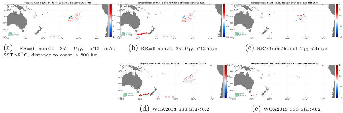
Figure 11: Temporal mean gridded over spatial boxes of size 1^\circ \times 1^\circ of \Delta SSS (SMAP SSS L2 v5 (RSS) - Surface drifters) for 5 different subdatasets corresponding to:RR=0 mm/h, 3 < U_{10} < 12 m/s, SST >5^\circ\text{C} , distance to coast > 800 km (a), RR=0 mm/h, 3 < U_{10} < 12 m/s (b), RR >1 mm/h and U_{10} < 4 m/s (c), WOA2013 SSS Std <0.2 (d), WOA2013 SSS Std >0.2 (e).
