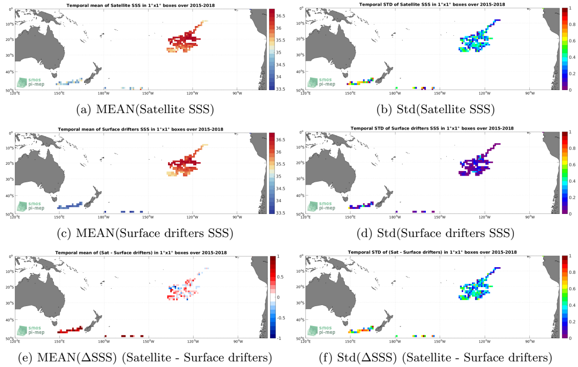
Figure 5: Temporal mean (left) and Std (right) of SSS from SMAP SSS L2 v5 (RSS) (top), Surface drifters (middle), and of \Delta SSS (Satellite - Surface drifters). Only match-up pairs are used to generate these maps.
