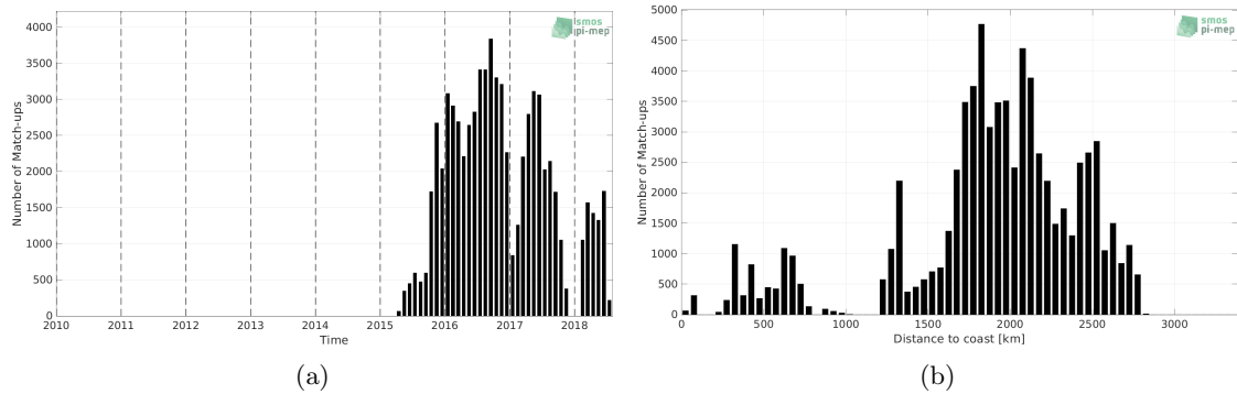
Figure 1: Number of match-ups between Surface drifters and SMAP SSS L2 v5 (RSS) SSS as a function of time (a) and as function of the distance to coast (b) over the South Pacific Ocean Pi-MEP region and for the full satellite product period.
