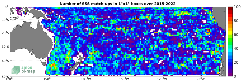
Figure 4: Number of SSS match-ups between Argo SSS and the SMAP SSS L2 v5 (RSS) SSS product for the South Pacific Ocean Pi-MEP region over 1^\circ \times 1^\circ boxes and for the full satellite product period.
