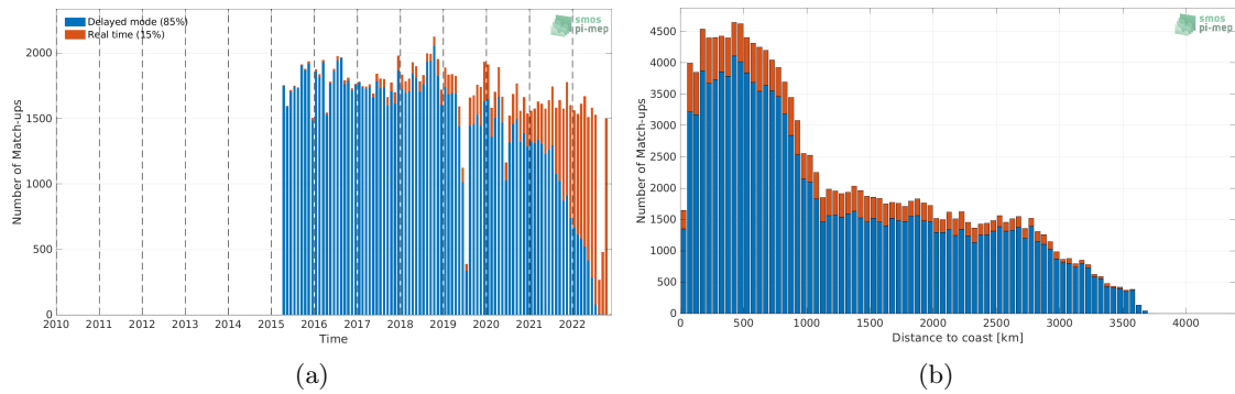
Figure 1: Number of match-ups between Argo and SMAP SSS L2 v5 (RSS) SSS as a function of time (a) and as function of the distance to coast (b) over the South Pacific Ocean Pi-MEP region and for the full satellite product period.
