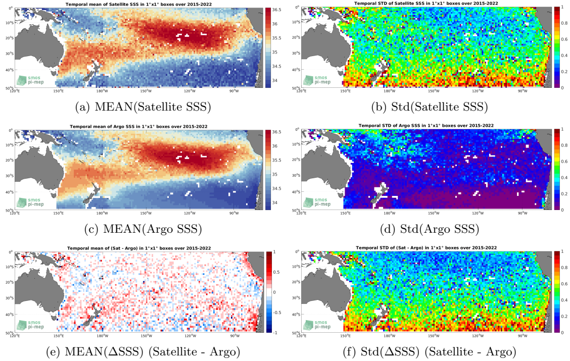
Figure 6: Temporal mean (left) and Std (right) of SSS from SMAP SSS L2 v5 (RSS) (top), Argo (middle), and of \Delta SSS (Satellite - Argo). Only match-up pairs are used to generate these maps.
