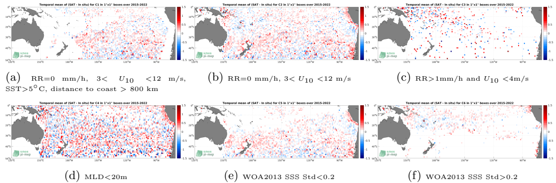
Figure 12: Temporal mean gridded over spatial boxes of size 1^\circ \times 1^\circ of \Delta SSS (SMAP SSS L2 v5 (RSS) - Argo) for 6 different subdatasets corresponding to:RR=0 mm/h, 3 < U_{10} < 12 m/s, SST >5^\circ C, distance to coast > 800 km (a), RR=0 mm/h, 3 < U_{10} < 12 m/s (b), RR >1 mm/h and U_{10} < 4 m/s (c),MLD <20 m (d),WOA2013 SSS Std <0.2 (e),WOA2013 SSS Std >0.2 (f).
