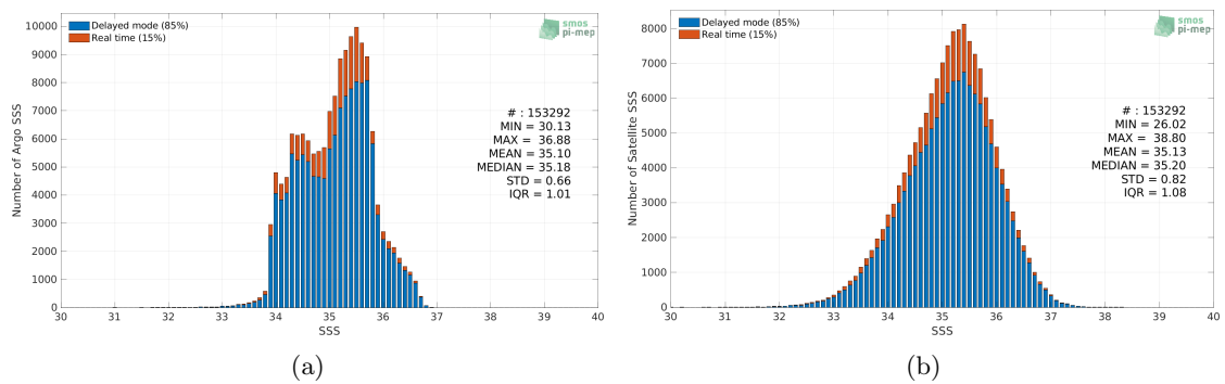
Figure 2: Histograms of SSS from Argo (a) and SMAP SSS L2 v5 (RSS) (b) considering all match-up pairs per bins of 0.1 over the South Pacific Ocean Pi-MEP region and for the full satellite product period.
