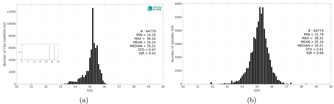
Figure 3: Histograms of SSS from TSG (SAMOS) (a) and SMAP SSS L2 v5.3 (RSS) (b) considering all match-up pairs per bins of 0.1 over the South Pacific Ocean Pi-MEP region and for the full satellite product period.
