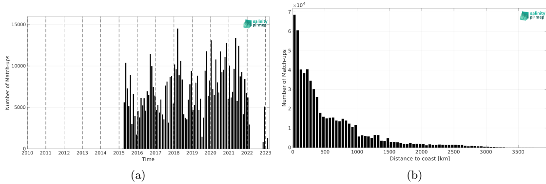
Figure 2: Number of match-ups between TSG (LEGOS-DM) and SMAP SSS L2 v5.3 (RSS) SSS as a function of time (a) and as function of the distance to coast (b) over the South Pacific Ocean Pi-MEP region and for the full satellite product period.
