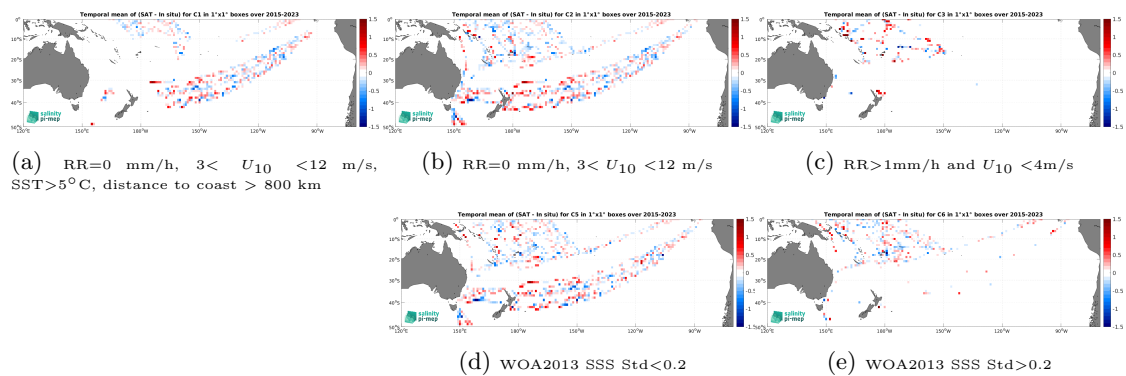
Figure 14: Temporal mean gridded over spatial boxes of size 1^\circ \times 1^\circ of \Delta\text{SSS} (SMAP SSS L2 v5.3 (RSS) - TSG (LEGOS-DM)) for 5 different subdatasets corresponding to:RR=0 mm/h, 3 < U_{10} < 12 m/s, SST>5°C, distance to coast > 800 km (a), RR=0 mm/h, 3 < U_{10} < 12 m/s (b), RR>1mm/h and U_{10} < 4 m/s (c), WOA2013 SSS Std<0.2 (d), WOA2013 SSS Std>0.2 (e).
