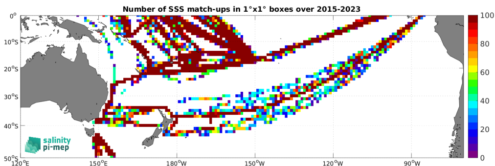
Figure 5: Number of SSS match-ups between TSG (LEGOS-DM) SSS and the SMAP SSS L2 v5.3 (RSS) SSS product for the South Pacific Ocean Pi-MEP region over 1^\circ \times 1^\circ boxes and for the full satellite product period.
