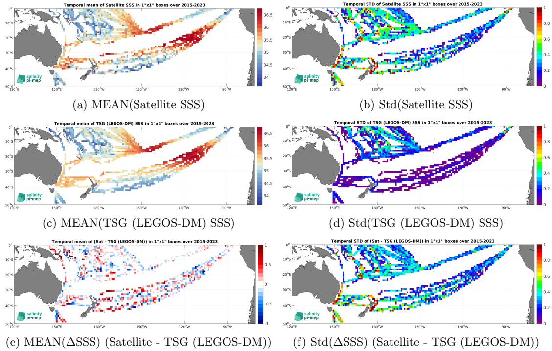
Figure 7: Temporal mean (left) and Std (right) of SSS from SMAP SSS L2 v5.3 (RSS) (top), TSG (LEGOS-DM) (middle), and of \Delta SSS (Satellite - TSG (LEGOS-DM)). Only match-up pairs are used to generate these maps.
