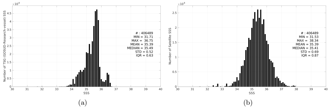
Figure 3: Histograms of SSS from TSG (GOSUD-Research-vessel) (a) and SMAP SSS L2 v5.3 (RSS) (b) considering all match-up pairs per bins of 0.1 over the South Pacific Ocean Pi-MEP region and for the full satellite product period.
