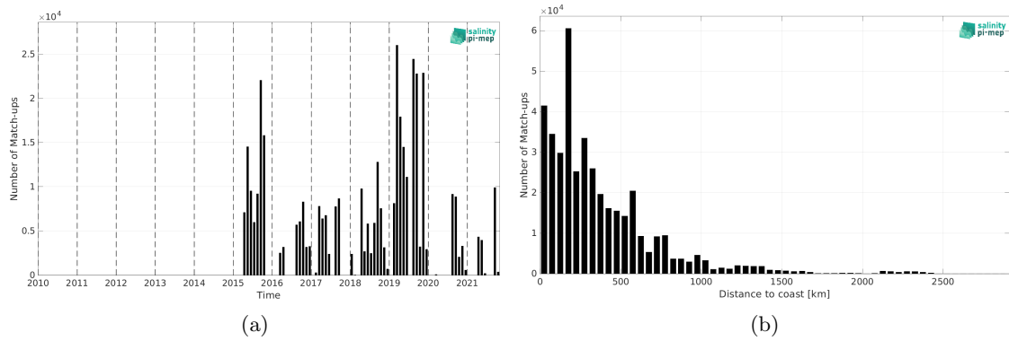
Figure 2: Number of match-ups between TSG (GOSUD-Research-vessel) and SMAP SSS L2 v5.3 (RSS) SSS as a function of time (a) and as function of the distance to coast (b) over the South Pacific Ocean Pi-MEP region and for the full satellite product period.
