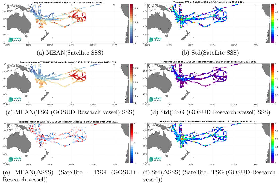
Figure 7: Temporal mean (left) and Std (right) of SSS from SMAP SSS L2 v5.3 (RSS) (top), TSG (GOSUD-Research-vessel) (middle), and of \Delta SSS (Satellite - TSG (GOSUD-Research-vessel)). Only match-up pairs are used to generate these maps.
