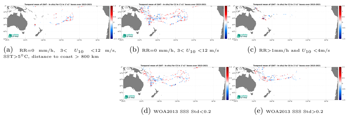
Figure 14: Temporal mean gridded over spatial boxes of size 1^\circ \times 1^\circ of \Delta SSS (SMAP SSS L2 v5.3 (RSS) - TSG (GOSUD-Research-vessel)) for 5 different subdatasets corresponding to:RR=0 mm/h, 3 < U_{10} < 12 m/s, SST > 5°C, distance to coast > 800 km (a), RR=0 mm/h, 3 < U_{10} < 12 m/s (b), RR > 1mm/h and U_{10} < 4 m/s (c), WOA2013 SSS Std < 0.2 (d), WOA2013 SSS Std > 0.2 (e).
