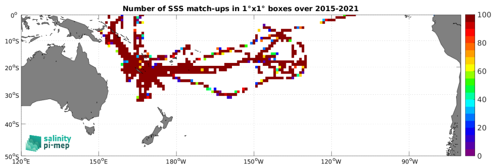
Figure 5: Number of SSS match-ups between TSG (GOSUD-Research-vessel) SSS and the SMAP SSS L2 v5.3 (RSS) SSS product for the South Pacific Ocean Pi-MEP region over 1^\circ \times 1^\circ boxes and for the full satellite product period.
