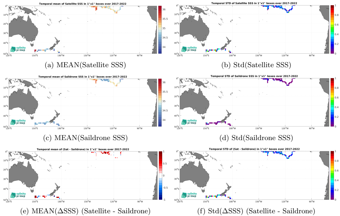
Figure 7: Temporal mean (left) and Std (right) of SSS from SMAP SSS L2 v5.3 (RSS) (top), Saildrone (middle), and of \Delta SSS (Satellite - Saildrone). Only match-up pairs are used to generate these maps.
