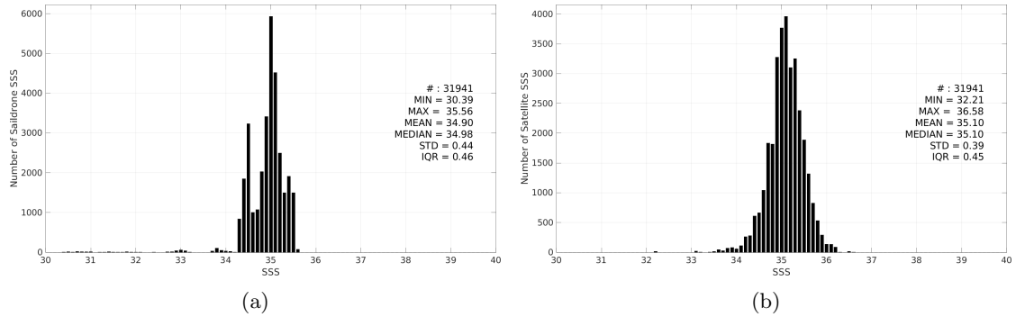
Figure 3: Histograms of SSS from Saildrone (a) and SMAP SSS L2 v5.3 (RSS) (b) considering all match-up pairs per bins of 0.1 over the South Pacific Ocean Pi-MEP region and for the full satellite product period.
