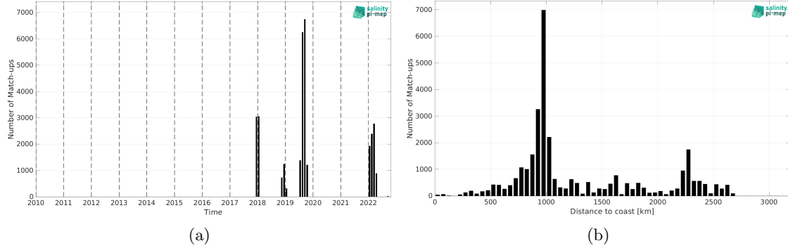
Figure 2: Number of match-ups between Saildrone and SMAP SSS L2 v5.3 (RSS) SSS as a function of time (a) and as function of the distance to coast (b) over the South Pacific Ocean Pi-MEP region and for the full satellite product period.
