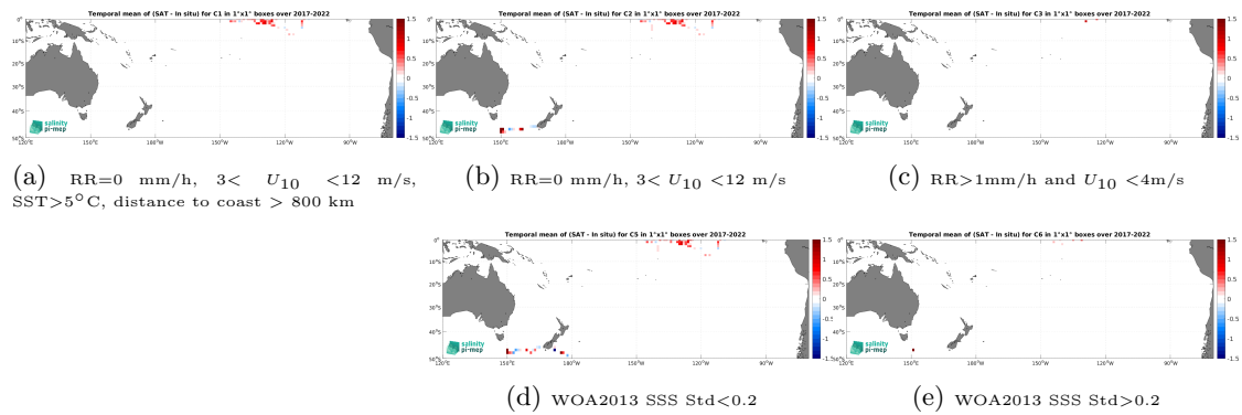
Figure 14: Temporal mean gridded over spatial boxes of size 1^\circ \times 1^\circ of \Delta SSS (SMAP SSS L2 v5.3 (RSS) - Saildrone) for 5 different subdatasets corresponding to:RR=0 mm/h, 3 < U_{10} < 12 m/s, SST >5^\circ C, distance to coast > 800 km (a), RR=0 mm/h, 3 < U_{10} < 12 m/s (b), RR >1 mm/h and U_{10} < 4 m/s (c), WOA2013 SSS Std <0.2 (d), WOA2013 SSS Std >0.2 (e).
