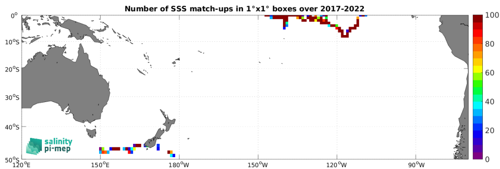
Figure 5: Number of SSS match-ups between Saildrone SSS and the SMAP SSS L2 v5.3 (RSS) SSS product for the South Pacific Ocean Pi-MEP region over 1^\circ \times 1^\circ boxes and for the full satellite product period.
