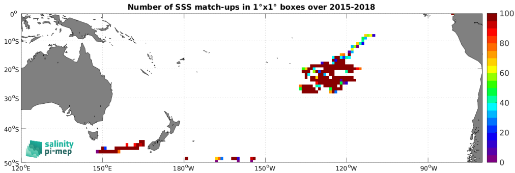
Figure 4: Number of SSS match-ups between Surface drifters SSS and the SMAP SSS L2 v5.3 (RSS) SSS product for the South Pacific Ocean Pi-MEP region over 1^\circ \times 1^\circ boxes and for the full satellite product period.
