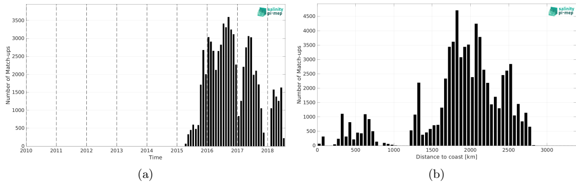
Figure 2: Number of match-ups between Surface drifters and SMAP SSS L2 v5.3 (RSS) SSS as a function of time (a) and as function of the distance to coast (b) over the South Pacific Ocean Pi-MEP region and for the full satellite product period.
