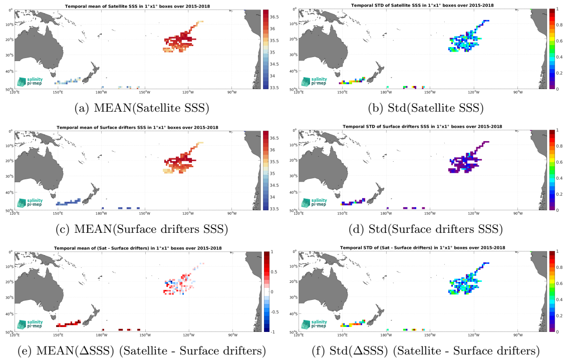
Figure 6: Temporal mean (left) and Std (right) of SSS from SMAP SSS L2 v5.3 (RSS) (top), Surface drifters (middle), and of \Delta SSS (Satellite - Surface drifters). Only match-up pairs are used to generate these maps.
