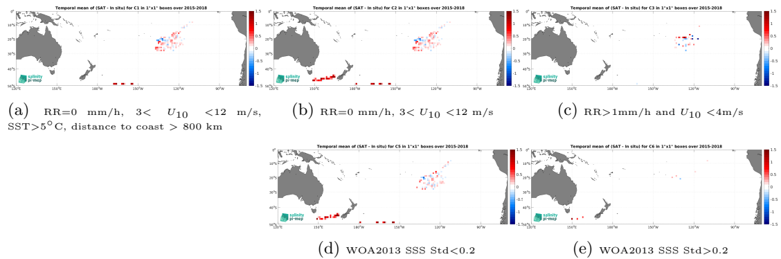
Figure 13: Temporal mean gridded over spatial boxes of size 1^\circ \times 1^\circ of \Delta SSS (SMAP SSS L2 v5.3 (RSS) - Surface drifters) for 5 different subdatasets corresponding to:RR=0 mm/h, 3 < U_{10} < 12 m/s, SST >5^\circ\text{C} , distance to coast > 800 km (a), RR=0 mm/h, 3 < U_{10} < 12 m/s (b), RR >1 mm/h and U_{10} < 4 m/s (c), WOA2013 SSS Std <0.2 (d), WOA2013 SSS Std >0.2 (e).
