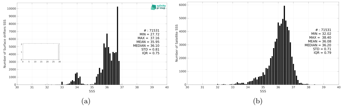
Figure 3: Histograms of SSS from Surface drifters (a) and SMAP SSS L2 v5.3 (RSS) (b) considering all match-up pairs per bins of 0.1 over the South Pacific Ocean Pi-MEP region and for the full satellite product period.
