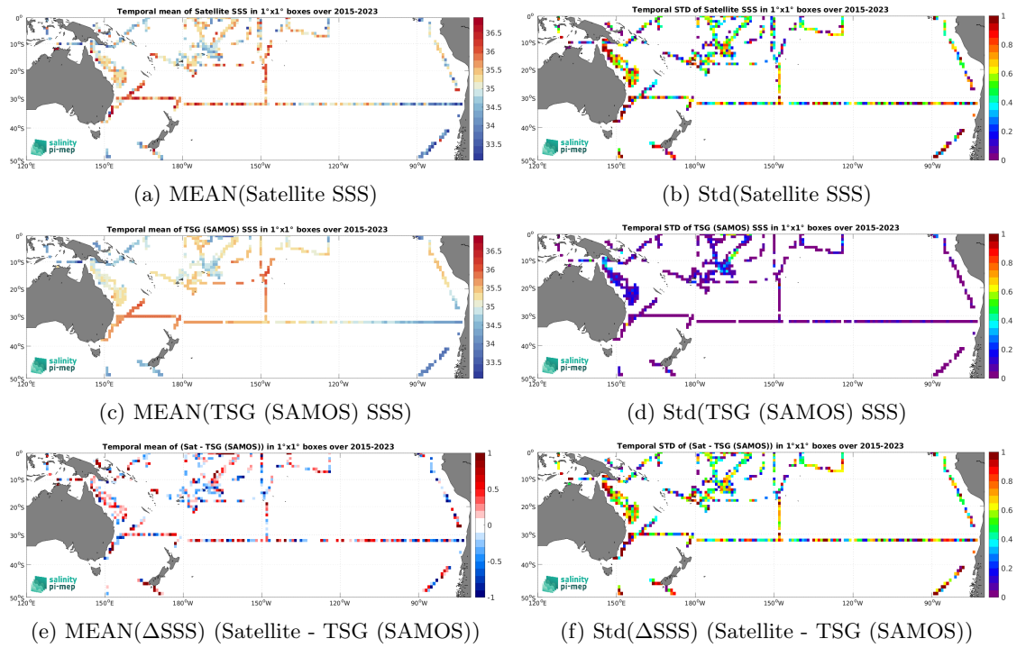
Figure 7: Temporal mean (left) and Std (right) of SSS from SMAP SSS L2 v5.3 - 40 km (RSS) (top), TSG (SAMOS) (middle), and of \Delta SSS (Satellite - TSG (SAMOS)). Only match-up pairs are used to generate these maps.
