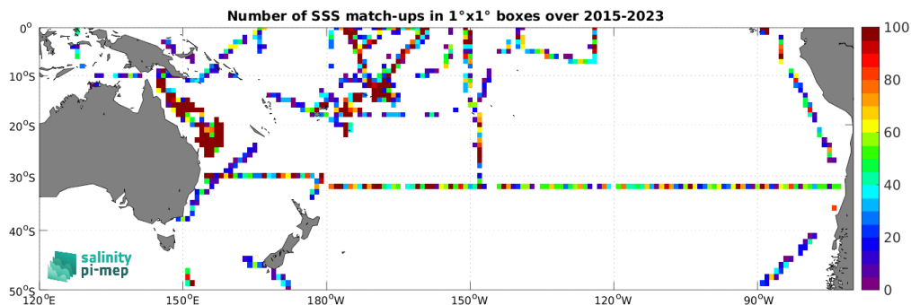
Figure 5: Number of SSS match-ups between TSG (SAMOS) SSS and the SMAP SSS L2 v5.3 - 40 km (RSS) SSS product for the South Pacific Ocean Pi-MEP region over 1^\circ \times 1^\circ boxes and for the full satellite product period.
