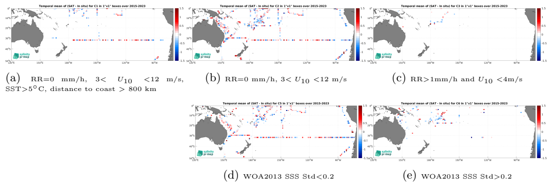
Figure 14: Temporal mean gridded over spatial boxes of size 1^\circ \times 1^\circ of \Delta SSS (SMAP SSS L2 v5.3 - 40 km (RSS) - TSG (SAMOS)) for 5 different subdatasets corresponding to:RR=0 mm/h, 3 < U_{10} < 12 m/s, SST >5^\circ C, distance to coast > 800 km (a), RR=0 mm/h, 3 < U_{10} < 12 m/s (b), RR >1 mm/h and U_{10} < 4 m/s (c), WOA2013 SSS Std <0.2 (d), WOA2013 SSS Std >0.2 (e).
