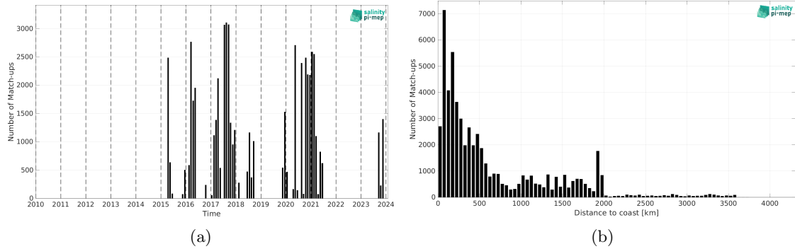
Figure 2: Number of match-ups between TSG (SAMOS) and SMAP SSS L2 v5.3 - 40 km (RSS) SSS as a function of time (a) and as function of the distance to coast (b) over the South Pacific Ocean Pi-MEP region and for the full satellite product period.
