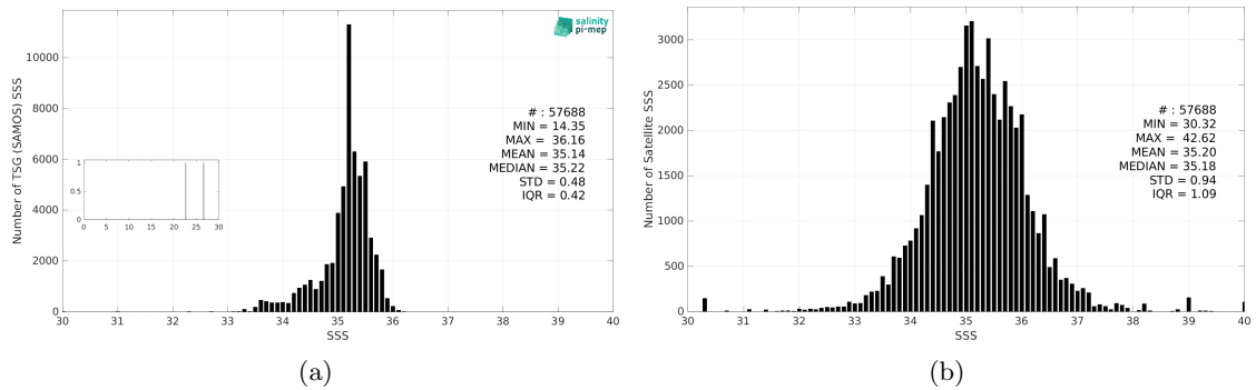
Figure 3: Histograms of SSS from TSG (SAMOS) (a) and SMAP SSS L2 v5.3 - 40 km (RSS) (b) considering all match-up pairs per bins of 0.1 over the South Pacific Ocean Pi-MEP region and for the full satellite product period.
