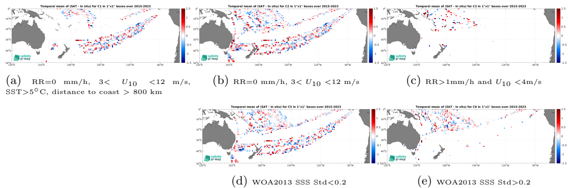
Figure 14: Temporal mean gridded over spatial boxes of size 1^\circ \times 1^\circ of \Delta\text{SSS} (SMAP SSS L2 v5.3 - 40 km (RSS) - TSG (LEGOS-DM)) for 5 different subdatasets corresponding to:RR=0 mm/h, 3 < U_{10} < 12 m/s, SST>5°C, distance to coast > 800 km (a), RR=0 mm/h, 3 < U_{10} < 12 m/s (b), RR>1mm/h and U_{10} < 4 m/s (c), WOA2013 SSS Std<0.2 (d), WOA2013 SSS Std>0.2 (e).
