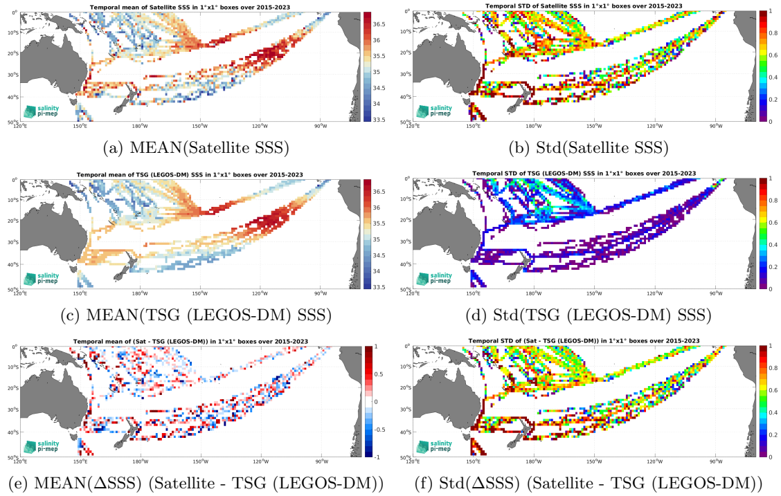
Figure 7: Temporal mean (left) and Std (right) of SSS from SMAP SSS L2 v5.3 - 40 km (RSS) (top), TSG (LEGOS-DM) (middle), and of \Delta SSS (Satellite - TSG (LEGOS-DM)). Only match-up pairs are used to generate these maps.
