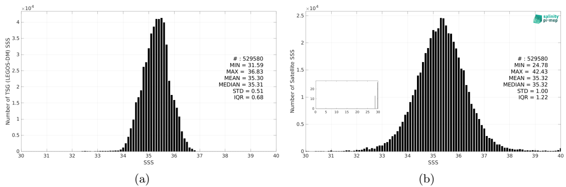
Figure 3: Histograms of SSS from TSG (LEGOS-DM) (a) and SMAP SSS L2 v5.3 - 40 km (RSS) (b) considering all match-up pairs per bins of 0.1 over the South Pacific Ocean Pi-MEP region and for the full satellite product period.
