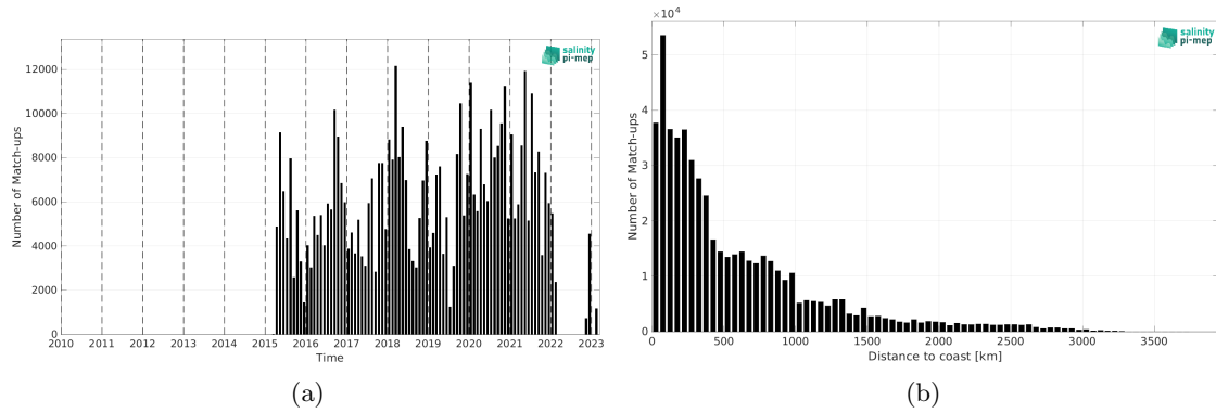
Figure 2: Number of match-ups between TSG (LEGOS-DM) and SMAP SSS L2 v5.3 - 40 km (RSS) SSS as a function of time (a) and as function of the distance to coast (b) over the South Pacific Ocean Pi-MEP region and for the full satellite product period.
