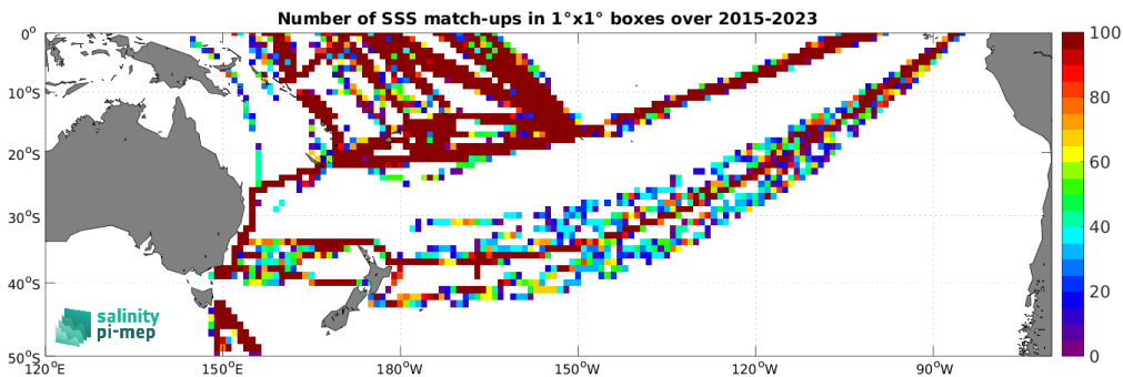
Figure 5: Number of SSS match-ups between TSG (LEGOS-DM) SSS and the SMAP SSS L2 v5.3 - 40 km (RSS) SSS product for the South Pacific Ocean Pi-MEP region over 1^\circ \times 1^\circ boxes and for the full satellite product period.
