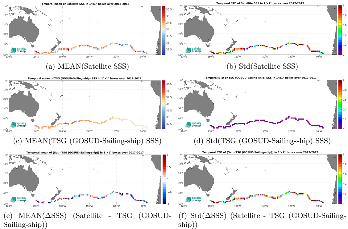
Figure 7: Temporal mean (left) and Std (right) of SSS from SMAP SSS L2 v5.3 - 40 km (RSS) (top), TSG (GOSUD-Sailing-ship) (middle), and of \Delta SSS (Satellite - TSG (GOSUD-Sailing-ship)). Only match-up pairs are used to generate these maps.
