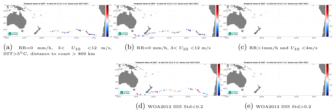
Figure 14: Temporal mean gridded over spatial boxes of size 1^\circ \times 1^\circ of \Delta SSS (SMAP SSS L2 v5.3 - 40 km (RSS) - TSG (GOSUD-Sailing-ship)) for 5 different subdatasets corresponding to:RR=0 mm/h, 3 < U_{10} < 12 m/s, SST>5°C, distance to coast > 800 km (a), RR=0 mm/h, 3 < U_{10} < 12 m/s (b), RR>1mm/h and U_{10} < 4 m/s (c), WOA2013 SSS Std<0.2 (d), WOA2013 SSS Std>0.2 (e).
