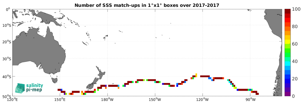
Figure 5: Number of SSS match-ups between TSG (GOSUD-Sailing-ship) SSS and the SMAP SSS L2 v5.3 - 40 km (RSS) SSS product for the South Pacific Ocean Pi-MEP region over 1^\circ \times 1^\circ boxes and for the full satellite product period.
