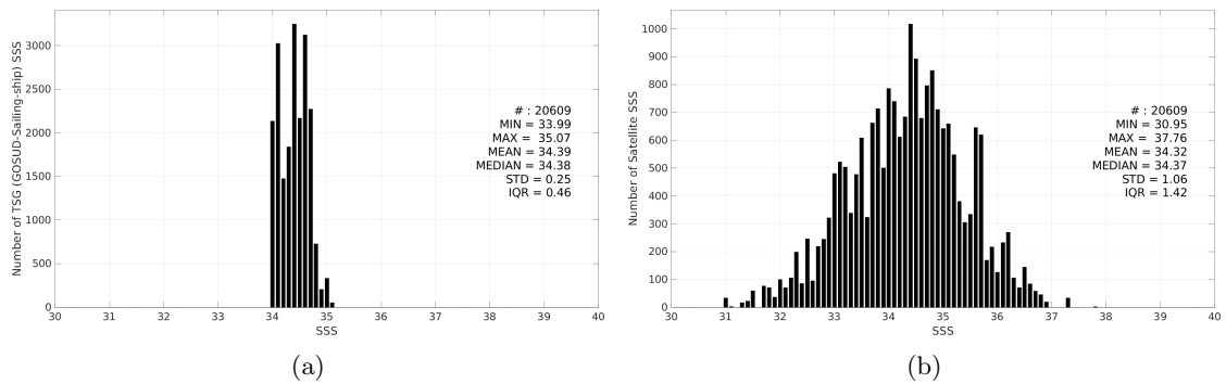
Figure 3: Histograms of SSS from TSG (GOSUD-Sailing-ship) (a) and SMAP SSS L2 v5.3 - 40 km (RSS) (b) considering all match-up pairs per bins of 0.1 over the South Pacific Ocean Pi-MEP region and for the full satellite product period.
