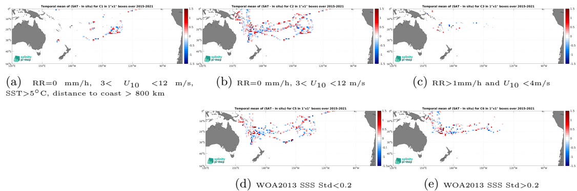
Figure 14: Temporal mean gridded over spatial boxes of size 1^\circ \times 1^\circ of \Delta SSS (SMAP SSS L2 v5.3 - 40 km (RSS) - TSG (GOSUD-Research-vessel)) for 5 different subdatasets corresponding to:RR=0 mm/h, 3 < U_{10} < 12 m/s, SST >5^\circ\text{C} , distance to coast > 800 km (a), RR=0 mm/h, 3 < U_{10} < 12 m/s (b), RR >1 mm/h and U_{10} < 4 m/s (c), WOA2013 SSS Std <0.2 (d), WOA2013 SSS Std >0.2 (e).
