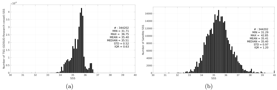
Figure 3: Histograms of SSS from TSG (GOSUD-Research-vessel) (a) and SMAP SSS L2 v5.3 - 40 km (RSS) (b) considering all match-up pairs per bins of 0.1 over the South Pacific Ocean Pi-MEP region and for the full satellite product period.
