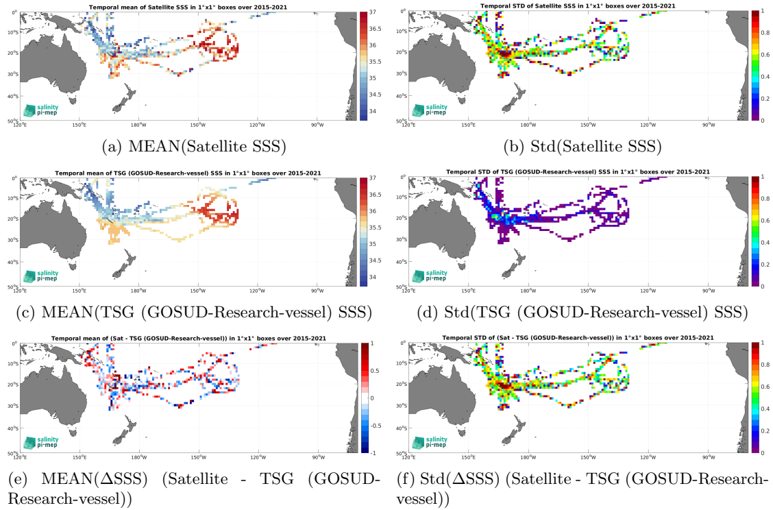
Figure 7: Temporal mean (left) and Std (right) of SSS from SMAP SSS L2 v5.3 - 40 km (RSS) (top), TSG (GOSUD-Research-vessel) (middle), and of \Delta SSS (Satellite - TSG (GOSUD-Research-vessel)). Only match-up pairs are used to generate these maps.
