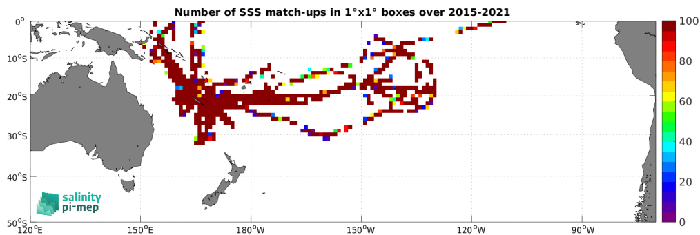
Figure 5: Number of SSS match-ups between TSG (GOSUD-Research-vessel) SSS and the SMAP SSS L2 v5.3 - 40 km (RSS) SSS product for the South Pacific Ocean Pi-MEP region over 1^\circ \times 1^\circ boxes and for the full satellite product period.
