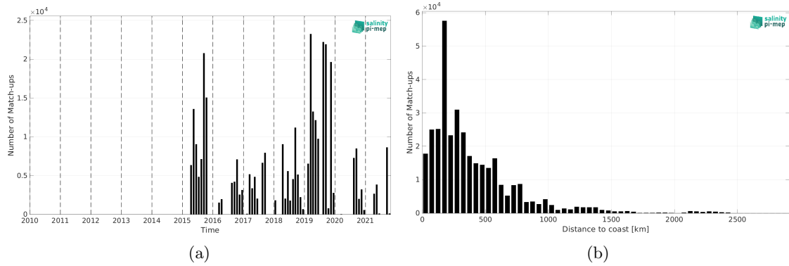
Figure 2: Number of match-ups between TSG (GOSUD-Research-vessel) and SMAP SSS L2 v5.3 - 40 km (RSS) SSS as a function of time (a) and as function of the distance to coast (b) over the South Pacific Ocean Pi-MEP region and for the full satellite product period.
