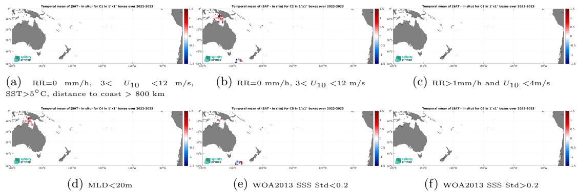
Figure 14: Temporal mean gridded over spatial boxes of size 1^\circ \times 1^\circ of \Delta SSS (SMAP SSS L2 v5.3 - 40 km (RSS) - Marine mammals) for 6 different subdatasets corresponding to:RR=0 mm/h, 3 < U_{10} < 12 m/s, SST>5°C, distance to coast > 800 km (a), RR=0 mm/h, 3 < U_{10} < 12 m/s (b), RR>1mm/h and U_{10} < 4 m/s (c),MLD<20m (d),WOA2013 SSS Std<0.2 (e),WOA2013 SSS Std>0.2 (f).
