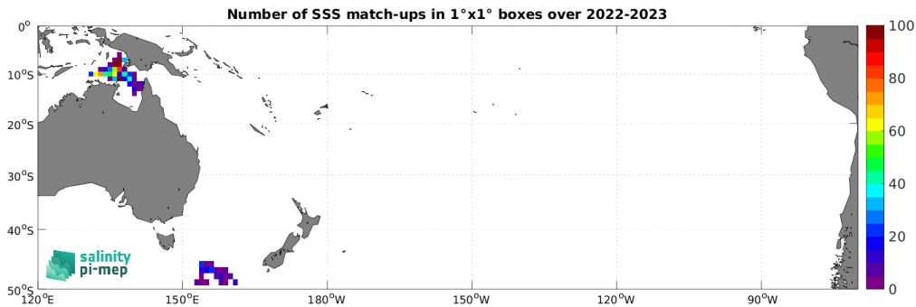
Figure 5: Number of SSS match-ups between Marine mammals SSS and the SMAP SSS L2 v5.3 - 40 km (RSS) SSS product for the South Pacific Ocean Pi-MEP region over 1^\circ \times 1^\circ boxes and for the full satellite product period.
