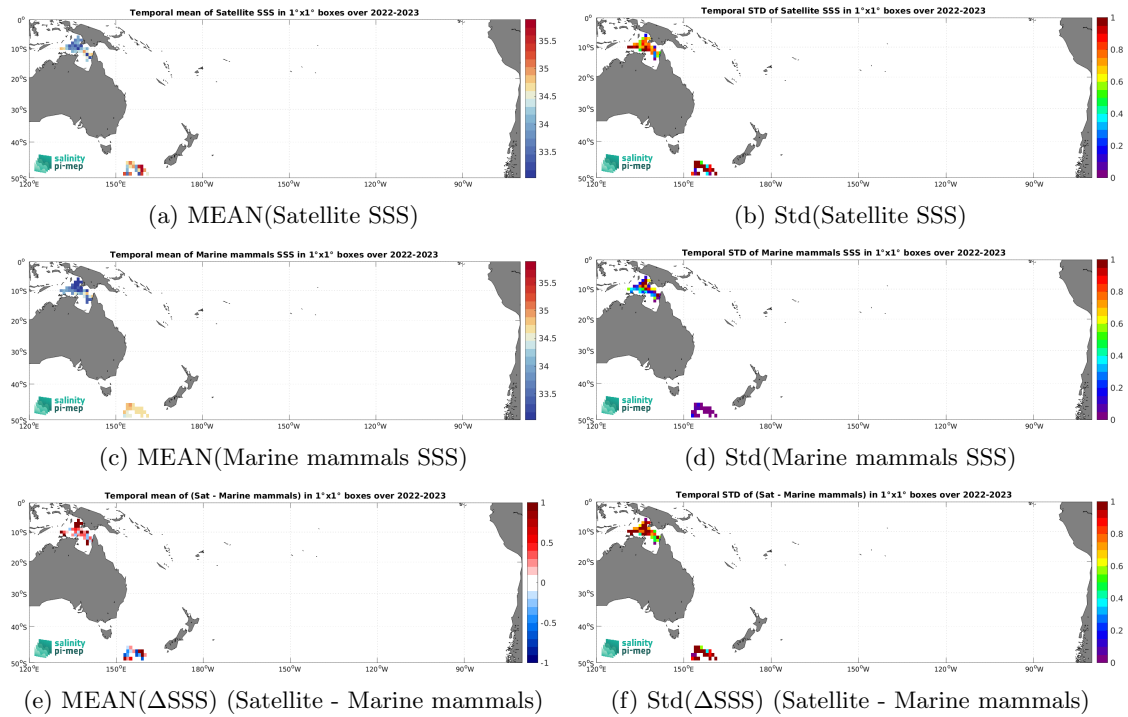
Figure 7: Temporal mean (left) and Std (right) of SSS from SMAP SSS L2 v5.3 - 40 km (RSS) (top), Marine mammals (middle), and of \Delta SSS (Satellite - Marine mammals). Only match-up pairs are used to generate these maps.
