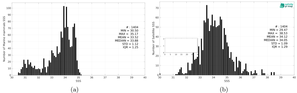
Figure 3: Histograms of SSS from Marine mammals (a) and SMAP SSS L2 v5.3 - 40 km (RSS) (b) considering all match-up pairs per bins of 0.1 over the South Pacific Ocean Pi-MEP region and for the full satellite product period.
