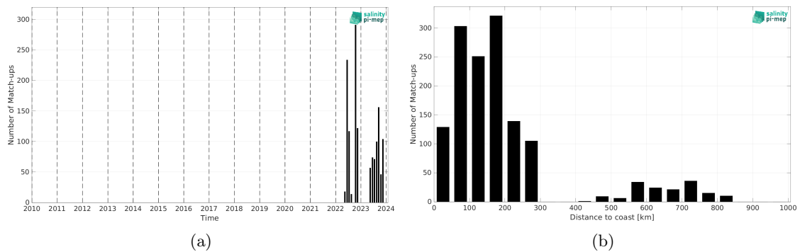
Figure 2: Number of match-ups between Marine mammals and SMAP SSS L2 v5.3 - 40 km (RSS) SSS as a function of time (a) and as function of the distance to coast (b) over the South Pacific Ocean Pi-MEP region and for the full satellite product period.
