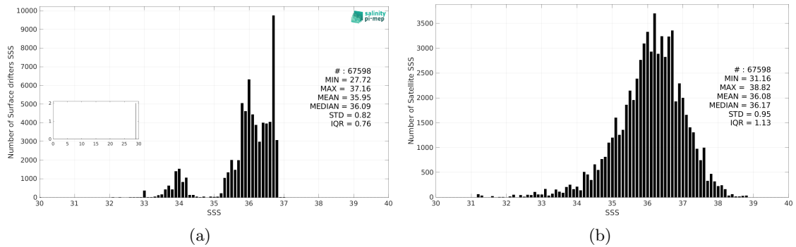
Figure 3: Histograms of SSS from Surface drifters (a) and SMAP SSS L2 v5.3 - 40 km (RSS) (b) considering all match-up pairs per bins of 0.1 over the South Pacific Ocean Pi-MEP region and for the full satellite product period.
