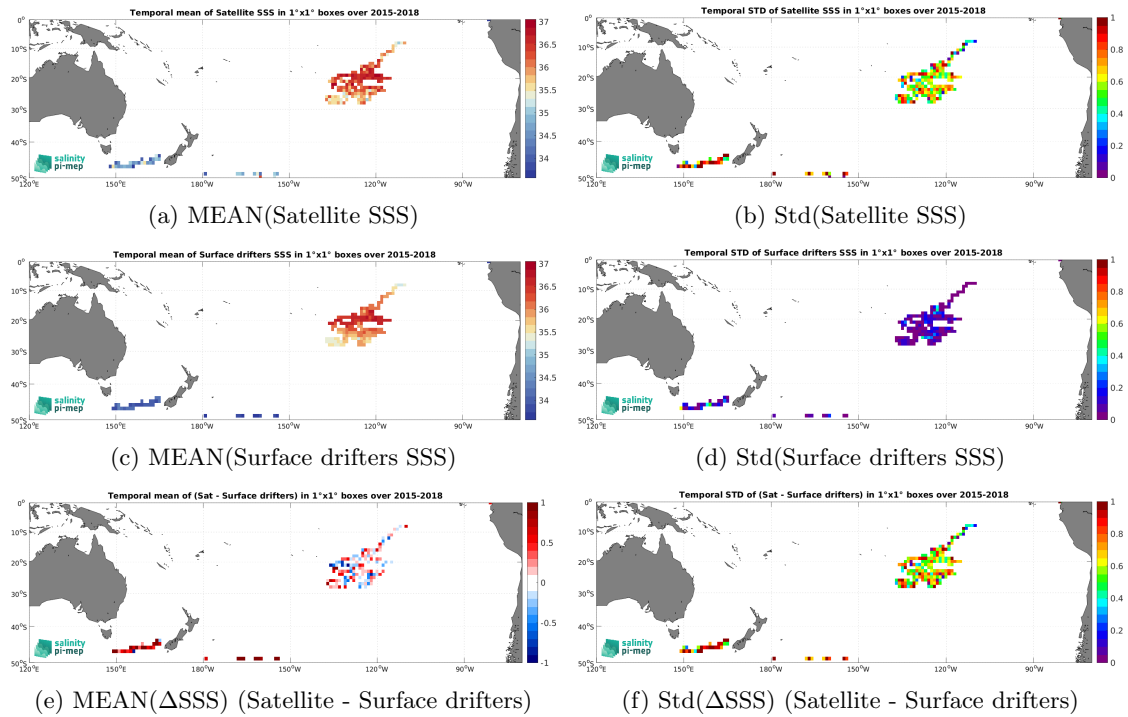
Figure 6: Temporal mean (left) and Std (right) of SSS from SMAP SSS L2 v5.3 - 40 km (RSS) (top), Surface drifters (middle), and of \Delta SSS (Satellite - Surface drifters). Only match-up pairs are used to generate these maps.
