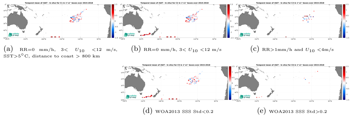
Figure 13: Temporal mean gridded over spatial boxes of size 1^\circ \times 1^\circ of \Delta SSS (SMAP SSS L2 v5.3 - 40 km (RSS) - Surface drifters) for 5 different subdatasets corresponding to: RR=0 mm/h, 3 < U_{10} < 12 m/s, SST > 5^\circ\text{C} , distance to coast > 800 km (a), RR=0 mm/h, 3 < U_{10} < 12 m/s (b), RR > 1 mm/h and U_{10} < 4 m/s (c), WOA2013 SSS Std < 0.2 (d), WOA2013 SSS Std > 0.2 (e).
