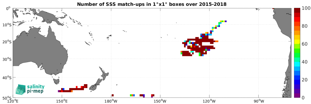
Figure 4: Number of SSS match-ups between Surface drifters SSS and the SMAP SSS L2 v5.3 - 40 km (RSS) SSS product for the South Pacific Ocean Pi-MEP region over 1^\circ \times 1^\circ boxes and for the full satellite product period.
