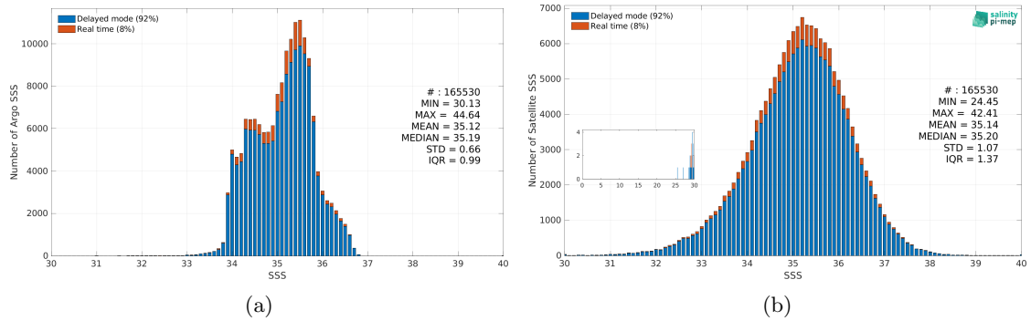
Figure 3: Histograms of SSS from Argo (a) and SMAP SSS L2 v5.3 - 40 km (RSS) (b) considering all match-up pairs per bins of 0.1 over the South Pacific Ocean Pi-MEP region and for the full satellite product period.
