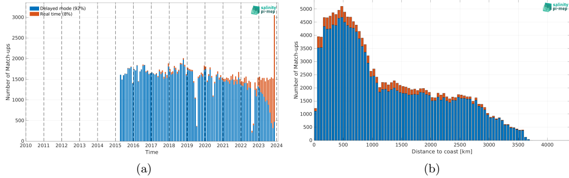
Figure 2: Number of match-ups between Argo and SMAP SSS L2 v5.3 - 40 km (RSS) SSS as a function of time (a) and as function of the distance to coast (b) over the South Pacific Ocean Pi-MEP region and for the full satellite product period.
