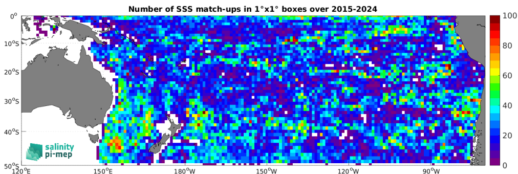
Figure 5: Number of SSS match-ups between Argo SSS and the SMAP SSS L2 v5.3 - 40 km (RSS) SSS product for the South Pacific Ocean Pi-MEP region over 1^\circ \times 1^\circ boxes and for the full satellite product period.
