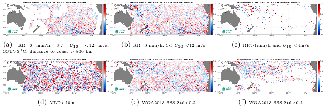
Figure 14: Temporal mean gridded over spatial boxes of size 1^\circ \times 1^\circ of \Delta SSS (SMAP SSS L2 v5.3 - 40 km (RSS) - Argo) for 6 different subdatasets corresponding to: RR=0 mm/h, 3 < U_{10} < 12 m/s, SST > 5°C, distance to coast > 800 km (a), RR=0 mm/h, 3 < U_{10} < 12 m/s (b), RR > 1mm/h and U_{10} < 4 m/s (c), MLD < 20m (d), WOA2013 SSS Std < 0.2 (e), WOA2013 SSS Std > 0.2 (f).
