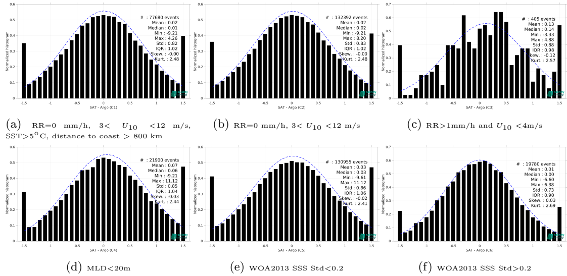
Figure 15: Normalized histogram of \Delta SSS (SMAP SSS L2 v5.3 - 40 km (RSS) - Argo) for 6 different subdatasets corresponding to: RR=0 mm/h, 3 < U_{10} < 12 m/s, SST > 5°C, distance to coast > 800 km (a), RR=0 mm/h, 3 < U_{10} < 12 m/s (b), RR > 1mm/h and U_{10} < 4 m/s (c), MLD < 20m (d), WOA2013 SSS Std < 0.2 (e), WOA2013 SSS Std > 0.2 (f).
