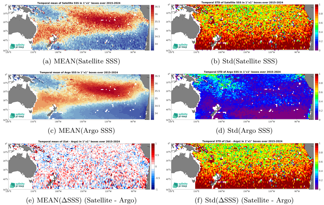
Figure 7: Temporal mean (left) and Std (right) of SSS from SMAP SSS L2 v5.3 - 40 km (RSS) (top), Argo (middle), and of \Delta SSS (Satellite - Argo). Only match-up pairs are used to generate these maps.
