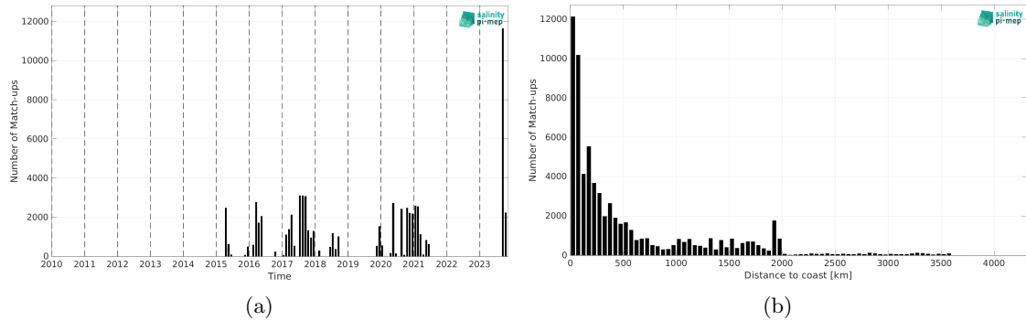
Figure 1: Number of match-ups between TSG (SAMOS) and SMAP SSS L2 v5 - 40 km (RSS) SSS as a function of time (a) and as function of the distance to coast (b) over the South Pacific Ocean Pi-MEP region and for the full satellite product period.
