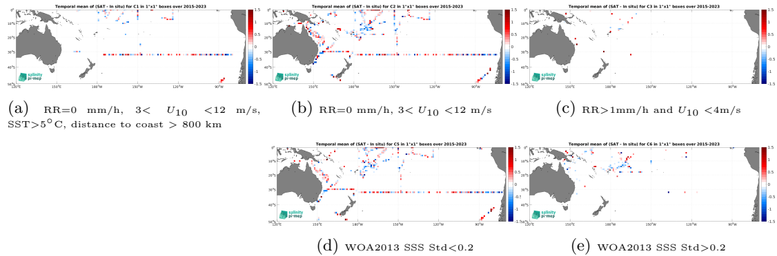
Figure 12: Temporal mean gridded over spatial boxes of size 1^\circ \times 1^\circ of \Delta\text{SSS} (SMAP SSS L2 v5 - 40 km (RSS) - TSG (SAMOS)) for 5 different subdatasets corresponding to:RR=0 mm/h, 3 < U_{10} < 12 m/s, SST >5^\circ\text{C} , distance to coast > 800 km (a), RR=0 mm/h, 3 < U_{10} < 12 m/s (b), RR >1 mm/h and U_{10} < 4 m/s (c), WOA2013 SSS Std <0.2 (d), WOA2013 SSS Std >0.2 (e).
