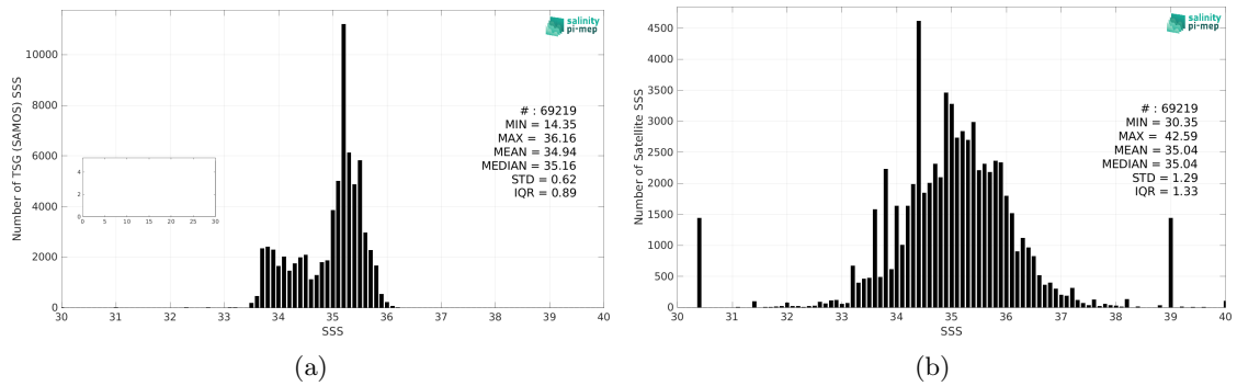
Figure 2: Histograms of SSS from TSG (SAMOS) (a) and SMAP SSS L2 v5 - 40 km (RSS) (b) considering all match-up pairs per bins of 0.1 over the South Pacific Ocean Pi-MEP region and for the full satellite product period.
