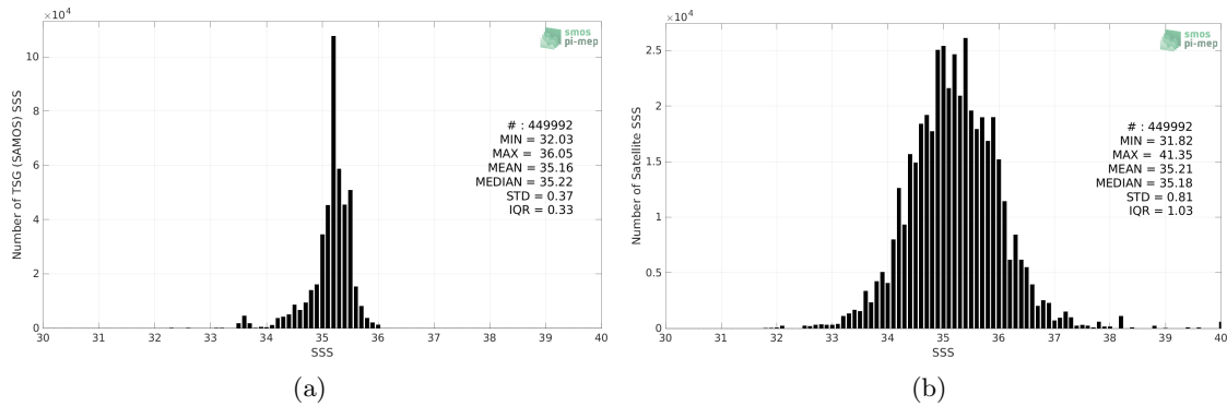
Figure 2: Histograms of SSS from TSG (SAMOS) (a) and SMAP SSS L2 v5 - 40 km (RSS) (b) considering all match-up pairs per bins of 0.1 over the South Pacific Ocean Pi-MEP region and for the full satellite product period.
