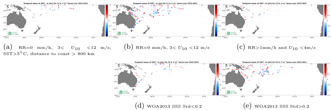
Figure 12: Temporal mean gridded over spatial boxes of size 1^\circ \times 1^\circ of \Delta SSS (SMAP SSS L2 v5 - 40 km (RSS) - TSG (SAMOS)) for 5 different subdatasets corresponding to:RR=0 mm/h, 3 < U_{10} < 12 m/s, SST >5^\circ\text{C} , distance to coast > 800 km (a), RR=0 mm/h, 3 < U_{10} < 12 m/s (b), RR >1 mm/h and U_{10} < 4 m/s (c), WOA2013 SSS Std <0.2 (d), WOA2013 SSS Std >0.2 (e).
