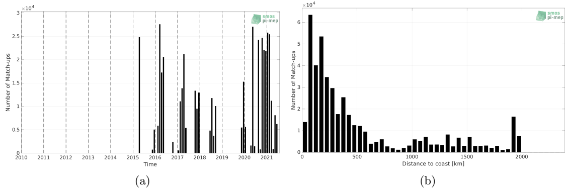
Figure 1: Number of match-ups between TSG (SAMOS) and SMAP SSS L2 v5 - 40 km (RSS) SSS as a function of time (a) and as function of the distance to coast (b) over the South Pacific Ocean Pi-MEP region and for the full satellite product period.
