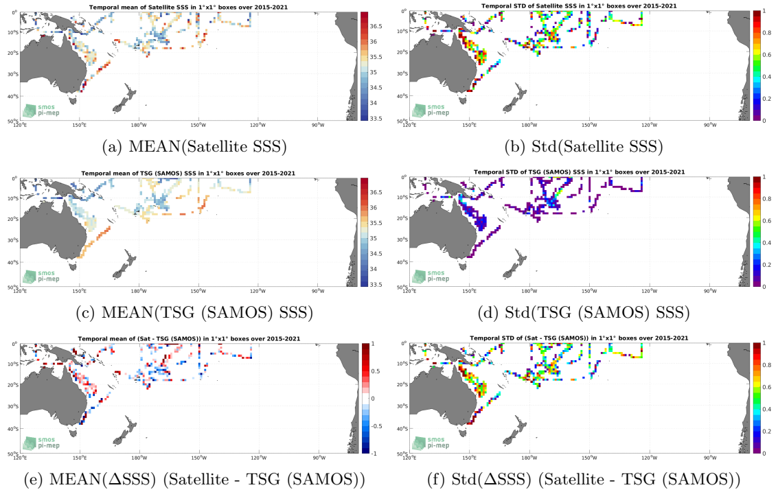
Figure 6: Temporal mean (left) and Std (right) of SSS from SMAP SSS L2 v5 - 40 km (RSS) (top), TSG (SAMOS) (middle), and of \Delta SSS (Satellite - TSG (SAMOS)). Only match-up pairs are used to generate these maps.
