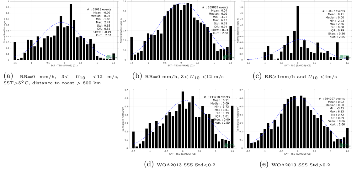
Figure 13: Normalized histogram of \Delta SSS (SMAP SSS L2 v5 - 40 km (RSS) - TSG (SAMOS)) for 5 different subdatasets corresponding to: RR=0 mm/h, 3 < U_{10} < 12 m/s, SST>5°C, distance to coast > 800 km (a), RR=0 mm/h, 3 < U_{10} < 12 m/s (b), RR>1mm/h and U_{10} < 4 m/s (c), WOA2013 SSS Std<0.2 (d), WOA2013 SSS Std>0.2 (e).
