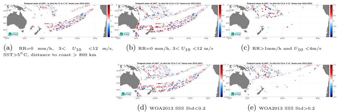
Figure 12: Temporal mean gridded over spatial boxes of size 1^\circ \times 1^\circ of \Delta\text{SSS} (SMAP SSS L2 v5 - 40 km (RSS) - TSG (LEGOS-DM)) for 5 different subdatasets corresponding to:RR=0 mm/h, 3 < U_{10} < 12 m/s, SST >5^\circ\text{C} , distance to coast > 800 km (a), RR=0 mm/h, 3 < U_{10} < 12 m/s (b), RR >1 mm/h and U_{10} < 4 m/s (c), WOA2013 SSS Std <0.2 (d), WOA2013 SSS Std >0.2 (e).
