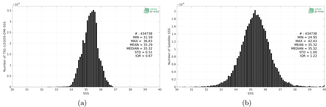
Figure 2: Histograms of SSS from TSG (LEGOS-DM) (a) and SMAP SSS L2 v5 - 40 km (RSS) (b) considering all match-up pairs per bins of 0.1 over the South Pacific Ocean Pi-MEP region and for the full satellite product period.
