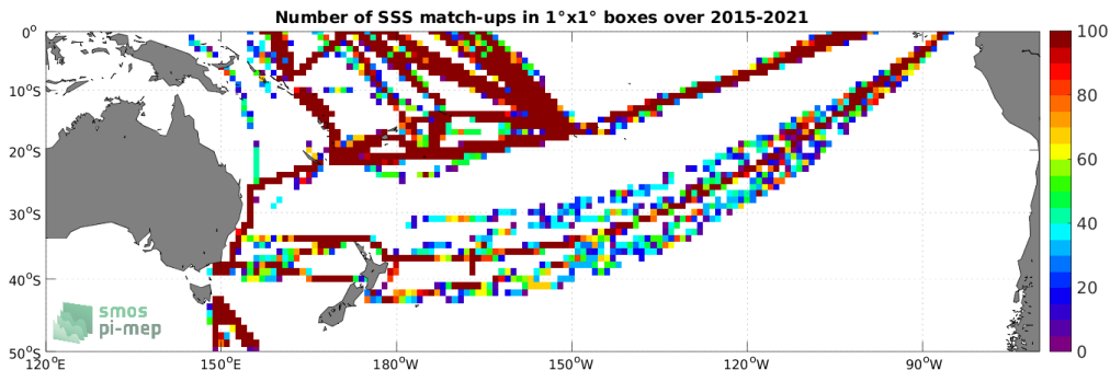
Figure 4: Number of SSS match-ups between TSG (LEGOS-DM) SSS and the SMAP SSS L2 v5 - 40 km (RSS) SSS product for the South Pacific Ocean Pi-MEP region over 1^\circ \times 1^\circ boxes and for the full satellite product period.
