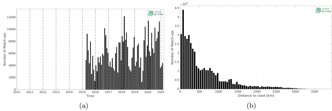
Figure 1: Number of match-ups between TSG (LEGOS-DM) and SMAP SSS L2 v5 - 40 km (RSS) SSS as a function of time (a) and as function of the distance to coast (b) over the South Pacific Ocean Pi-MEP region and for the full satellite product period.
