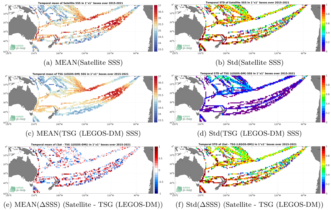
Figure 6: Temporal mean (left) and Std (right) of SSS from SMAP SSS L2 v5 - 40 km (RSS) (top), TSG (LEGOS-DM) (middle), and of \Delta SSS (Satellite - TSG (LEGOS-DM)). Only match-up pairs are used to generate these maps.
