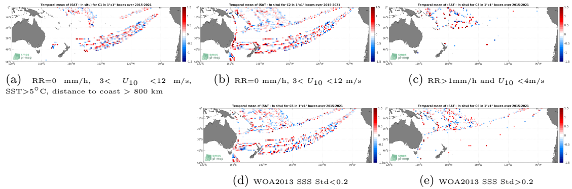
Figure 12: Temporal mean gridded over spatial boxes of size 1^\circ \times 1^\circ of \Delta SSS (SMAP SSS L2 v5 - 40 km (RSS) - TSG (LEGOS-DM)) for 5 different subdatasets corresponding to:RR=0 mm/h, 3 < U_{10} < 12 m/s, SST >5^\circ\text{C} , distance to coast > 800 km (a), RR=0 mm/h, 3 < U_{10} < 12 m/s (b), RR >1 mm/h and U_{10} < 4 m/s (c), WOA2013 SSS Std <0.2 (d), WOA2013 SSS Std >0.2 (e).
