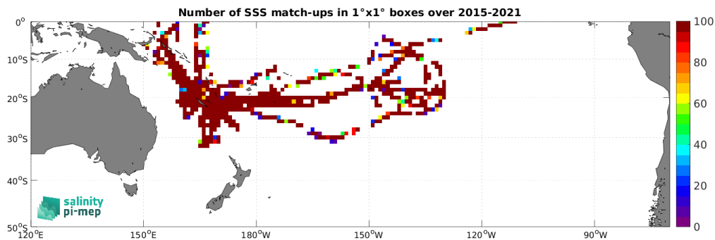
Figure 4: Number of SSS match-ups between TSG (GOSUD-Research-vessel) SSS and the SMAP SSS L2 v5 - 40 km (RSS) SSS product for the South Pacific Ocean Pi-MEP region over 1^\circ \times 1^\circ boxes and for the full satellite product period.
