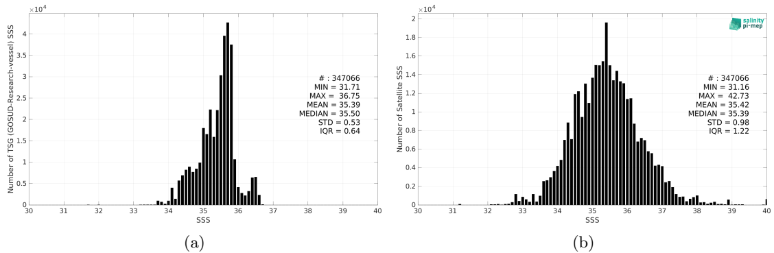
Figure 2: Histograms of SSS from TSG (GOSUD-Research-vessel) (a) and SMAP SSS L2 v5 - 40 km (RSS) (b) considering all match-up pairs per bins of 0.1 over the South Pacific Ocean Pi-MEP region and for the full satellite product period.
