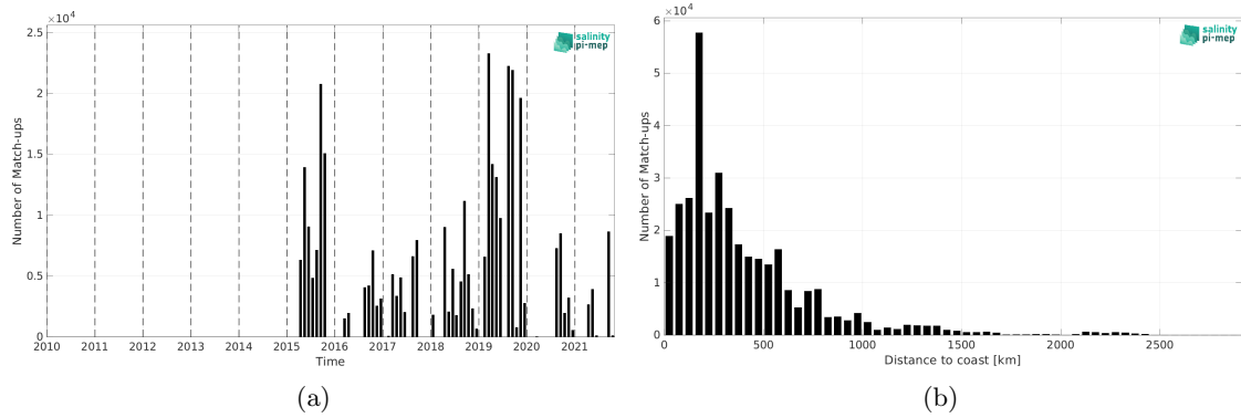
Figure 1: Number of match-ups between TSG (GOSUD-Research-vessel) and SMAP SSS L2 v5 - 40 km (RSS) SSS as a function of time (a) and as function of the distance to coast (b) over the South Pacific Ocean Pi-MEP region and for the full satellite product period.
