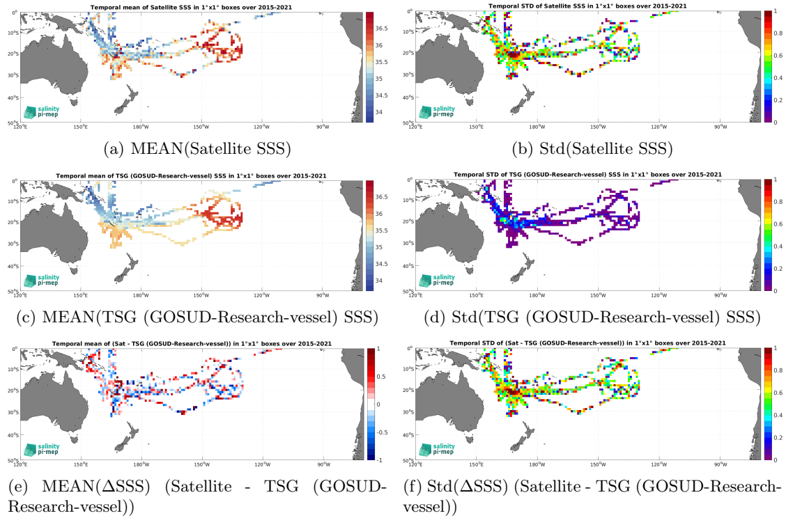
Figure 6: Temporal mean (left) and Std (right) of SSS from SMAP SSS L2 v5 - 40 km (RSS) (top), TSG (GOSUD-Research-vessel) (middle), and of \Delta SSS (Satellite - TSG (GOSUD-Research-vessel)). Only match-up pairs are used to generate these maps.
