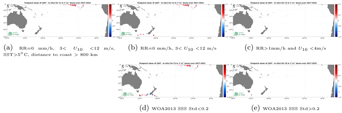
Figure 12: Temporal mean gridded over spatial boxes of size 1^\circ \times 1^\circ of \Delta SSS (SMAP SSS L2 v5 - 40 km (RSS) - Saldrone) for 5 different subdatasets corresponding to:RR=0 mm/h, 3 < U_{10} < 12 m/s, SST >5^\circ\text{C} , distance to coast > 800 km (a), RR=0 mm/h, 3 < U_{10} < 12 m/s (b), RR >1 mm/h and U_{10} < 4 m/s (c), WOA2013 SSS Std <0.2 (d), WOA2013 SSS Std >0.2 (e).
