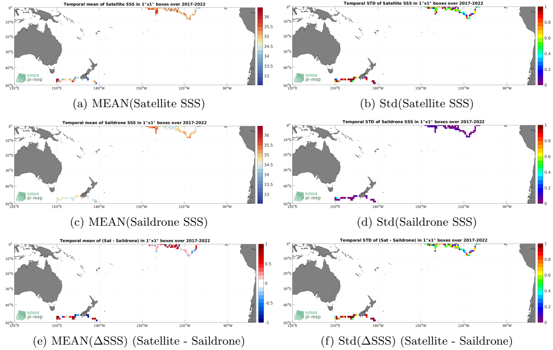
Figure 6: Temporal mean (left) and Std (right) of SSS from SMAP SSS L2 v5 - 40 km (RSS) (top), Saildrone (middle), and of \Delta SSS (Satellite - Saildrone). Only match-up pairs are used to generate these maps.
