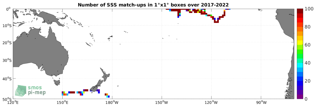
Figure 4: Number of SSS match-ups between Saildrone SSS and the SMAP SSS L2 v5 - 40 km (RSS) SSS product for the South Pacific Ocean Pi-MEP region over 1^\circ \times 1^\circ boxes and for the full satellite product period.
