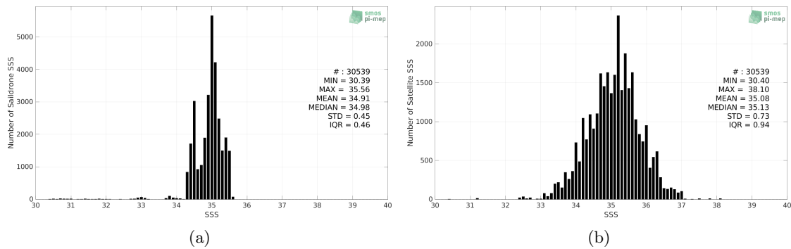
Figure 2: Histograms of SSS from Saildrone (a) and SMAP SSS L2 v5 - 40 km (RSS) (b) considering all match-up pairs per bins of 0.1 over the South Pacific Ocean Pi-MEP region and for the full satellite product period.
