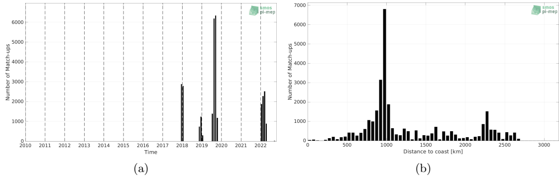
Figure 1: Number of match-ups between Saildrone and SMAP SSS L2 v5 - 40 km (RSS) SSS as a function of time (a) and as function of the distance to coast (b) over the South Pacific Ocean Pi-MEP region and for the full satellite product period.
