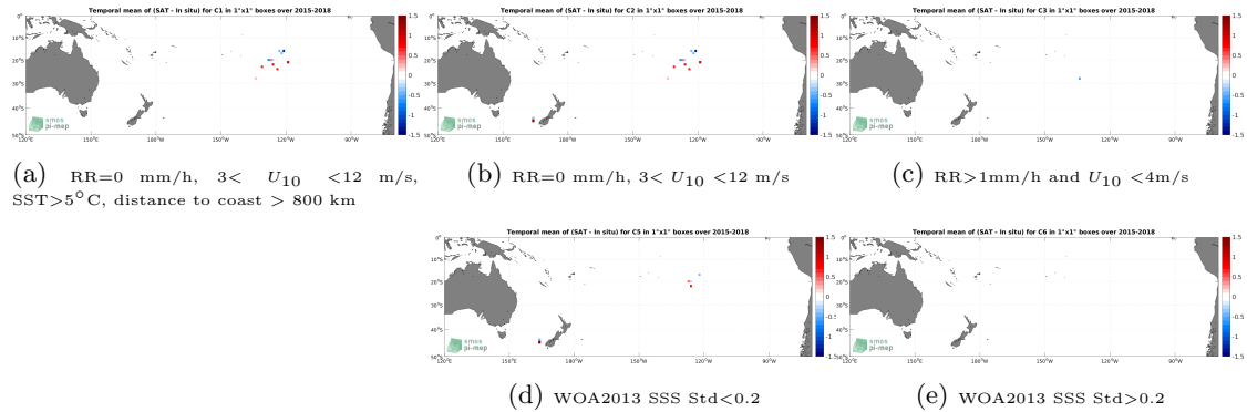
Figure 11: Temporal mean gridded over spatial boxes of size 1^\circ \times 1^\circ of \Delta SSS (SMAP SSS L2 v5 - 40 km (RSS) - Surface drifters) for 5 different subdatasets corresponding to:RR=0 mm/h, 3 < U_{10} < 12 m/s, SST >5^\circ\text{C} , distance to coast > 800 km (a), RR=0 mm/h, 3 < U_{10} < 12 m/s (b), RR >1 mm/h and U_{10} < 4 m/s (c), WOA2013 SSS Std <0.2 (d), WOA2013 SSS Std >0.2 (e).
