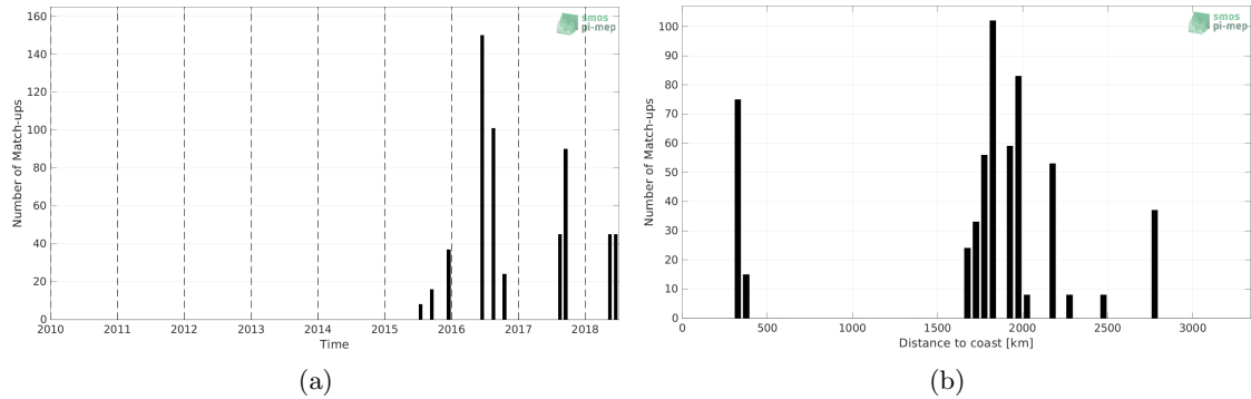
Figure 1: Number of match-ups between Surface drifters and SMAP SSS L2 v5 - 40 km (RSS) SSS as a function of time (a) and as function of the distance to coast (b) over the South Pacific Ocean Pi-MEP region and for the full satellite product period.
