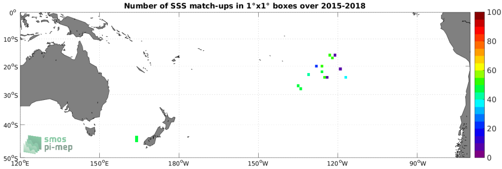
Figure 3: Number of SSS match-ups between Surface drifters SSS and the SMAP SSS L2 v5 - 40 km (RSS) SSS product for the South Pacific Ocean Pi-MEP region over 1^\circ \times 1^\circ boxes and for the full satellite product period.
