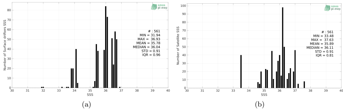
Figure 2: Histograms of SSS from Surface drifters (a) and SMAP SSS L2 v5 - 40 km (RSS) (b) considering all match-up pairs per bins of 0.1 over the South Pacific Ocean Pi-MEP region and for the full satellite product period.
