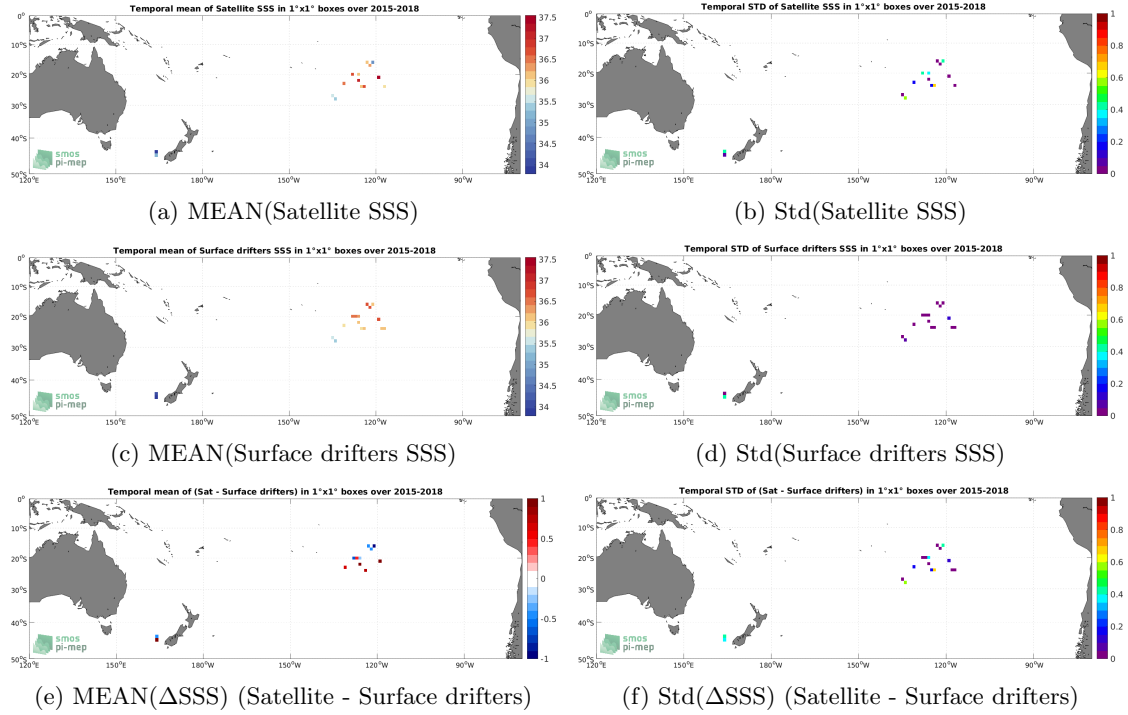
Figure 5: Temporal mean (left) and Std (right) of SSS from SMAP SSS L2 v5 - 40 km (RSS) (top), Surface drifters (middle), and of \Delta SSS (Satellite - Surface drifters). Only match-up pairs are used to generate these maps.
