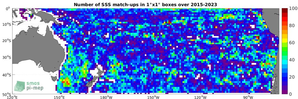
Figure 4: Number of SSS match-ups between Argo SSS and the SMAP SSS L2 v5 - 40 km (RSS) SSS product for the South Pacific Ocean Pi-MEP region over 1^\circ \times 1^\circ boxes and for the full satellite product period.
