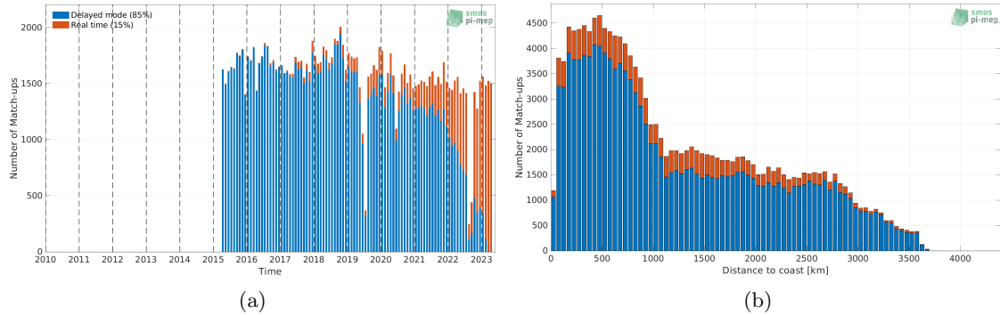
Figure 1: Number of match-ups between Argo and SMAP SSS L2 v5 - 40 km (RSS) SSS as a function of time (a) and as function of the distance to coast (b) over the South Pacific Ocean Pi-MEP region and for the full satellite product period.
