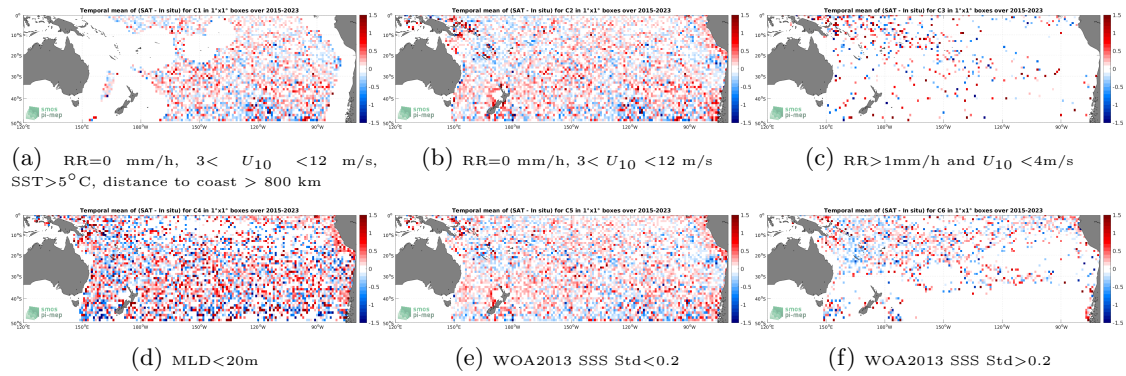
Figure 12: Temporal mean gridded over spatial boxes of size 1^\circ \times 1^\circ of \Delta SSS (SMAP SSS L2 v5 - 40 km (RSS) - Argo) for 6 different subdatasets corresponding to:RR=0 mm/h, 3 < U_{10} < 12 m/s, SST >5^\circ\text{C} , distance to coast > 800 km (a), RR=0 mm/h, 3 < U_{10} < 12 m/s (b), RR >1 mm/h and U_{10} < 4 m/s (c),MLD <20 m (d),WOA2013 SSS Std <0.2 (e),WOA2013 SSS Std >0.2 (f).
