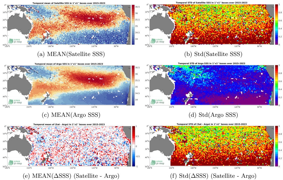
Figure 6: Temporal mean (left) and Std (right) of SSS from SMAP SSS L2 v5 - 40 km (RSS) (top), Argo (middle), and of \Delta SSS (Satellite - Argo). Only match-up pairs are used to generate these maps.
