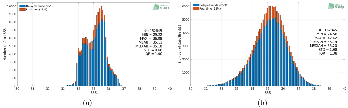
Figure 2: Histograms of SSS from Argo (a) and SMAP SSS L2 v5 - 40 km (RSS) (b) considering all match-up pairs per bins of 0.1 over the South Pacific Ocean Pi-MEP region and for the full satellite product period.
