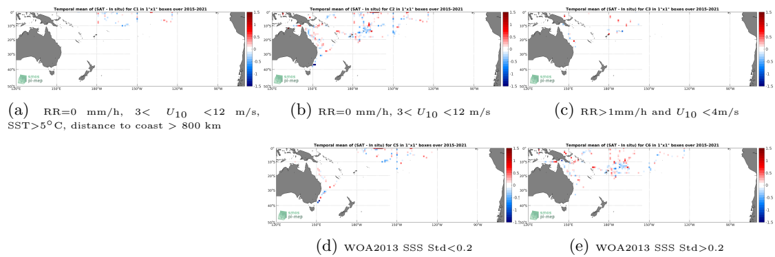
Figure 12: Temporal mean gridded over spatial boxes of size 1^\circ \times 1^\circ of \Delta\text{SSS} (SMAP SSS L2 v4 (RSS) - TSG (SAMOS)) for 5 different subdatasets corresponding to:RR=0 mm/h, 3 < U_{10} < 12 m/s, SST >5^\circ\text{C} , distance to coast > 800 km (a), RR=0 mm/h, 3 < U_{10} < 12 m/s (b), RR >1 mm/h and U_{10} < 4 m/s (c), WOA2013 SSS Std <0.2 (d), WOA2013 SSS Std >0.2 (e).
