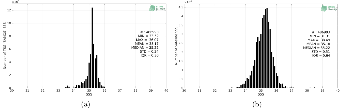
Figure 2: Histograms of SSS from TSG (SAMOS) (a) and SMAP SSS L2 v4 (RSS) (b) considering all match-up pairs per bins of 0.1 over the South Pacific Ocean Pi-MEP region and for the full satellite product period.
