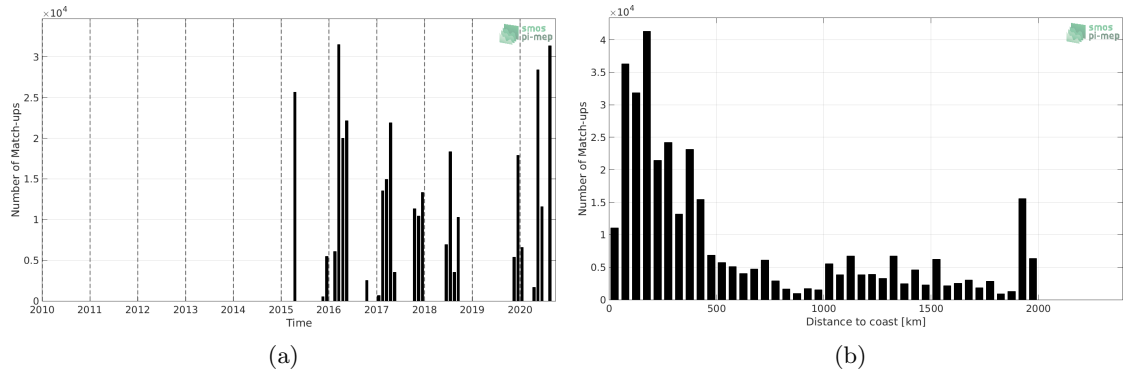
Figure 1: Number of match-ups between TSG (SAMOS) and SMAP SSS L2 v4 (RSS) SSS as a function of time (a) and as function of the distance to coast (b) over the South Pacific Ocean Pi-MEP region and for the full satellite product period.
