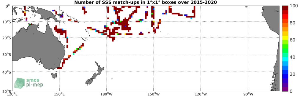
Figure 4: Number of SSS match-ups between TSG (SAMOS) SSS and the SMAP SSS L2 v4 (RSS) SSS product for the South Pacific Ocean Pi-MEP region over 1^\circ \times 1^\circ boxes and for the full satellite product period.
