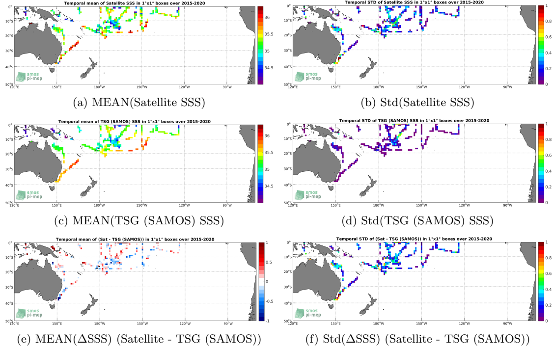
Figure 6: Temporal mean (left) and Std (right) of SSS from SMAP SSS L2 v4 (RSS) (top), TSG (SAMOS) (middle), and of \Delta SSS (Satellite - TSG (SAMOS)). Only match-up pairs are used to generate these maps.
