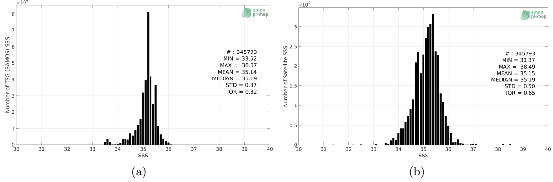
Figure 2: Histograms of SSS from TSG (SAMOS) (a) and SMAP SSS L2 v4 (RSS) (b) considering all match-up pairs per bins of 0.1 over the South Pacific Ocean Pi-MEP region and for the full satellite product period.
