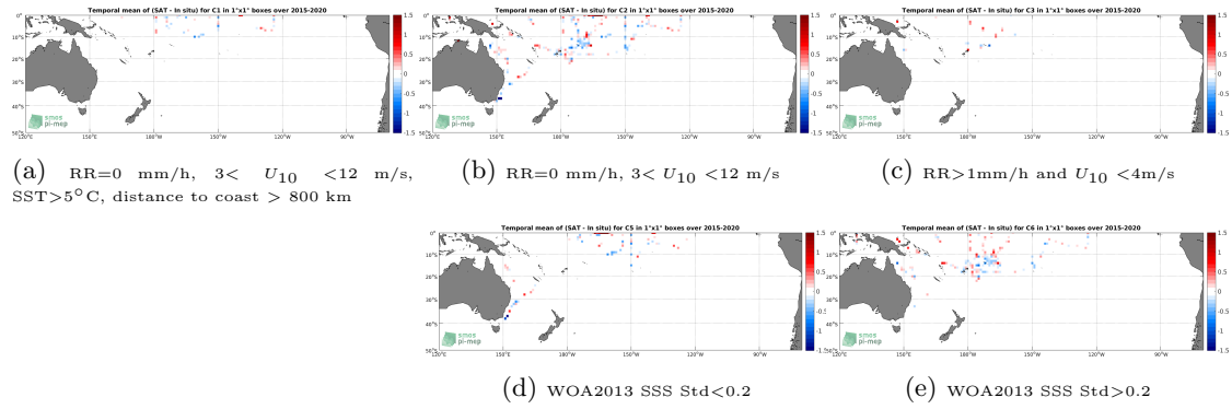
Figure 12: Temporal mean gridded over spatial boxes of size 1^\circ \times 1^\circ of \Delta SSS (SMAP SSS L2 v4 (RSS) - TSG (SAMOS)) for 5 different subdatasets corresponding to: RR=0 mm/h, 3 < U_{10} < 12 m/s, SST > 5^\circ\text{C} , distance to coast > 800 km (a), RR=0 mm/h, 3 < U_{10} < 12 m/s (b), RR > 1 mm/h and U_{10} < 4 m/s (c), WOA2013 SSS Std < 0.2 (d), WOA2013 SSS Std > 0.2 (e).
