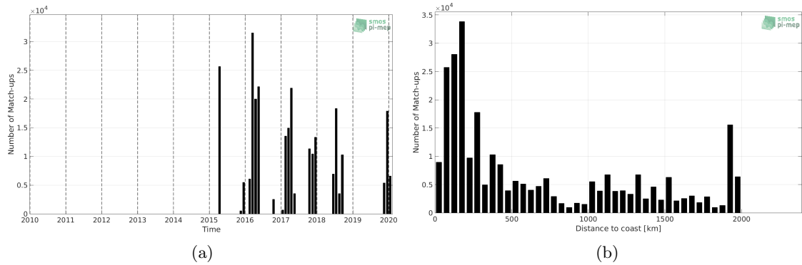
Figure 1: Number of match-ups between TSG-SAMOS and SMAP-L2-RSS-V4 SSS as a function of time (a) and as function of the distance to coast (b) over the South Pacific Ocean Pi-MEP region and for the full satellite product period.
