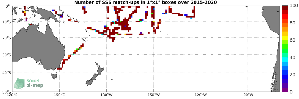
Figure 4: Number of SSS match-ups between TSG-SAMOS SSS and the SMAP-L2-RSS-V4 SSS product for the South Pacific Ocean Pi-MEP region over 1^\circ \times 1^\circ boxes and for the full satellite product period.
