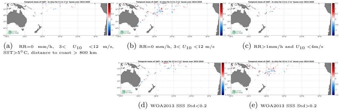
Figure 12: Temporal mean gridded over spatial boxes of size 1^\circ \times 1^\circ of \Delta SSS (SMAP-L2-RSS-V4 - TSG-SAMOS) for 5 different subdatasets corresponding to: RR=0 mm/h, 3 < U_{10} < 12 m/s, SST > 5^\circ\text{C} , distance to coast > 800 km (a), RR=0 mm/h, 3 < U_{10} < 12 m/s (b), RR > 1 mm/h and U_{10} < 4 m/s (c), WOA2013 SSS Std < 0.2 (d), WOA2013 SSS Std > 0.2 (e).
