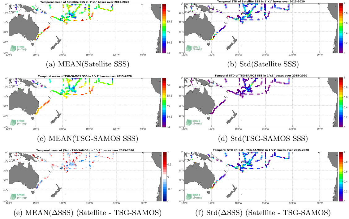
Figure 6: Temporal mean (left) and Std (right) of SSS from SMAP-L2-RSS-V4 (top), TSG-SAMOS (middle), and of \Delta SSS (Satellite - TSG-SAMOS). Only match-up pairs are used to generate these maps.
