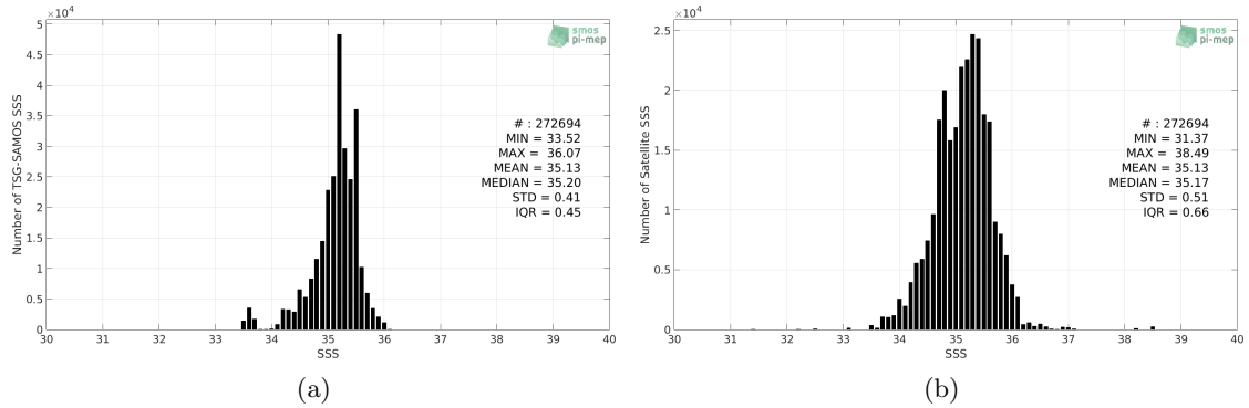
Figure 2: Histograms of SSS from TSG-SAMOS (a) and SMAP-L2-RSS-V4 (b) considering all match-up pairs per bins of 0.1 over the South Pacific Ocean Pi-MEP region and for the full satellite product period.
