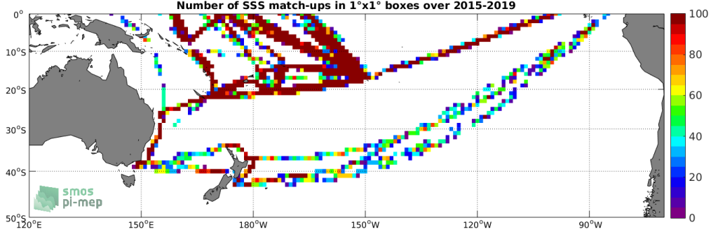
Figure 4: Number of SSS match-ups between TSG (LEGOS-DM) SSS and the SMAP SSS L2 v4 (RSS) SSS product for the South Pacific Ocean Pi-MEP region over 1^\circ \times 1^\circ boxes and for the full satellite product period.
