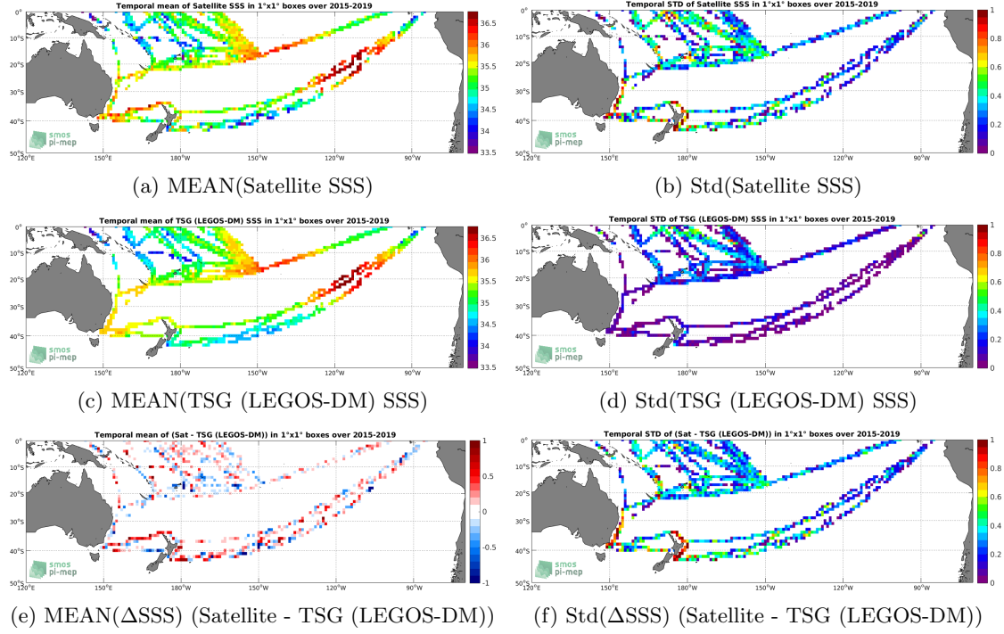
Figure 6: Temporal mean (left) and Std (right) of SSS from SMAP SSS L2 v4 (RSS) (top), TSG (LEGOS-DM) (middle), and of \Delta SSS (Satellite - TSG (LEGOS-DM)). Only match-up pairs are used to generate these maps.
