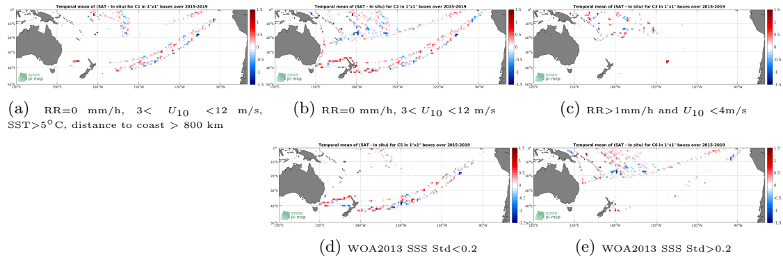
Figure 12: Temporal mean gridded over spatial boxes of size 1^\circ \times 1^\circ of \Delta SSS (SMAP SSS L2 v4 (RSS) - TSG (LEGOS-DM)) for 5 different subdatasets corresponding to: RR=0 mm/h, 3 < U_{10} < 12 m/s, SST > 5^\circ C , distance to coast > 800 km (a), RR=0 mm/h, 3 < U_{10} < 12 m/s (b), RR > 1 mm/h and U_{10} < 4 m/s (c), WOA2013 SSS Std < 0.2 (d), WOA2013 SSS Std > 0.2 (e).
