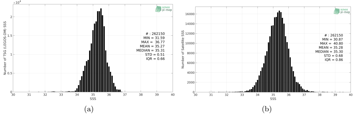
Figure 2: Histograms of SSS from TSG (LEGOS-DM) (a) and SMAP SSS L2 v4 (RSS) (b) considering all match-up pairs per bins of 0.1 over the South Pacific Ocean Pi-MEP region and for the full satellite product period.
