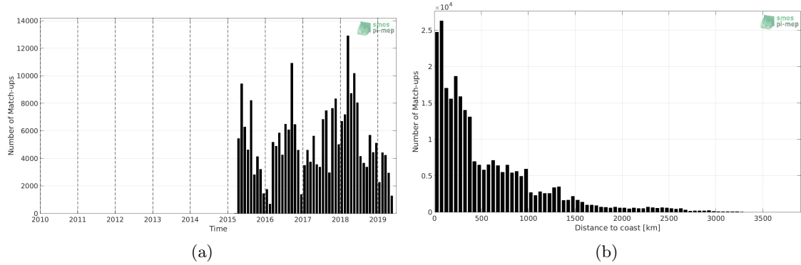
Figure 1: Number of match-ups between TSG (LEGOS-DM) and SMAP SSS L2 v4 (RSS) SSS as a function of time (a) and as function of the distance to coast (b) over the South Pacific Ocean Pi-MEP region and for the full satellite product period.
