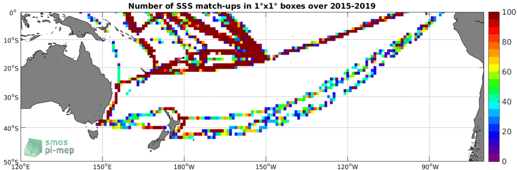
Figure 4: Number of SSS match-ups between TSG-LEGOS-DM SSS and the SMAP-L2-RSS-V4 SSS product for the South Pacific Ocean Pi-MEP region over 1^\circ \times 1^\circ boxes and for the full satellite product period.
