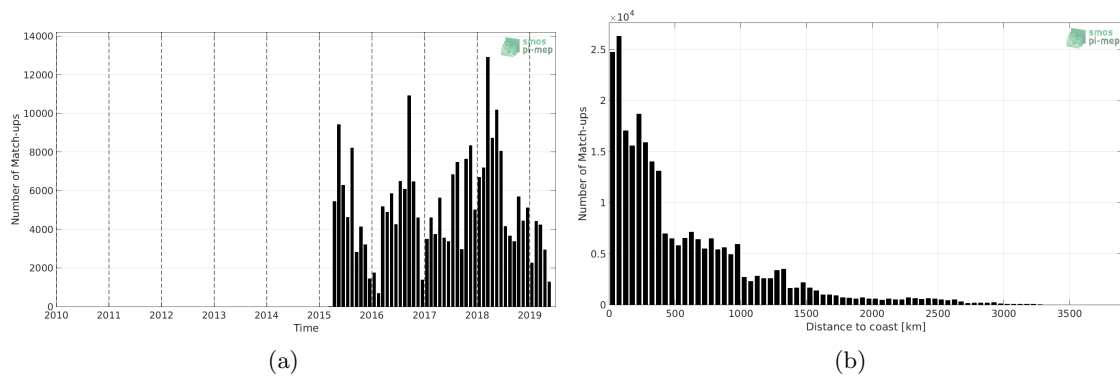
Figure 1: Number of match-ups between TSG-LEGOS-DM and SMAP-L2-RSS-V4 SSS as a function of time (a) and as function of the distance to coast (b) over the South Pacific Ocean Pi-MEP region and for the full satellite product period.
