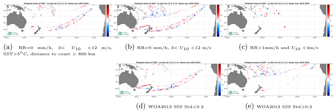
Figure 12: Temporal mean gridded over spatial boxes of size 1^\circ \times 1^\circ of \Delta SSS (SMAP-L2-RSS-V4 - TSG-LEGOS-DM) for 5 different subdatasets corresponding to:RR=0 mm/h, 3 < U_{10} < 12 m/s, SST >5^\circ C, distance to coast > 800 km (a), RR=0 mm/h, 3 < U_{10} < 12 m/s (b), RR >1 mm/h and U_{10} < 4 m/s (c), WOA2013 SSS Std <0.2 (d), WOA2013 SSS Std >0.2 (e).
