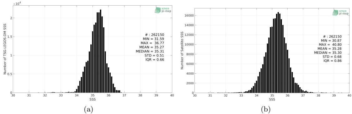
Figure 2: Histograms of SSS from TSG-LEGOS-DM (a) and SMAP-L2-RSS-V4 (b) considering all match-up pairs per bins of 0.1 over the South Pacific Ocean Pi-MEP region and for the full satellite product period.
