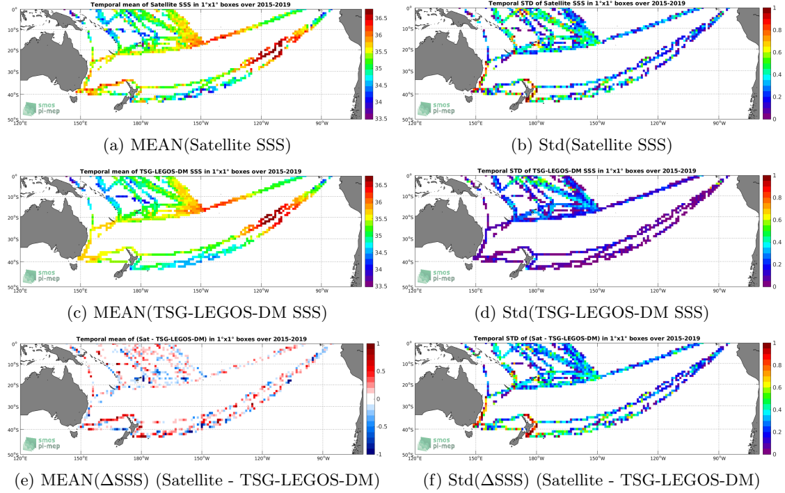
Figure 6: Temporal mean (left) and Std (right) of SSS from SMAP-L2-RSS-V4 (top), TSG-LEGOS-DM (middle), and of \Delta SSS (Satellite - TSG-LEGOS-DM). Only match-up pairs are used to generate these maps.
