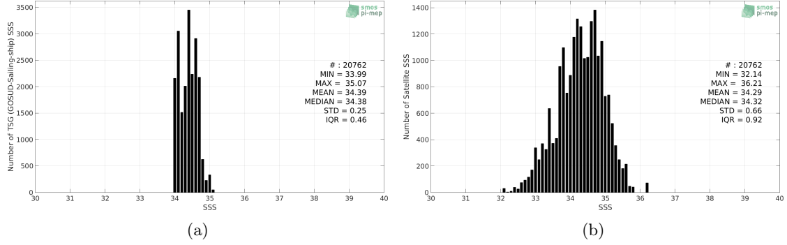
Figure 2: Histograms of SSS from TSG (GOSUD-Sailing-ship) (a) and SMAP SSS L2 v4 (RSS) (b) considering all match-up pairs per bins of 0.1 over the South Pacific Ocean Pi-MEP region and for the full satellite product period.
