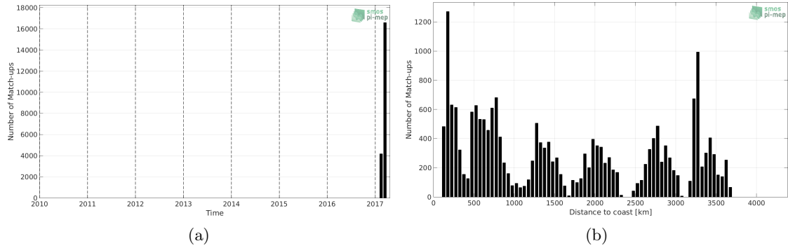
Figure 1: Number of match-ups between TSG (GOSUD-Sailing-ship) and SMAP SSS L2 v4 (RSS) SSS as a function of time (a) and as function of the distance to coast (b) over the South Pacific Ocean Pi-MEP region and for the full satellite product period.
