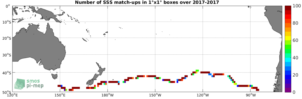
Figure 4: Number of SSS match-ups between TSG (GOSUD-Sailing-ship) SSS and the SMAP SSS L2 v4 (RSS) SSS product for the South Pacific Ocean Pi-MEP region over 1^\circ \times 1^\circ boxes and for the full satellite product period.
