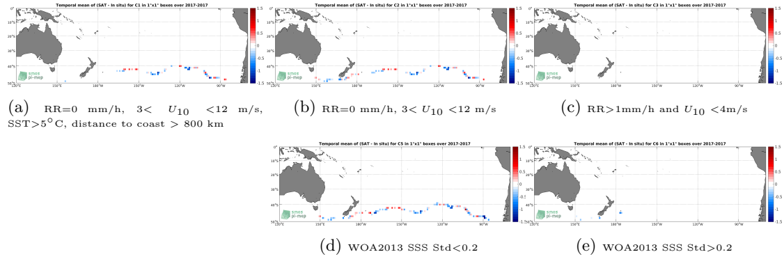
Figure 12: Temporal mean gridded over spatial boxes of size 1^\circ \times 1^\circ of \Delta SSS (SMAP SSS L2 v4 (RSS) - TSG (GOSUD-Sailing-ship)) for 5 different subdatasets corresponding to: RR=0 mm/h, 3 < U_{10} < 12 m/s, SST >5^\circ C, distance to coast > 800 km (a), RR=0 mm/h, 3 < U_{10} < 12 m/s (b), RR>1 mm/h and U_{10} < 4 m/s (c), WOA2013 SSS Std <0.2 (d), WOA2013 SSS Std >0.2 (e).
