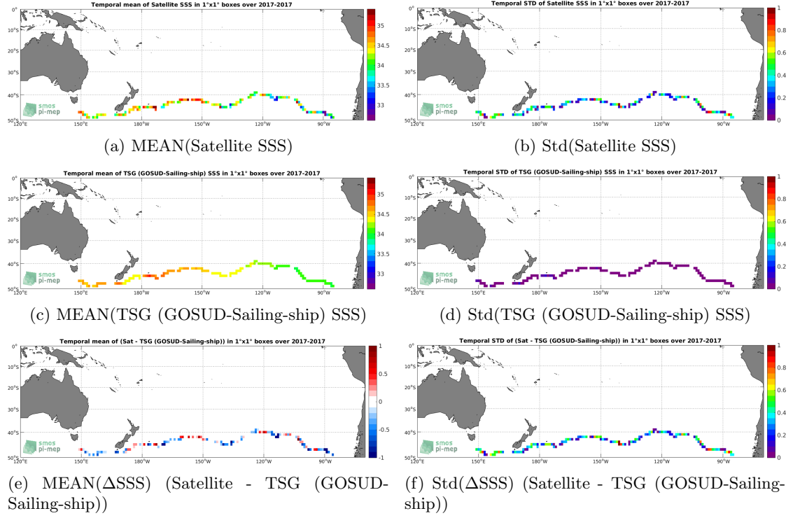
Figure 6: Temporal mean (left) and Std (right) of SSS from SMAP SSS L2 v4 (RSS) (top), TSG (GOSUD-Sailing-ship) (middle), and of \Delta SSS (Satellite - TSG (GOSUD-Sailing-ship)). Only match-up pairs are used to generate these maps.
