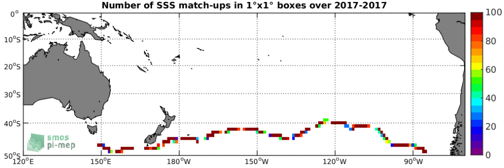
Figure 4: Number of SSS match-ups between TSG-GOSUD-Sailing-ship SSS and the SMAP-L2-RSS-V4 SSS product for the South Pacific Ocean Pi-MEP region over 1^\circ \times 1^\circ boxes and for the full satellite product period.
