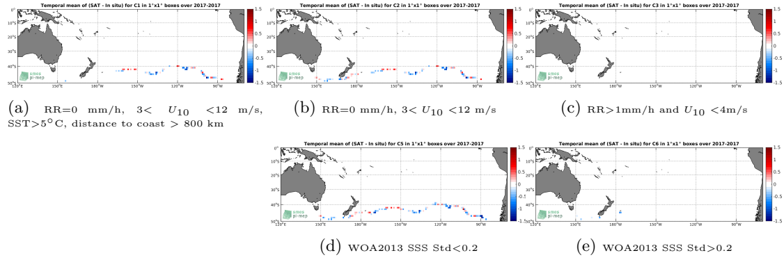
Figure 12: Temporal mean gridded over spatial boxes of size 1^\circ \times 1^\circ of \Delta SSS (SMAP-L2-RSS-V4 - TSG-GOSUD-Sailing-ship) for 5 different subdatasets corresponding to: RR=0 mm/h, 3 < U_{10} < 12 m/s, SST > 5^\circ C , distance to coast > 800 km (a), RR=0 mm/h, 3 < U_{10} < 12 m/s (b), RR > 1 mm/h and U_{10} < 4 m/s (c), WOA2013 SSS Std < 0.2 (d), WOA2013 SSS Std > 0.2 (e).
