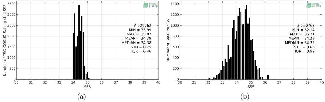
Figure 2: Histograms of SSS from TSG-GOSUD-Sailing-ship (a) and SMAP-L2-RSS-V4 (b) considering all match-up pairs per bins of 0.1 over the South Pacific Ocean Pi-MEP region and for the full satellite product period.
