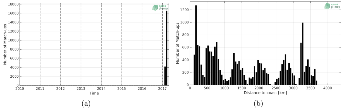
Figure 1: Number of match-ups between TSG-GOSUD-Sailing-ship and SMAP-L2-RSS-V4 SSS as a function of time (a) and as function of the distance to coast (b) over the South Pacific Ocean Pi-MEP region and for the full satellite product period.
