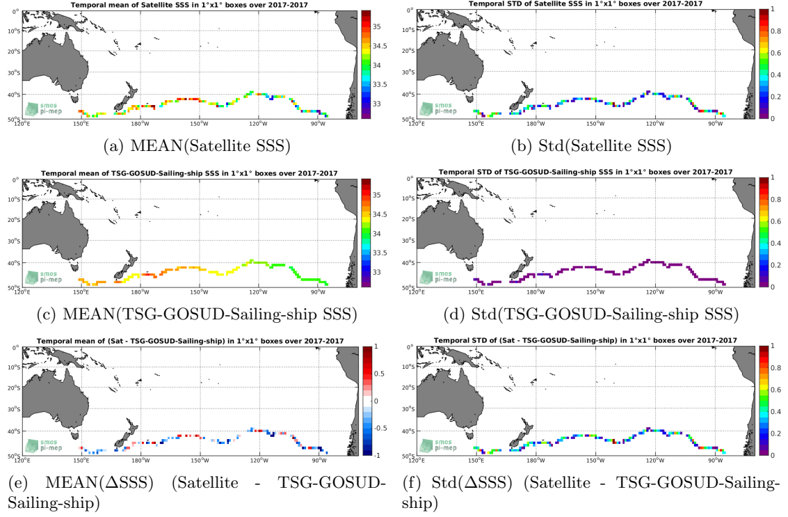
Figure 6: Temporal mean (left) and Std (right) of SSS from SMAP-L2-RSS-V4 (top), TSG-GOSUD-Sailing-ship (middle), and of \Delta SSS (Satellite - TSG-GOSUD-Sailing-ship). Only match-up pairs are used to generate these maps.
