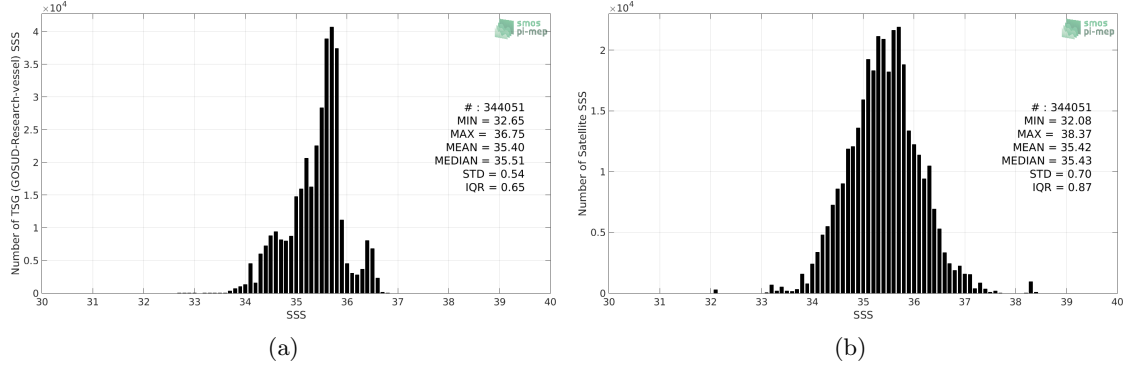
Figure 2: Histograms of SSS from TSG (GOSUD-Research-vessel) (a) and SMAP SSS L2 v4 (RSS) (b) considering all match-up pairs per bins of 0.1 over the South Pacific Ocean Pi-MEP region and for the full satellite product period.
