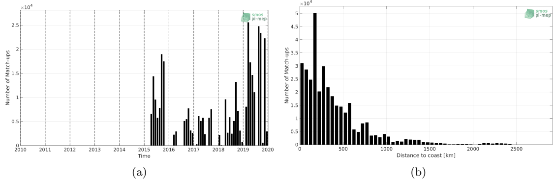
Figure 1: Number of match-ups between TSG (GOSUD-Research-vessel) and SMAP SSS L2 v4 (RSS) SSS as a function of time (a) and as function of the distance to coast (b) over the South Pacific Ocean Pi-MEP region and for the full satellite product period.
