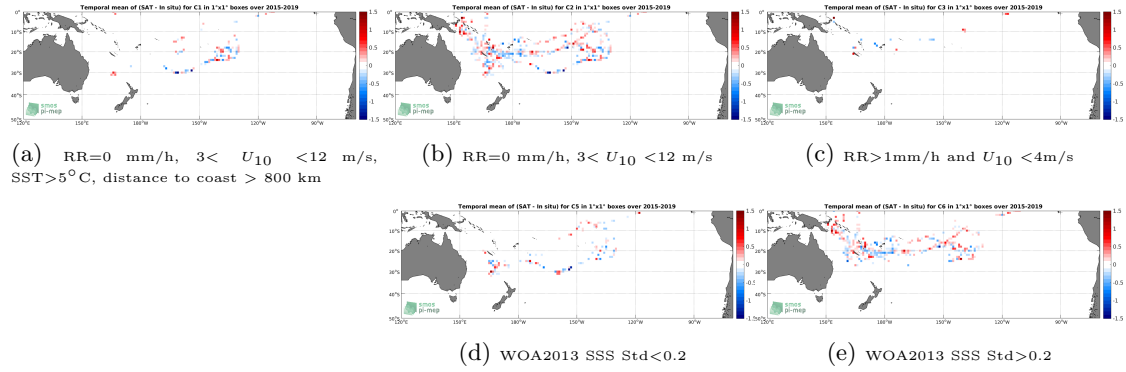
Figure 12: Temporal mean gridded over spatial boxes of size 1^\circ \times 1^\circ of \Delta SSS (SMAP SSS L2 v4 (RSS) - TSG (GOSUD-Research-vessel)) for 5 different subdatasets corresponding to: RR=0 mm/h, 3 < U_{10} < 12 m/s, SST > 5^\circ\text{C} , distance to coast > 800 km (a), RR=0 mm/h, 3 < U_{10} < 12 m/s (b), RR > 1 mm/h and U_{10} < 4 m/s (c), WOA2013 SSS Std < 0.2 (d), WOA2013 SSS Std > 0.2 (e).
