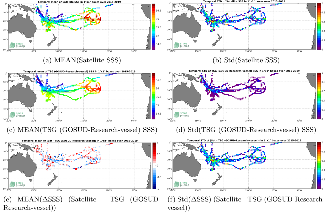
Figure 6: Temporal mean (left) and Std (right) of SSS from SMAP SSS L2 v4 (RSS) (top), TSG (GOSUD-Research-vessel) (middle), and of \Delta SSS (Satellite - TSG (GOSUD-Research-vessel)). Only match-up pairs are used to generate these maps.
