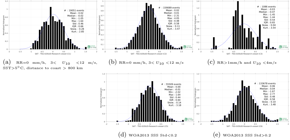
Figure 13: Normalized histogram of \Delta\text{SSS} (SMAP-L2-RSS-V4 - TSG-GOSUD-Research-vessel) for 5 different subdatasets corresponding to: RR=0 mm/h, 3 < U_{10} < 12 m/s, SST > 5^\circ\text{C} , distance to coast > 800 km (a), RR=0 mm/h, 3 < U_{10} < 12 m/s (b), RR > 1 mm/h and U_{10} < 4 m/s (c), WOA2013 SSS Std < 0.2 (d), WOA2013 SSS Std > 0.2 (e).
