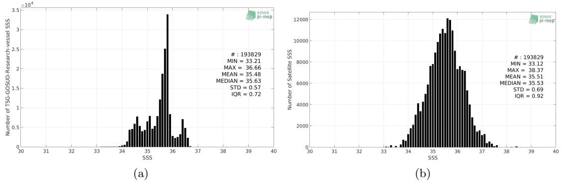
Figure 2: Histograms of SSS from TSG-GOSUD-Research-vessel (a) and SMAP-L2-RSS-V4 (b) considering all match-up pairs per bins of 0.1 over the South Pacific Ocean Pi-MEP region and for the full satellite product period.
