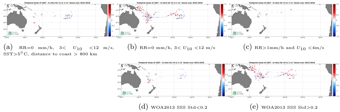
Figure 12: Temporal mean gridded over spatial boxes of size 1^\circ \times 1^\circ of \Delta SSS (SMAP-L2-RSS-V4 - TSG-GOSUD-Research-vessel) for 5 different subdatasets corresponding to: RR=0 mm/h, 3 < U_{10} < 12 m/s, SST > 5^\circ C , distance to coast > 800 km (a), RR=0 mm/h, 3 < U_{10} < 12 m/s (b), RR > 1 mm/h and U_{10} < 4 m/s (c), WOA2013 SSS Std < 0.2 (d), WOA2013 SSS Std > 0.2 (e).
