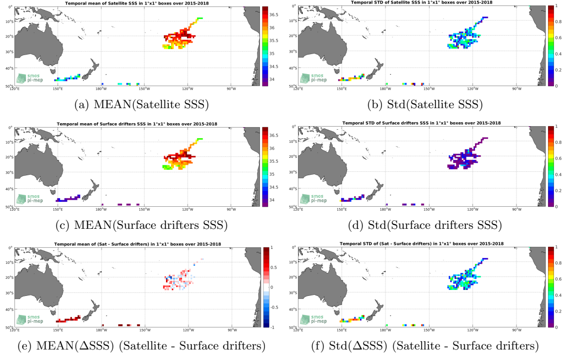
Figure 5: Temporal mean (left) and Std (right) of SSS from SMAP SSS L2 v4 (RSS) (top), Surface drifters (middle), and of \Delta SSS (Satellite - Surface drifters). Only match-up pairs are used to generate these maps.
