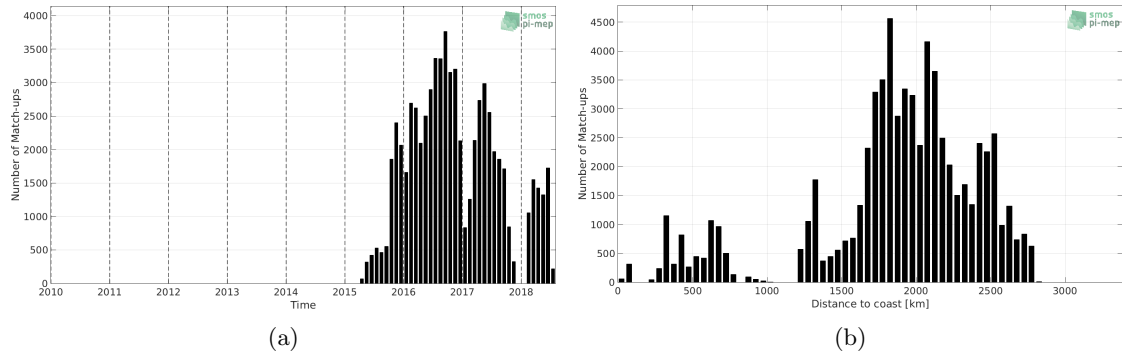
Figure 1: Number of match-ups between Surface drifters and SMAP SSS L2 v4 (RSS) SSS as a function of time (a) and as function of the distance to coast (b) over the South Pacific Ocean Pi-MEP region and for the full satellite product period.
