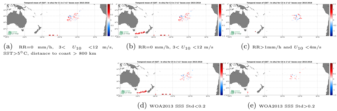
Figure 11: Temporal mean gridded over spatial boxes of size 1^\circ \times 1^\circ of \Delta SSS (SMAP SSS L2 v4 (RSS) - Surface drifters) for 5 different subdatasets corresponding to: RR=0 mm/h, 3 < U_{10} < 12 m/s, SST > 5^\circ C , distance to coast > 800 km (a), RR=0 mm/h, 3 < U_{10} < 12 m/s (b), RR > 1 mm/h and U_{10} < 4 m/s (c), WOA2013 SSS Std < 0.2 (d), WOA2013 SSS Std > 0.2 (e).
