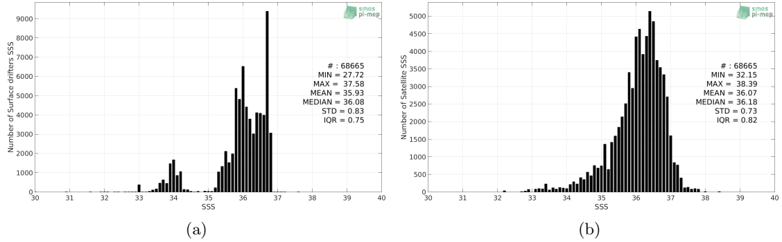
Figure 2: Histograms of SSS from Surface drifters (a) and SMAP SSS L2 v4 (RSS) (b) considering all match-up pairs per bins of 0.1 over the South Pacific Ocean Pi-MEP region and for the full satellite product period.
