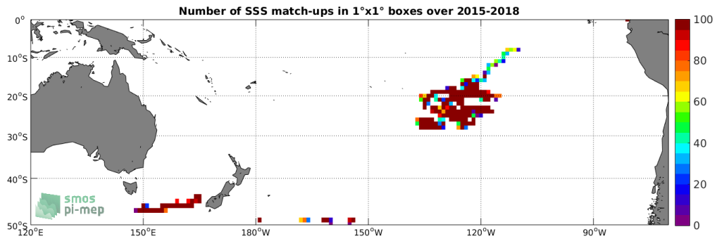
Figure 3: Number of SSS match-ups between Surface drifters SSS and the SMAP SSS L2 v4 (RSS) SSS product for the South Pacific Ocean Pi-MEP region over 1°x1° boxes and for the full satellite product period.
