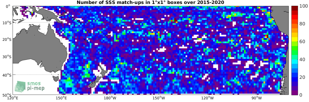
Figure 4: Number of SSS match-ups between Argo SSS and the SMAP SSS L2 v4 (RSS) SSS product for the South Pacific Ocean Pi-MEP region over 1^\circ \times 1^\circ boxes and for the full satellite product period.
