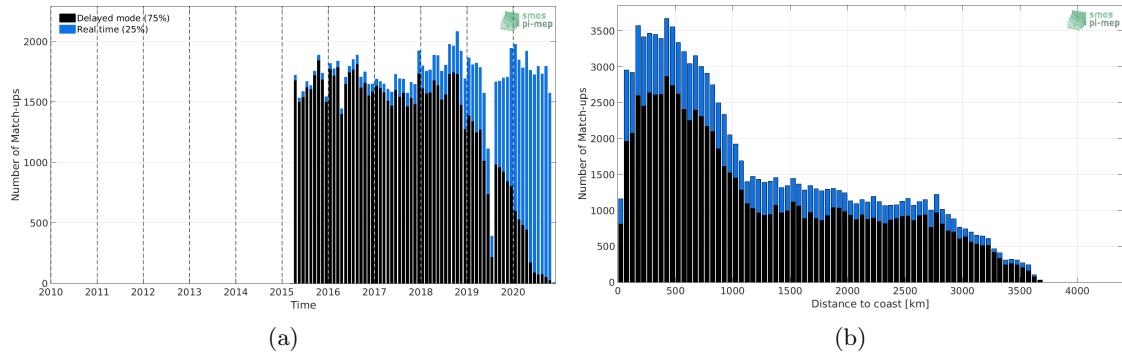
Figure 1: Number of match-ups between Argo and SMAP SSS L2 v4 (RSS) SSS as a function of time (a) and as function of the distance to coast (b) over the South Pacific Ocean Pi-MEP region and for the full satellite product period.
