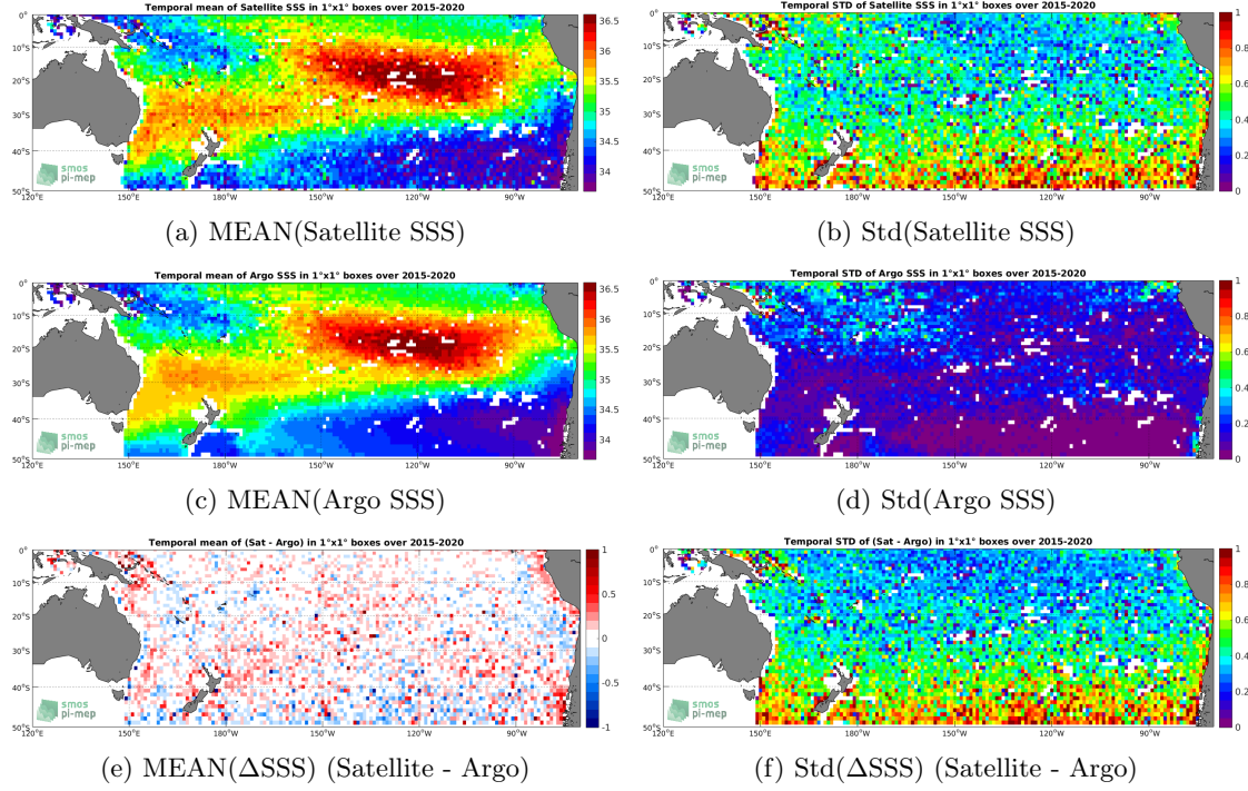
Figure 6: Temporal mean (left) and Std (right) of SSS from SMAP SSS L2 v4 (RSS) (top), Argo (middle), and of \Delta SSS (Satellite - Argo). Only match-up pairs are used to generate these maps.
