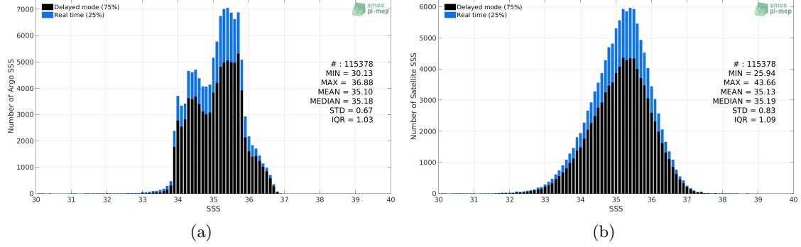
Figure 2: Histograms of SSS from Argo (a) and SMAP SSS L2 v4 (RSS) (b) considering all match-up pairs per bins of 0.1 over the South Pacific Ocean Pi-MEP region and for the full satellite product period.
