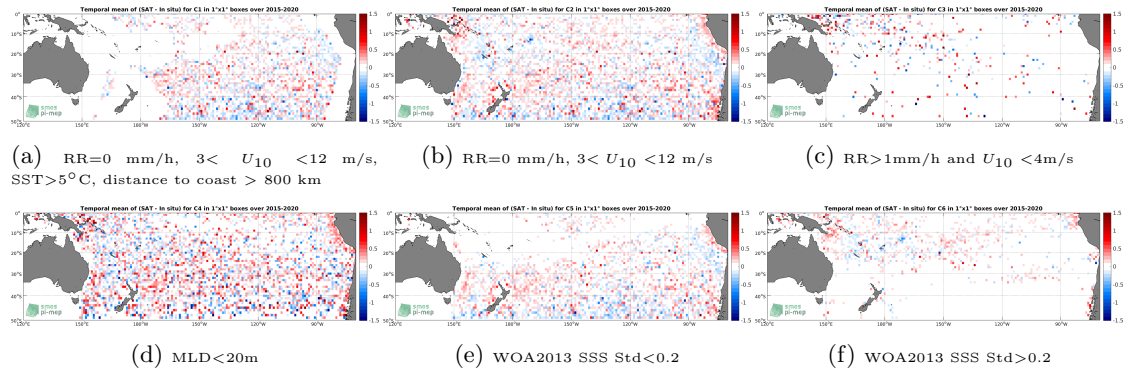
Figure 12: Temporal mean gridded over spatial boxes of size 1^\circ \times 1^\circ of \Delta SSS (SMAP SSS L2 v4 (RSS) - Argo) for 6 different subdatasets corresponding to: RR=0 mm/h, 3 < U_{10} < 12 m/s, SST >5^\circ C, distance to coast > 800 km (a), RR=0 mm/h, 3 < U_{10} < 12 m/s (b), RR>1 mm/h and U_{10} < 4 m/s (c), MLD <20 m (d), WOA2013 SSS Std <0.2 (e), WOA2013 SSS Std >0.2 (f).
