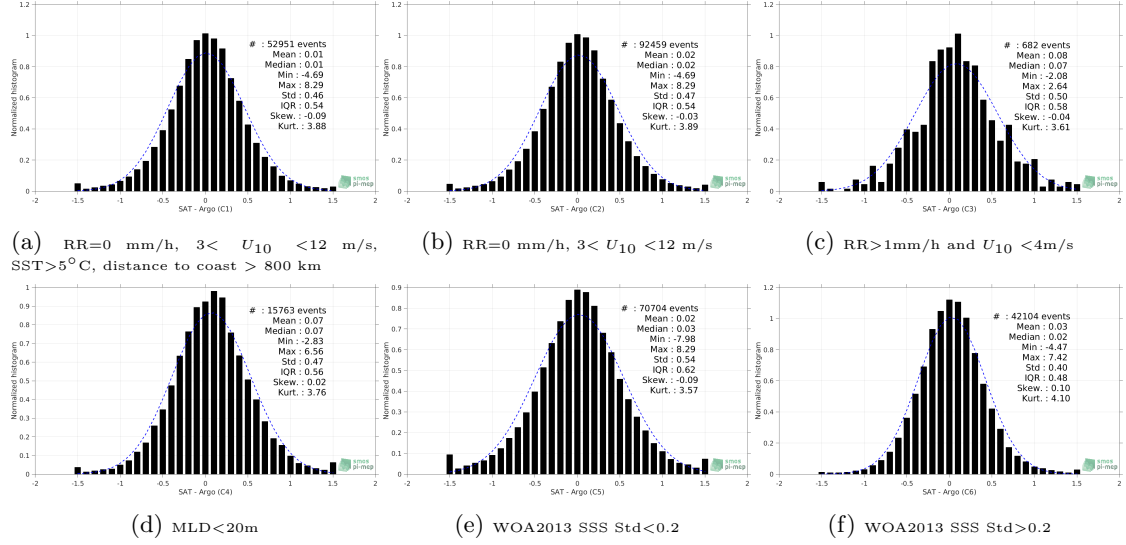
Figure 13: Normalized histogram of \Delta\text{SSS} (SMAP SSS L2 v4 (RSS) - Argo) for 6 different subdatasets corresponding to: RR=0 mm/h, 3 < U_{10} < 12 m/s, SST>5°C, distance to coast > 800 km (a), RR=0 mm/h, 3 < U_{10} < 12 m/s (b), RR>1mm/h and U_{10} < 4 m/s (c), MLD<20m (d), WOA2013 SSS Std<0.2 (e), WOA2013 SSS Std>0.2 (f).
