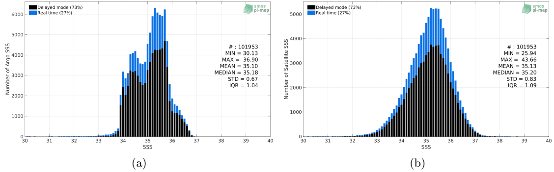
Figure 2: Histograms of SSS from Argo (a) and SMAP-L2-RSS-V4 (b) considering all match-up pairs per bins of 0.1 over the South Pacific Ocean Pi-MEP region and for the full satellite product period.
