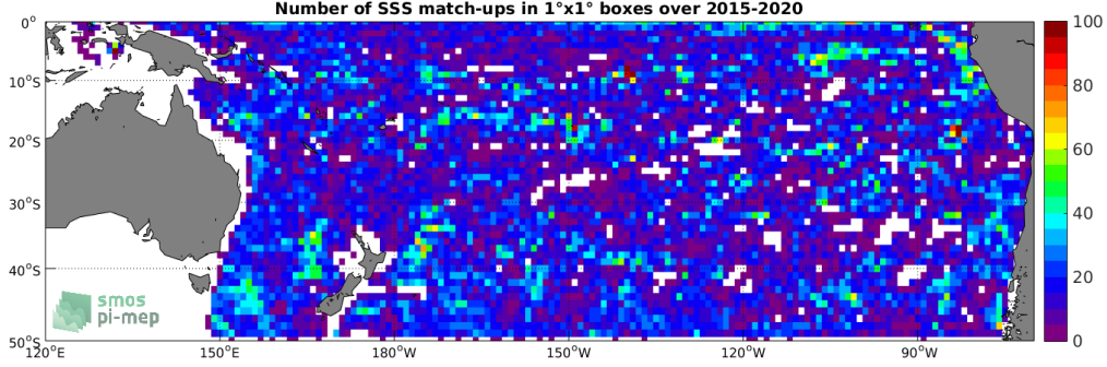
Figure 4: Number of SSS match-ups between Argo SSS and the SMAP-L2-RSS-V4 SSS product for the South Pacific Ocean Pi-MEP region over 1°x1° boxes and for the full satellite product period.
