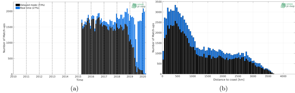
Figure 1: Number of match-ups between Argo and SMAP-L2-RSS-V4 SSS as a function of time (a) and as function of the distance to coast (b) over the South Pacific Ocean Pi-MEP region and for the full satellite product period.
