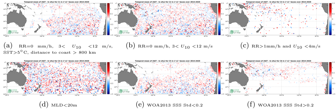
Figure 12: Temporal mean gridded over spatial boxes of size 1^\circ \times 1^\circ of \Delta SSS (SMAP-L2-RSS-V4 - Argo) for 6 different subdatasets corresponding to: RR=0 mm/h, 3 < U_{10} < 12 m/s, SST > 5^\circ C , distance to coast > 800 km (a), RR=0 mm/h, 3 < U_{10} < 12 m/s (b), RR > 1 mm/h and U_{10} < 4 m/s (c), MLD < 20 m (d), WOA2013 SSS Std < 0.2 (e), WOA2013 SSS Std > 0.2 (f).
