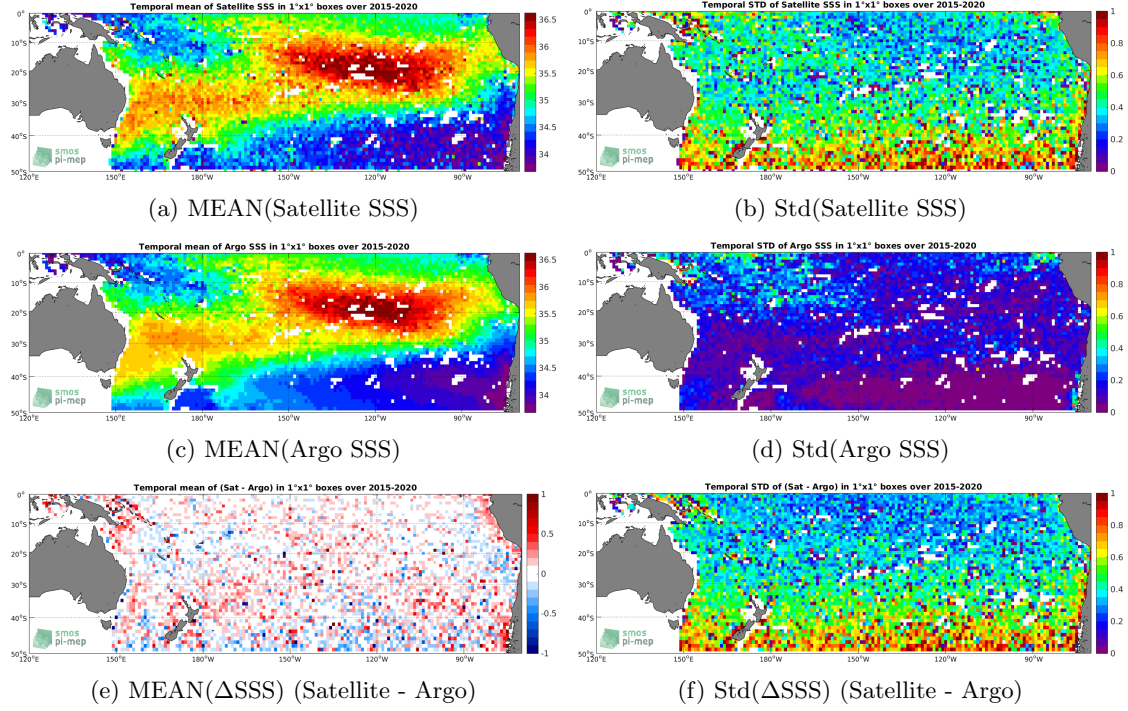
Figure 6: Temporal mean (left) and Std (right) of SSS from SMAP-L2-RSS-V4 (top), Argo (middle), and of \Delta SSS (Satellite - Argo). Only match-up pairs are used to generate these maps.
