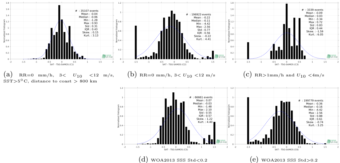
Figure 13: Normalized histogram of \Delta SSS (SMAP-L2-RSS-V3-70KM - TSG-SAMOS) for 5 different subdatasets corresponding to: RR=0 mm/h, 3 < U_{10} < 12 m/s, SST >5^\circ C, distance to coast > 800 km (a), RR=0 mm/h, 3 < U_{10} < 12 m/s (b), RR >1 mm/h and U_{10} < 4 m/s (c), WOA2013 SSS Std <0.2 (d), WOA2013 SSS Std >0.2 (e).
