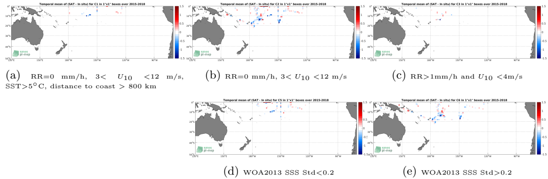
Figure 12: Temporal mean gridded over spatial boxes of size 1^\circ \times 1^\circ of \Delta SSS (SMAP-L2-RSS-V3-70KM - TSG-SAMOS) for 5 different subdatasets corresponding to:RR=0 mm/h, 3 < U_{10} < 12 m/s, SST >5^\circ C, distance to coast > 800 km (a), RR=0 mm/h, 3 < U_{10} < 12 m/s (b), RR >1 mm/h and U_{10} < 4 m/s (c), WOA2013 SSS Std <0.2 (d), WOA2013 SSS Std >0.2 (e).
