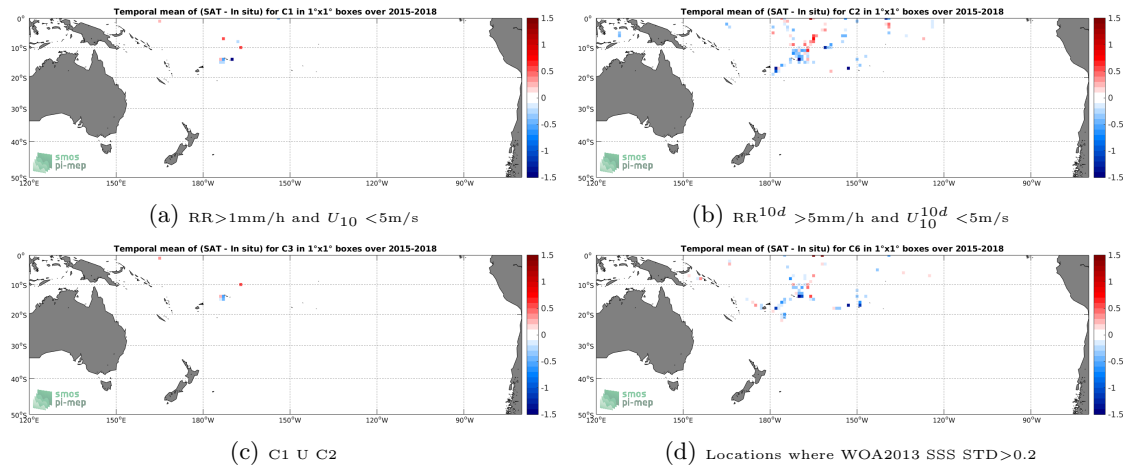
Figure 12: Temporal mean gridded over spatial boxes of size 1^\circ \times 1^\circ of \Delta SSS (SMAP-L2-RSS-V3-70KM - TSG-SAMOS) for 4 different subdatasets corresponding to: RR > 1\text{mm/h} and U_{10} < 5\text{m/s} (a), RR^{10d} > 5\text{mm/h} and U_{10}^{10d} < 5\text{m/s} (b), C1 U C2 (c), Locations where WOA2013 SSS STD > 0.2 (d).
