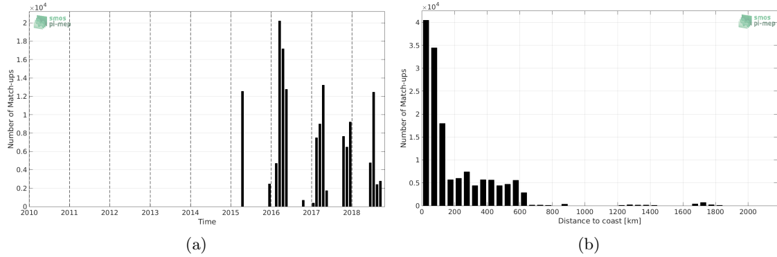
Figure 1: Number of match-ups between TSG-SAMOS and SMAP-L2-RSS-V3-70KM SSS as a function of time (a) and as function of the distance to coast (b) over the South Pacific Ocean Pi-MEP region and for the full satellite product period.
