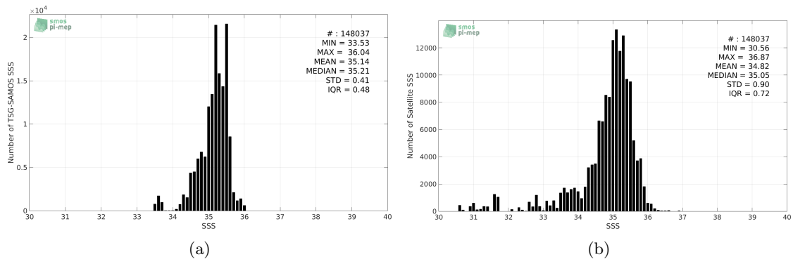
Figure 2: Histograms of SSS from TSG-SAMOS (a) and SMAP-L2-RSS-V3-70KM (b) considering all match-up pairs per bins of 0.1 over the South Pacific Ocean Pi-MEP region and for the full satellite product period.
