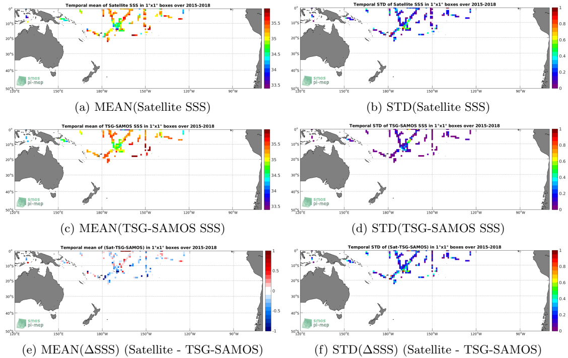
Figure 6: Temporal mean (left) and STD (right) of SSS from SMAP-L2-RSS-V3-70KM (top), TSG-SAMOS (middle), and of \Delta SSS (Satellite - TSG-SAMOS). Only match-up pairs are used to generate these maps.
