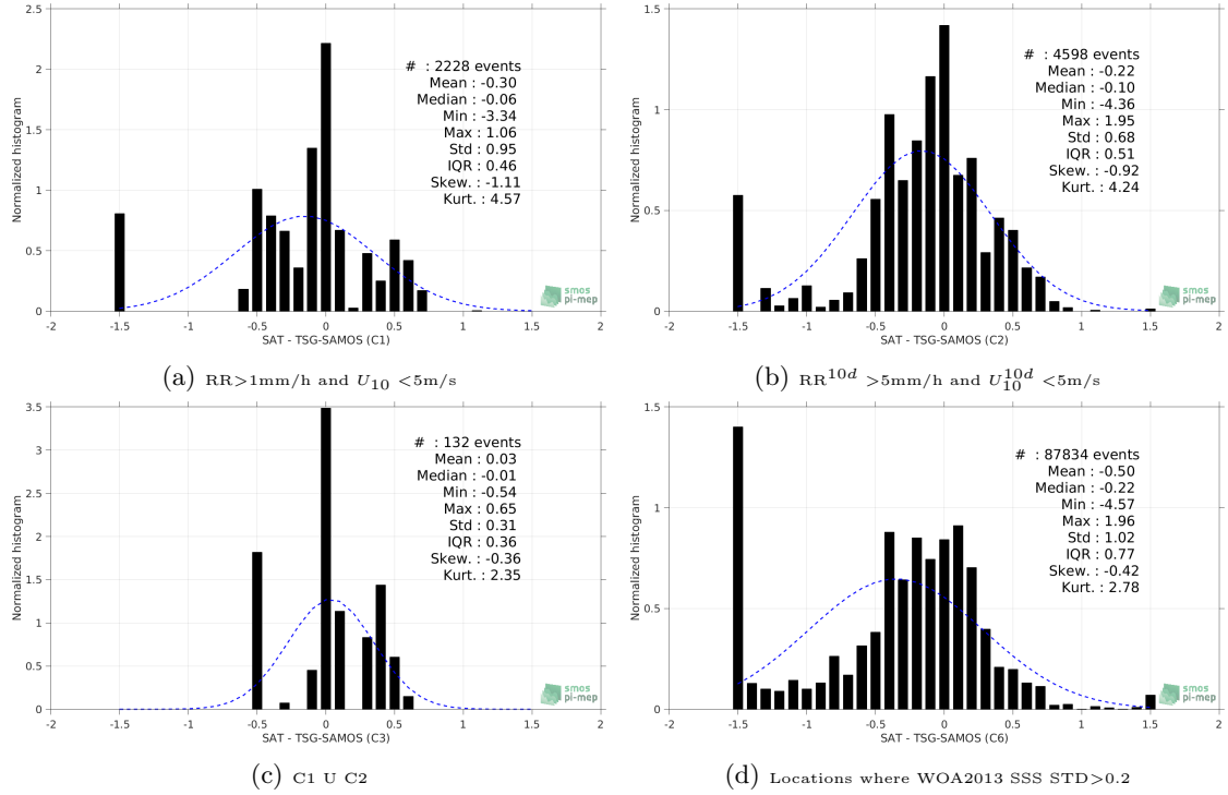
Figure 13: Normalized histogram of \Delta SSS (SMAP-L2-RSS-V3-70KM - TSG-SAMOS) for 6 different subdatasets corresponding to: RR > 1mm/h and U_{10} < 5 m/s (a), RR^{10d} > 5 mm/h and U_{10}^{10d} < 5 m/s (b), C1 U C2 (c), Locations where WOA2013 SSS STD > 0.2 (d).
