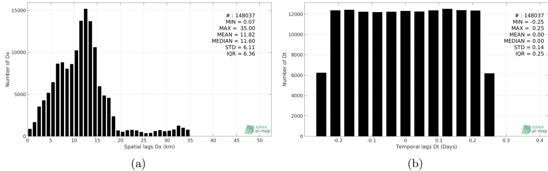
Figure 5: Histograms of the spatial (a) and temporal (b) lags between the time of the TSG-SAMOS measurements and the date of the corresponding SMAP-L2-RSS-V3-70KM SSS product.
