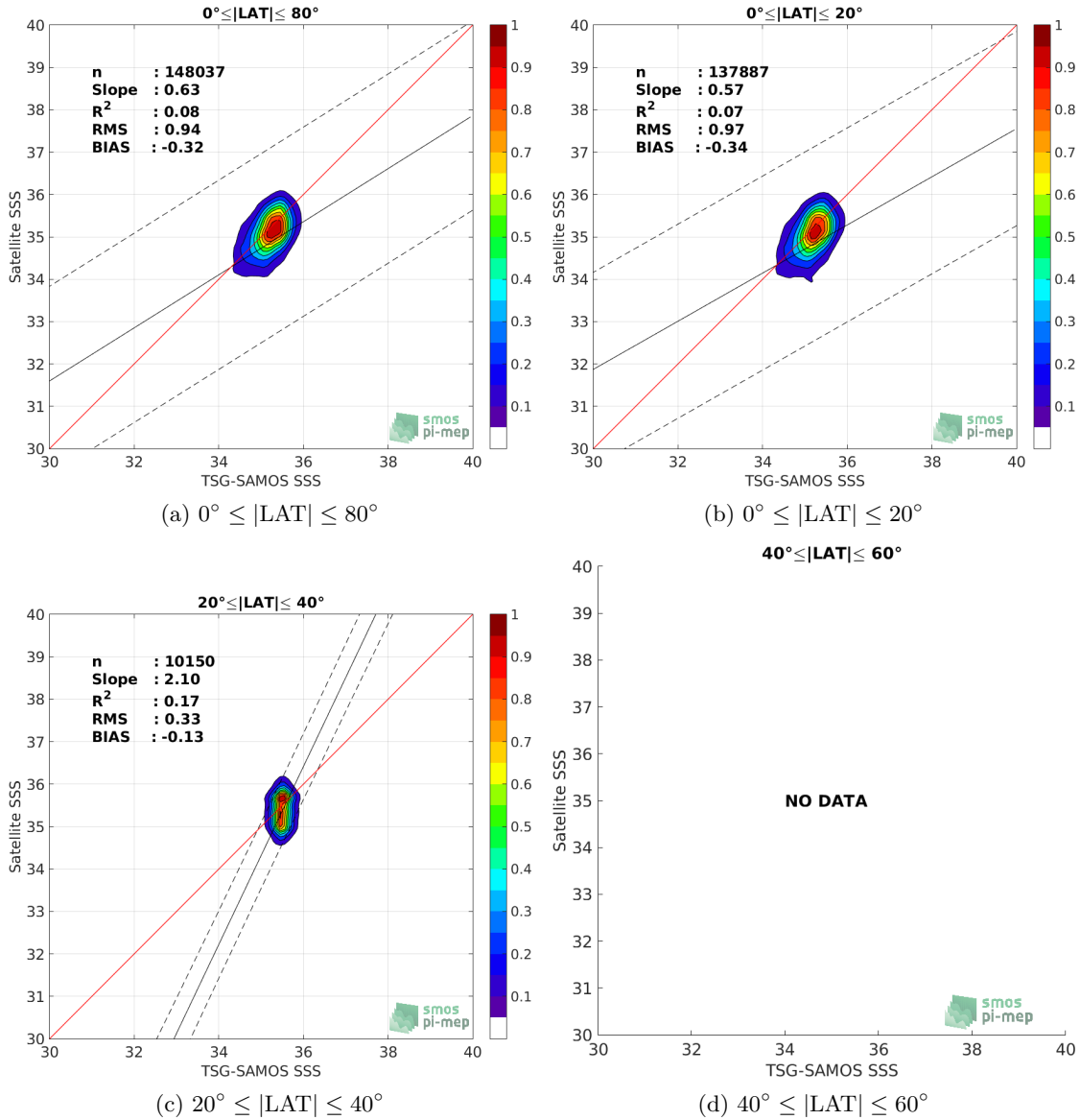
Figure 9: Contour maps of the concentration of SMAP-L2-RSS-V3-70KM SSS (y-axis) versus TSG-SAMOS SSS (x-axis) at match-up pairs for different latitude bands. For each plot, the red line shows x=y . The black thin and dashed lines indicate a linear fit through the data cloud and the \pm 95\% confidence levels, respectively. The number match-up pairs n , the slope and R^2 coefficient of the linear fit, the root mean square (RMS) and the mean bias between satellite and in situ data are indicated for each latitude band in each plots.
