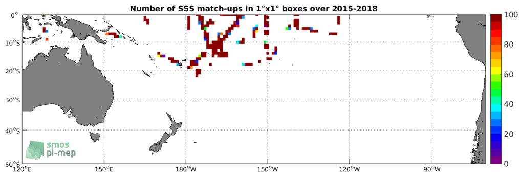
Figure 4: Number of SSS match-ups between TSG-SAMOS SSS and the SMAP-L2-RSS-V3-70KM SSS product for the South Pacific Ocean Pi-MEP region over 1^\circ \times 1^\circ boxes and for the full satellite product period.
