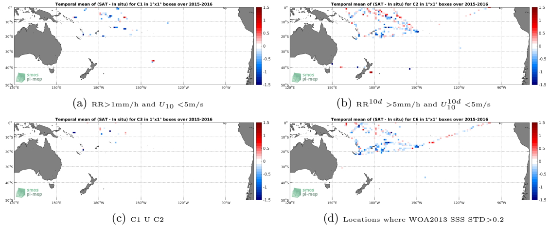
Figure 12: Temporal mean gridded over spatial boxes of size 1^\circ \times 1^\circ of \Delta SSS (SMAP-L2-RSS-V3-70KM - TSG-LEGOS-DM) for 4 different subdatasets corresponding to: RR > 1mm/h and U_{10} < 5\text{m/s} (a), RR^{10d} > 5\text{mm/h} and U_{10}^{10d} < 5\text{m/s} (b), C1 U C2 (c), Locations where WOA2013 SSS STD > 0.2 (d).
