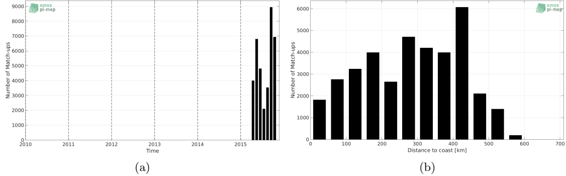
Figure 1: Number of match-ups between TSG-GOSUD-Research-vessel and SMAP-L2-RSS-V3-70KM SSS as a function of time (a) and as function of the distance to coast (b) over the South Pacific Ocean Pi-MEP region and for the full satellite product period.
