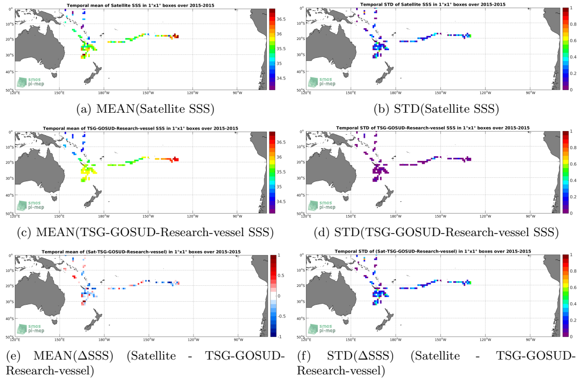
Figure 6: Temporal mean (left) and STD (right) of SSS from SMAP-L2-RSS-V3-70KM (top), TSG-GOSUD-Research-vessel (middle), and of \Delta SSS (Satellite - TSG-GOSUD-Research-vessel). Only match-up pairs are used to generate these maps.
