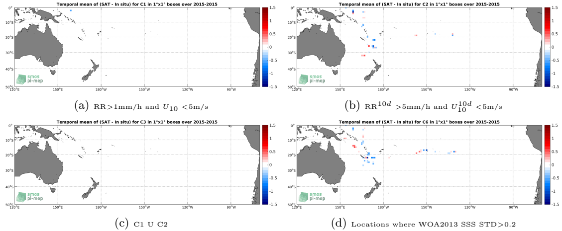
Figure 12: Temporal mean gridded over spatial boxes of size 1^\circ \times 1^\circ of \Delta SSS (SMAP-L2-RSS-V3-70KM - TSG-GOSUD-Research-vessel) for 4 different subdatasets corresponding to: RR > 1\text{mm/h} and U_{10} < 5\text{m/s} (a), RR^{10d} > 5\text{mm/h} and U_{10}^{10d} < 5\text{m/s} (b), C1 U C2 (c), Locations where WOA2013 SSS STD > 0.2 (d).
