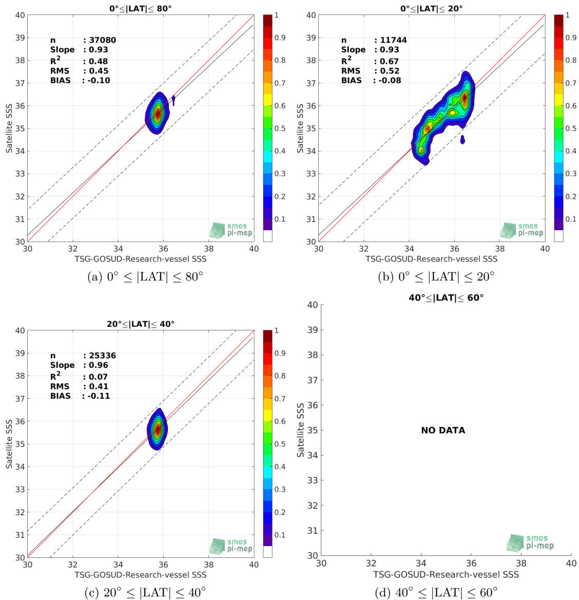
Figure 9: Contour maps of the concentration of SMAP-L2-RSS-V3-70KM SSS (y-axis) versus TSG-GOSUD-Research-vessel SSS (x-axis) at match-up pairs for different latitude bands. For each plot, the red line shows x=y . The black thin and dashed lines indicate a linear fit through the data cloud and the \pm 95\% confidence levels, respectively. The number match-up pairs n , the slope and R^2 coefficient of the linear fit, the root mean square (RMS) and the mean bias between satellite and in situ data are indicated for each latitude band in each plots.
