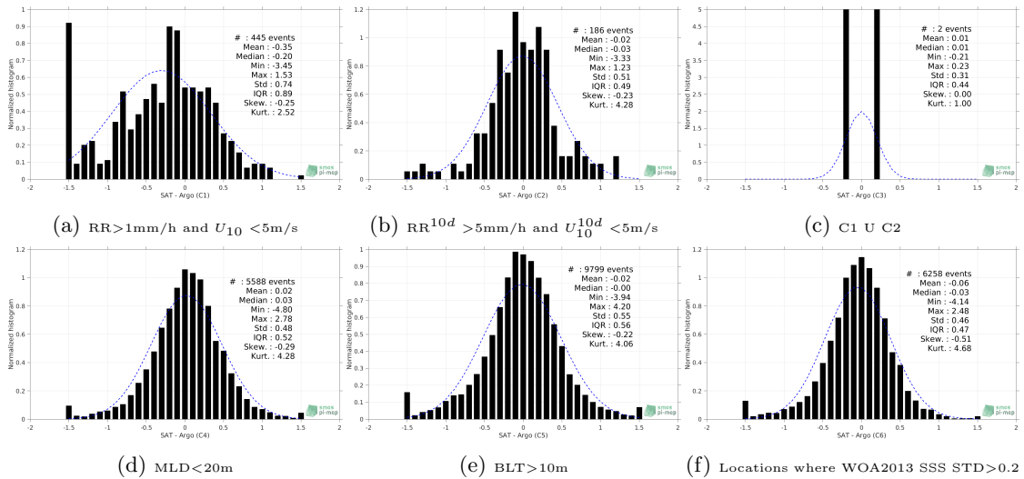
Figure 13: Normalized histogram of \Delta SSS (SMAP-L2-RSS-V3-70KM - Argo) for 6 different subdatasets corresponding to: RR>1mm/h and U_{10} <5m/s (a), RR^{10d} >5mm/h and U_{10}^{10d} <5m/s (b), C1 U C2 (c),MLD<20m (d),BLT>10m (e),Locations where WOA2013 SSS STD>0.2 (f).
