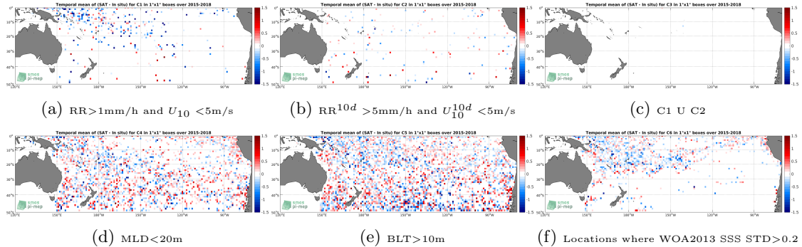
Figure 12: Temporal mean gridded over spatial boxes of size 1°x1° of \Delta SSS (SMAP-L2-RSS-V3-70KM - Argo) for 6 different subdatasets corresponding to:RR>1mm/h and U_{10} <5m/s (a), RR^{10d} >5mm/h and U_{10}^{10d} <5m/s (b), C1 U C2 (c),MLD<20m (d),BLT>10m (e),Locations where WOA2013 SSS STD>0.2 (f).
