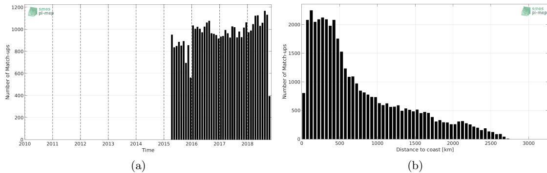
Figure 1: Number of match-ups between Argo and SMAP-L2-RSS-V3-70KM SSS as a function of time (a) and as function of the distance to coast (b) over the South Pacific Ocean Pi-MEP region and for the full satellite product period.
