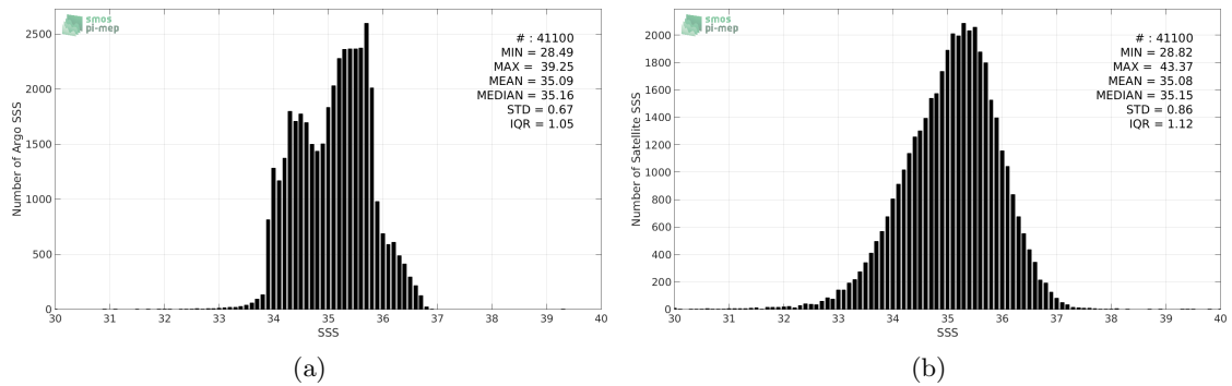
Figure 2: Histograms of SSS from Argo (a) and SMAP-L2-RSS-V3-70KM (b) considering all match-up pairs per bins of 0.1 over the South Pacific Ocean Pi-MEP region and for the full satellite product period.
