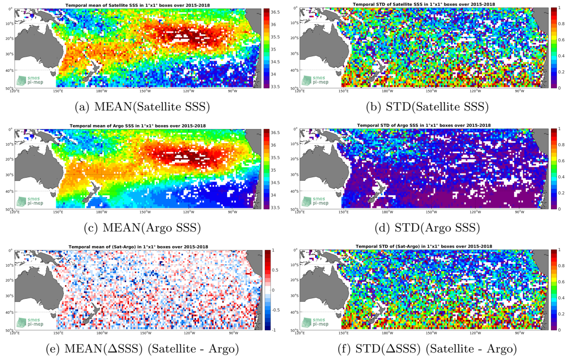
Figure 6: Temporal mean (left) and STD (right) of SSS from SMAP-L2-RSS-V3-70KM (top), Argo (middle), and of \Delta SSS (Satellite - Argo). Only match-up pairs are used to generate these maps.
